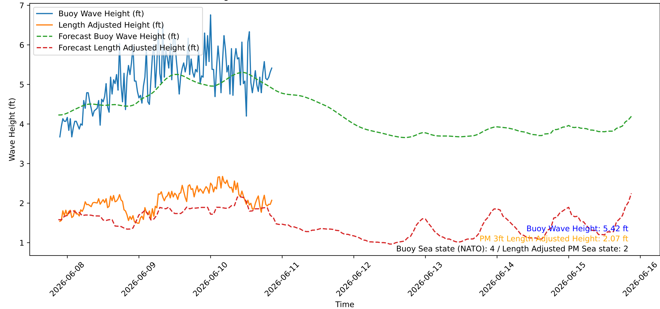
Wave Heights over Time for Oceanside Harbor at 2026-06-10 21:20:27
