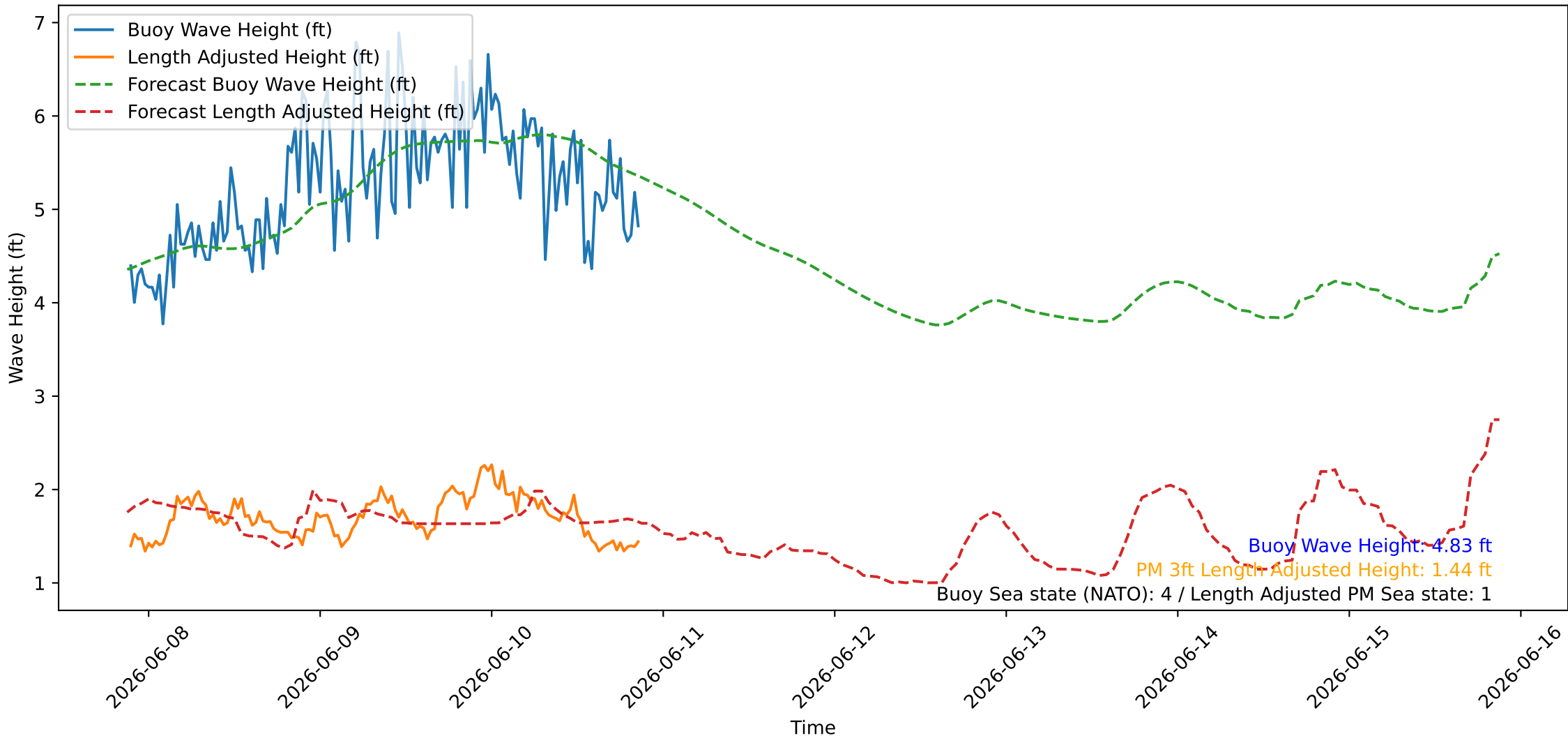
Wave Heights over Time for Green Beach at 2026-06-10 21:21:11
