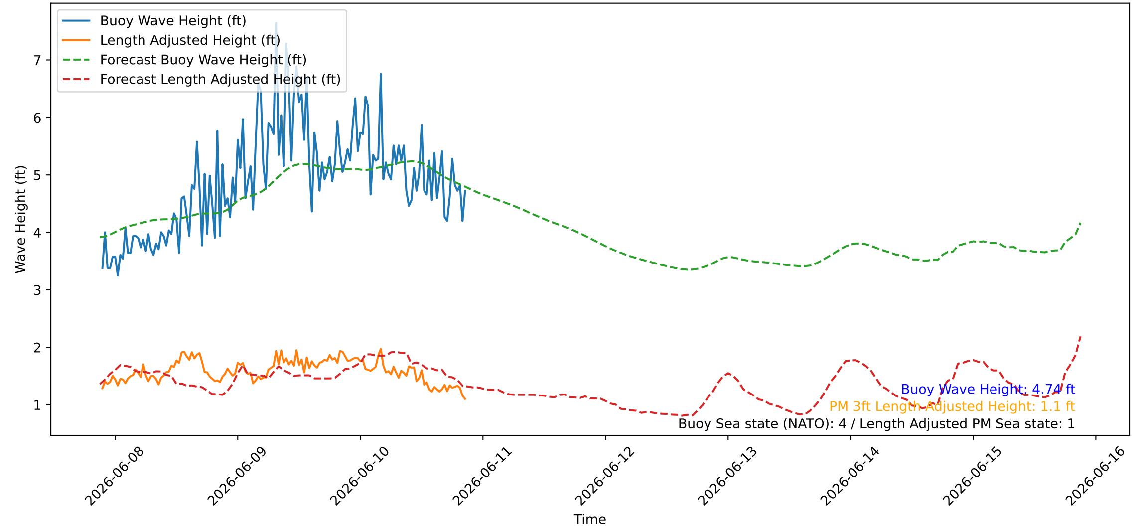
Wave Heights over Time for Red Beach at 2026-06-10 21:20:48
