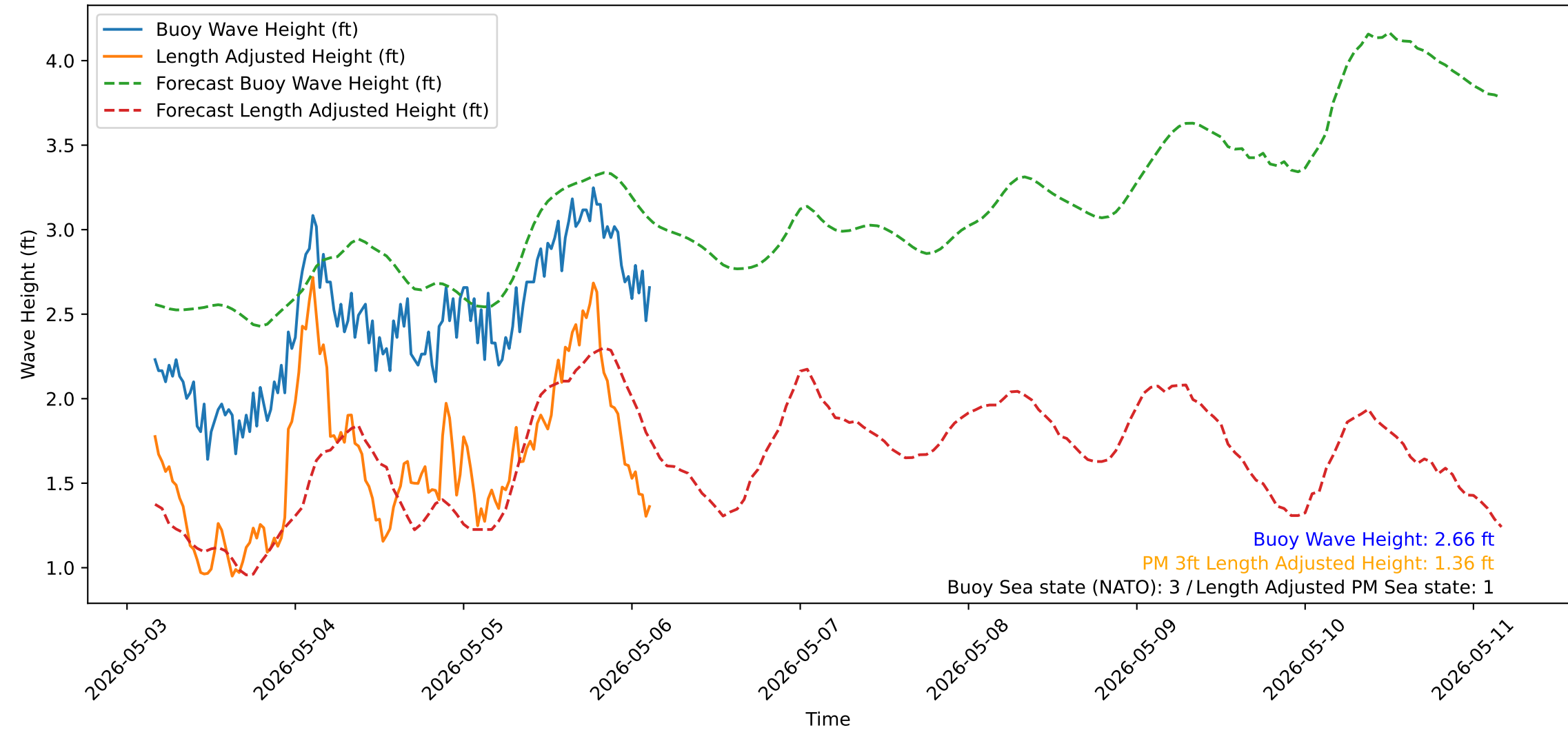
Wave Heights over Time for Oceanside Harbor at 2026-05-06 03:50:31
