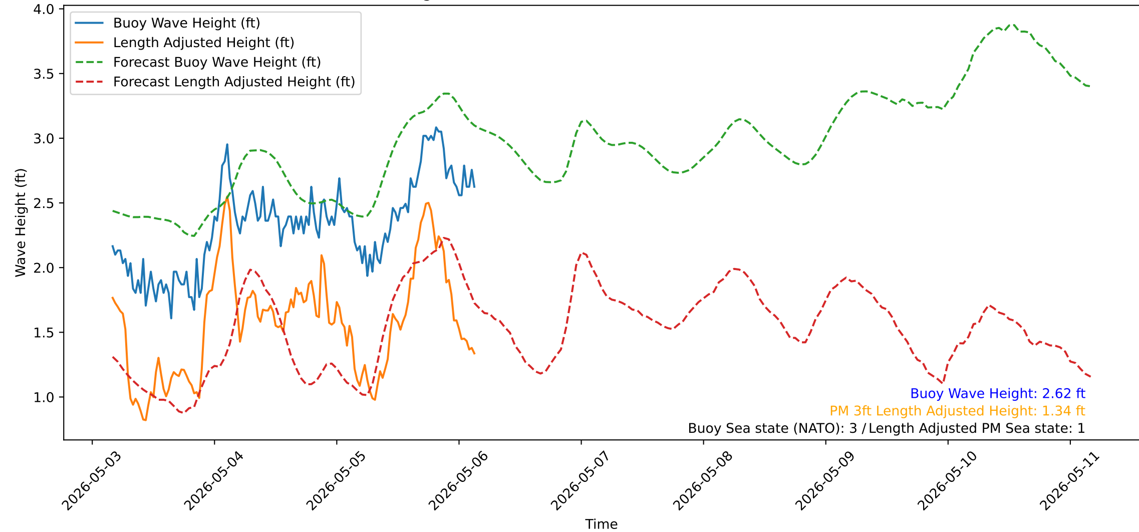
Wave Heights over Time for Red Beach at 2026-05-06 03:50:51
