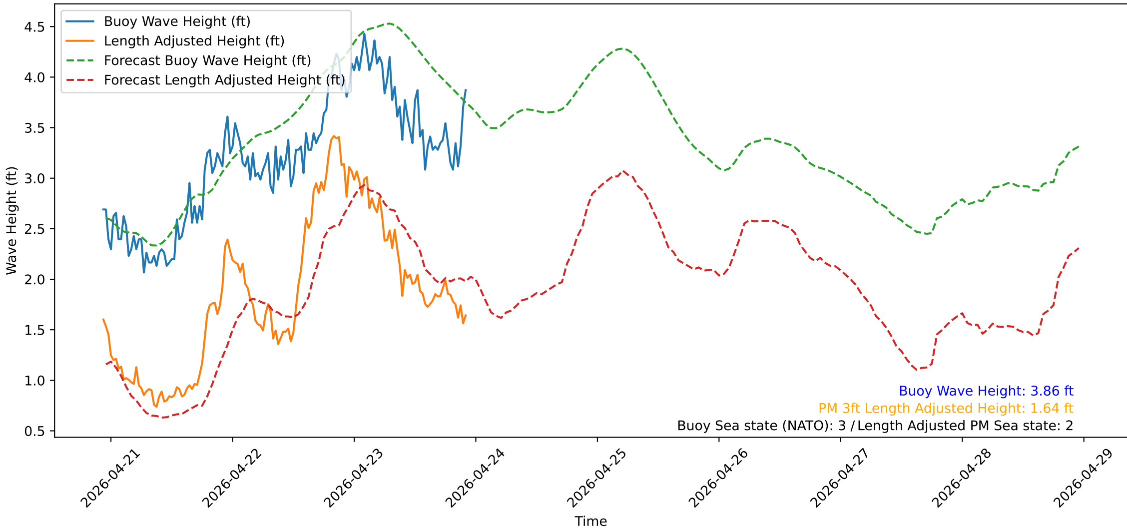
Wave Heights over Time for Oceanside Harbor at 2026-04-23 22:40:31
