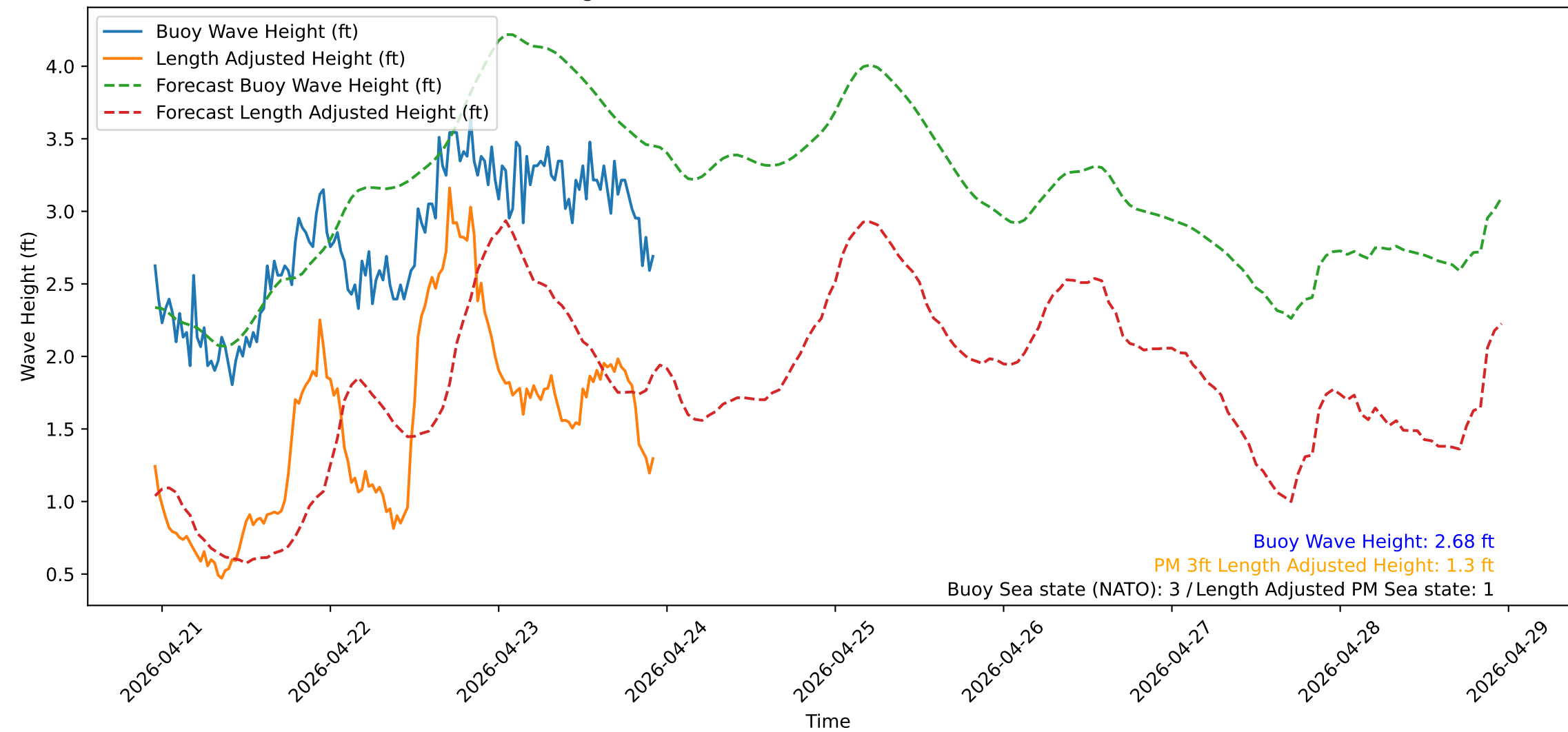
Wave Heights over Time for Red Beach at 2026-04-23 22:40:50
