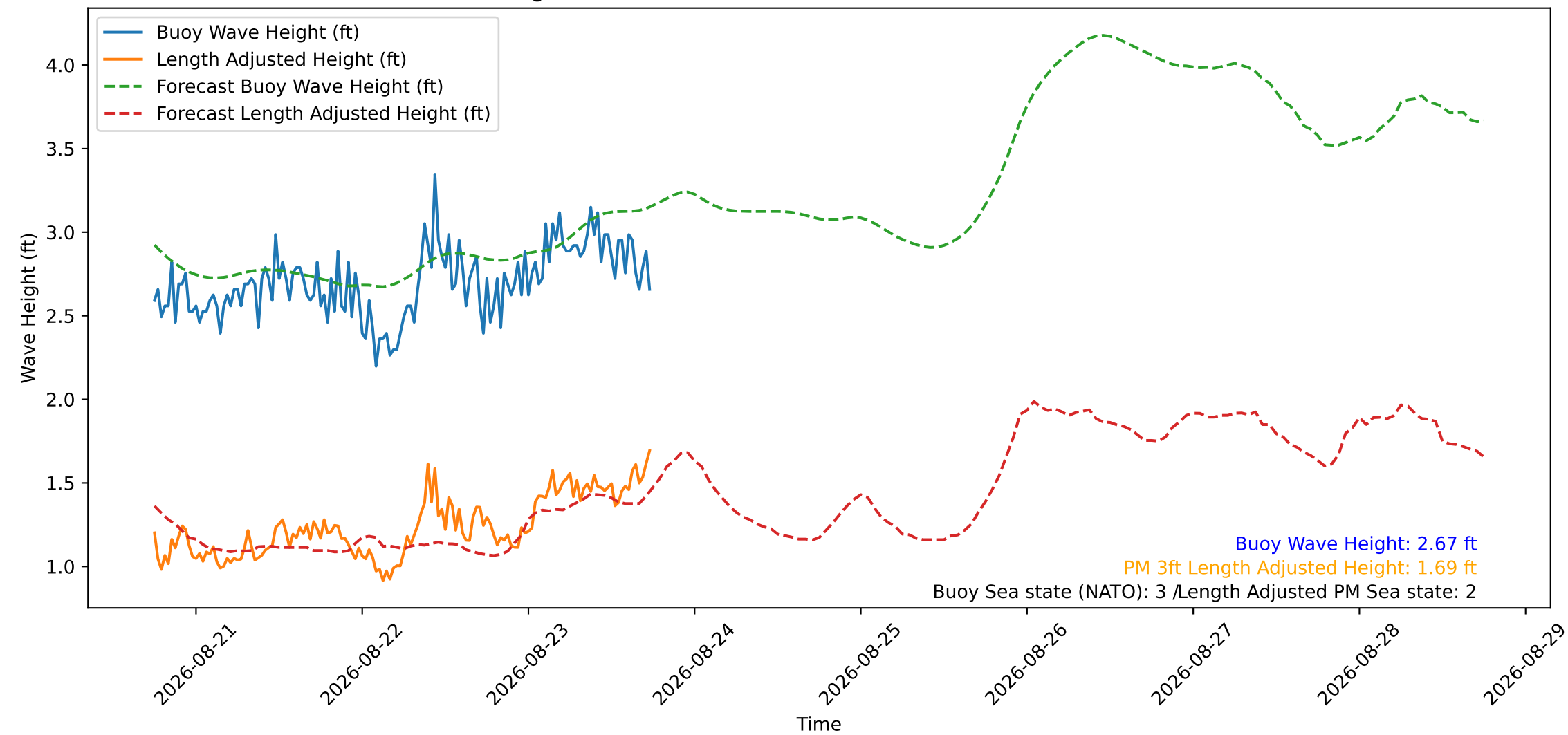
Wave Heights over Time for Oceanside Harbor at 2026-08-23 18:00:30
