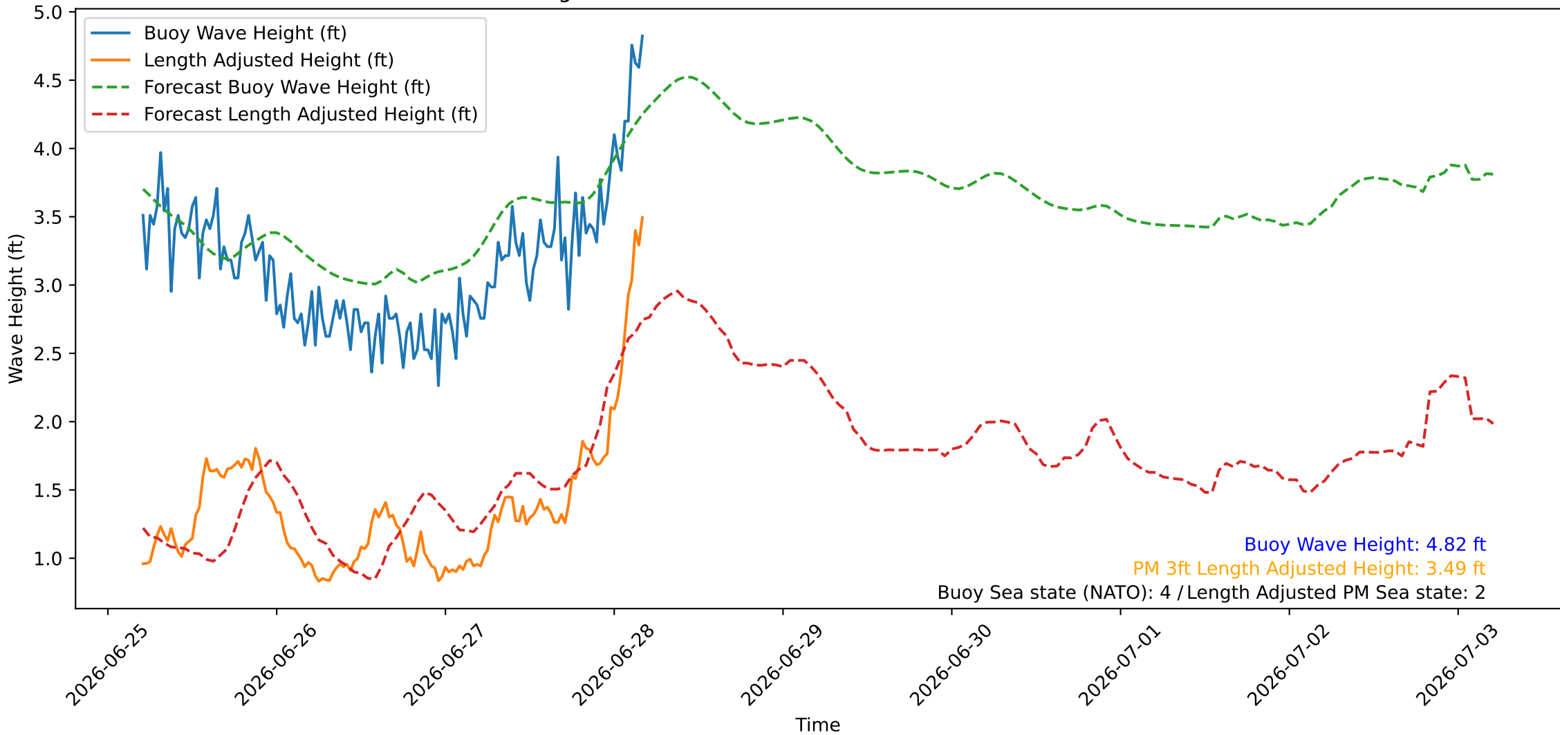
Wave Heights over Time for Green Beach at 2026-06-28 04:51:08
