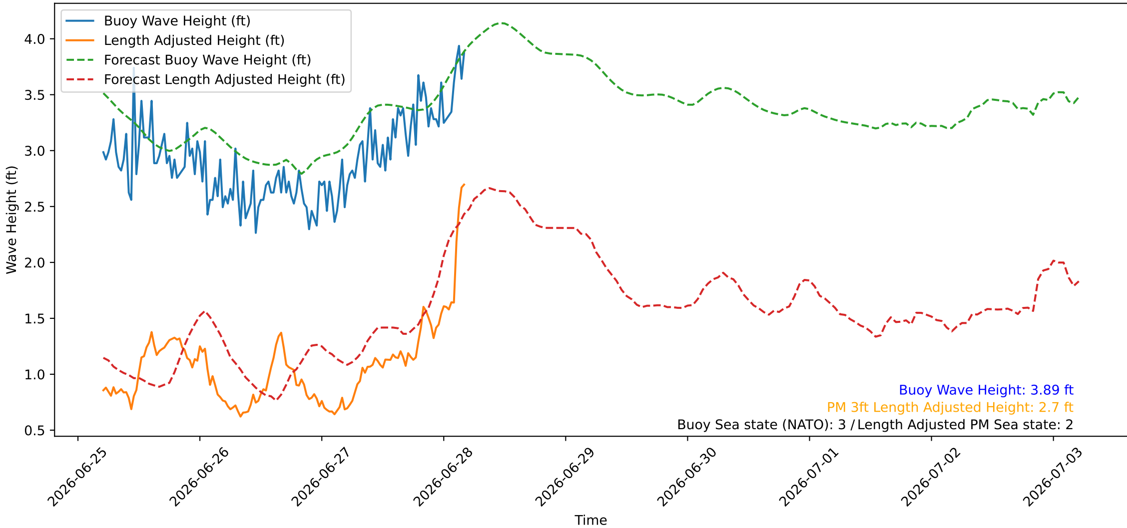
Wave Heights over Time for Red Beach at 2026-06-28 04:50:46
