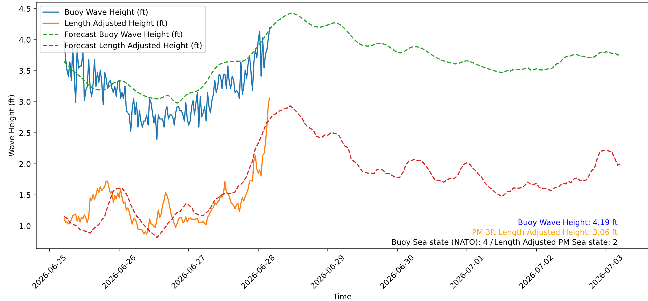
Wave Heights over Time for Oceanside Harbor at 2026-06-28 04:50:26
