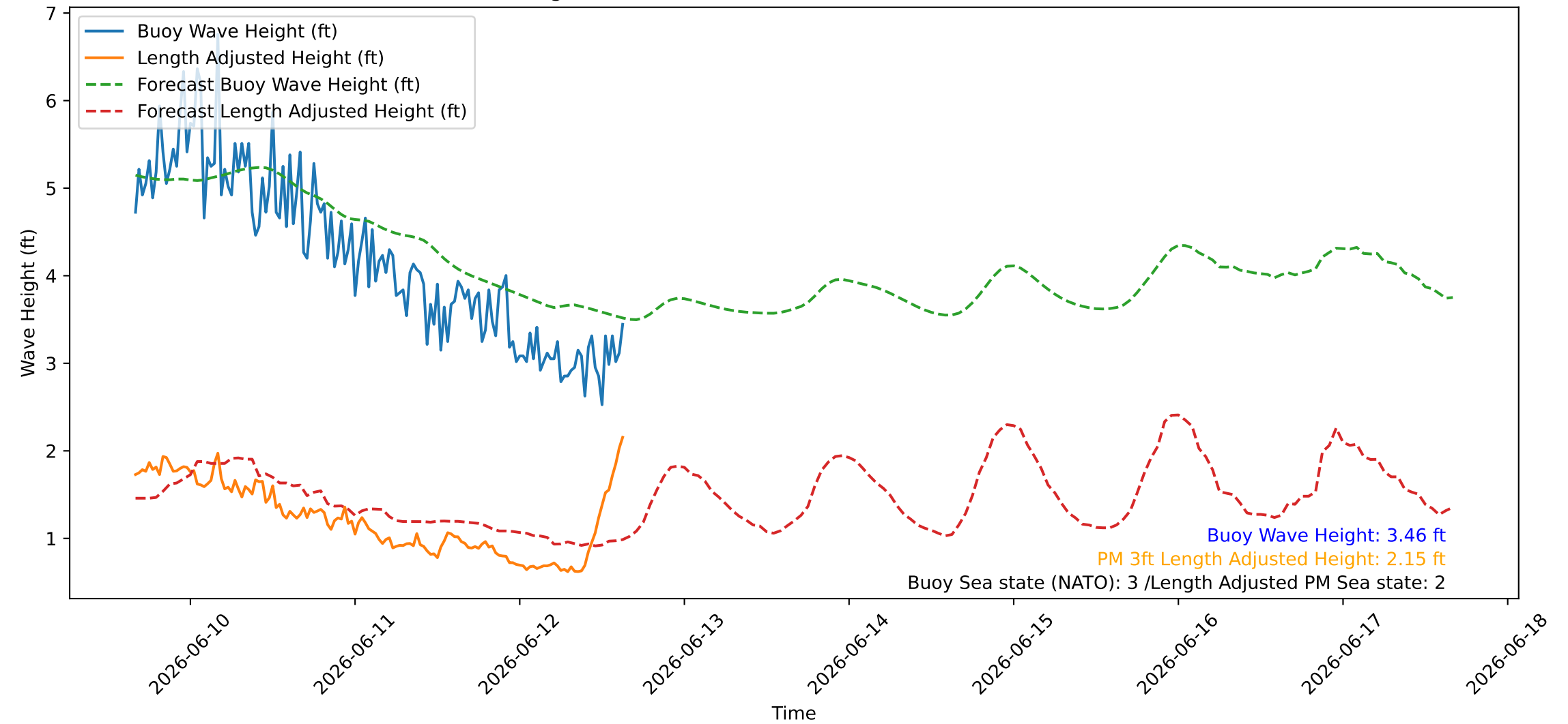
Wave Heights over Time for Red Beach at 2026-06-12 15:40:45
