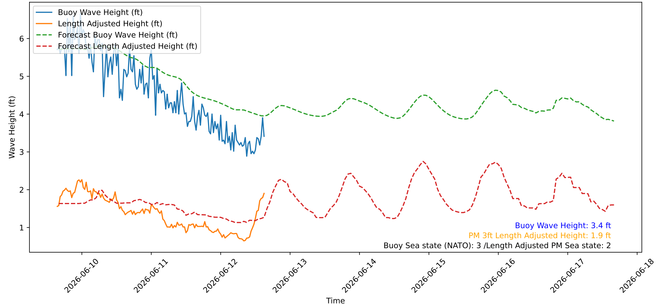
Wave Heights over Time for Green Beach at 2026-06-12 15:41:09
