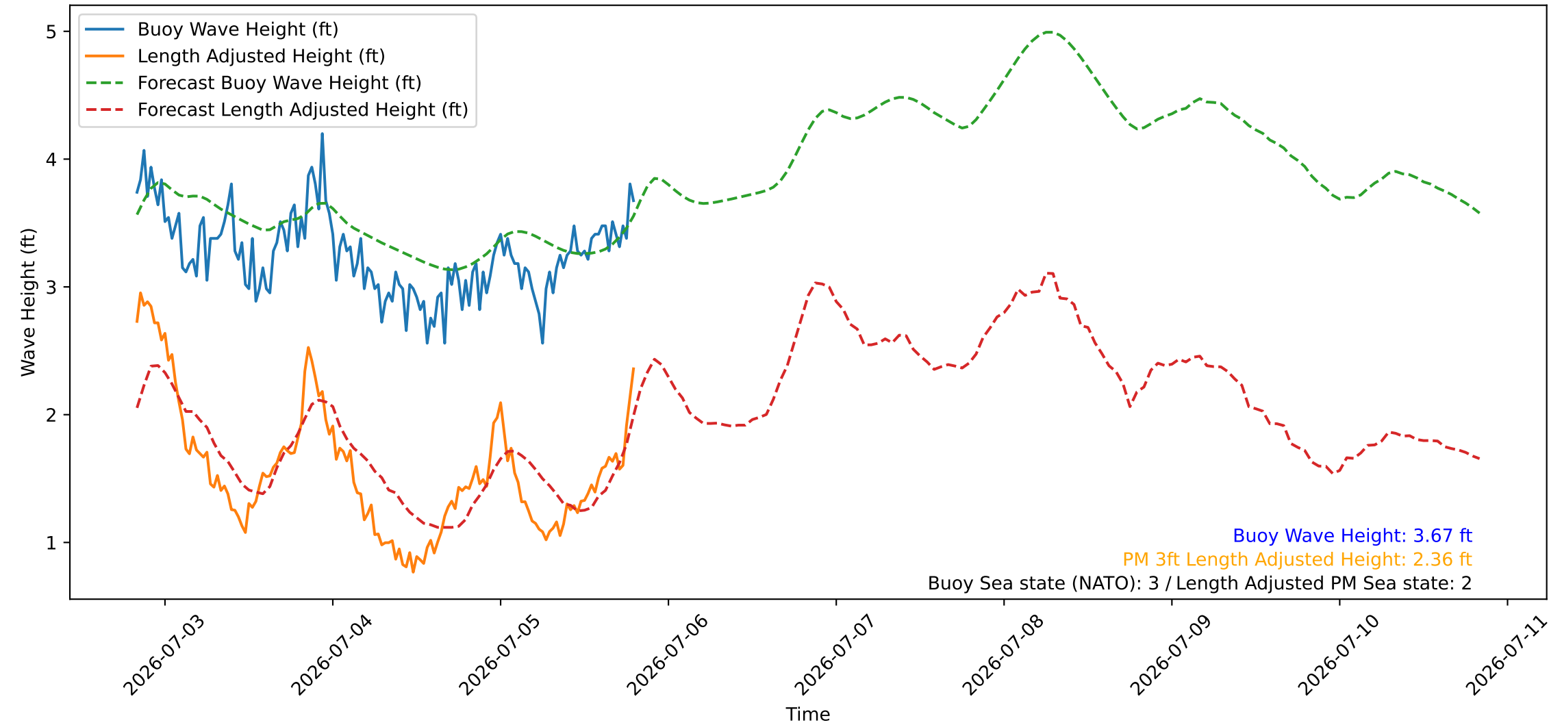
Wave Heights over Time for Green Beach at 2026-07-05 20:01:09
