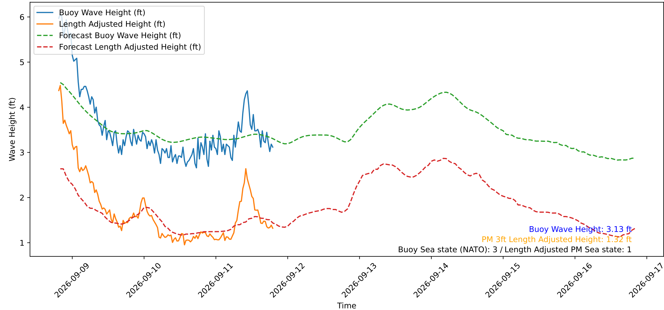
Wave Heights over Time for Oceanside Harbor at 2026-09-11 19:40:32
