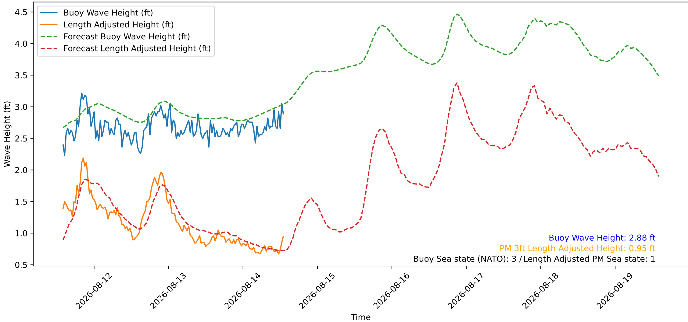
Wave Heights over Time for Green Beach at 2026-08-14 14:01:08
