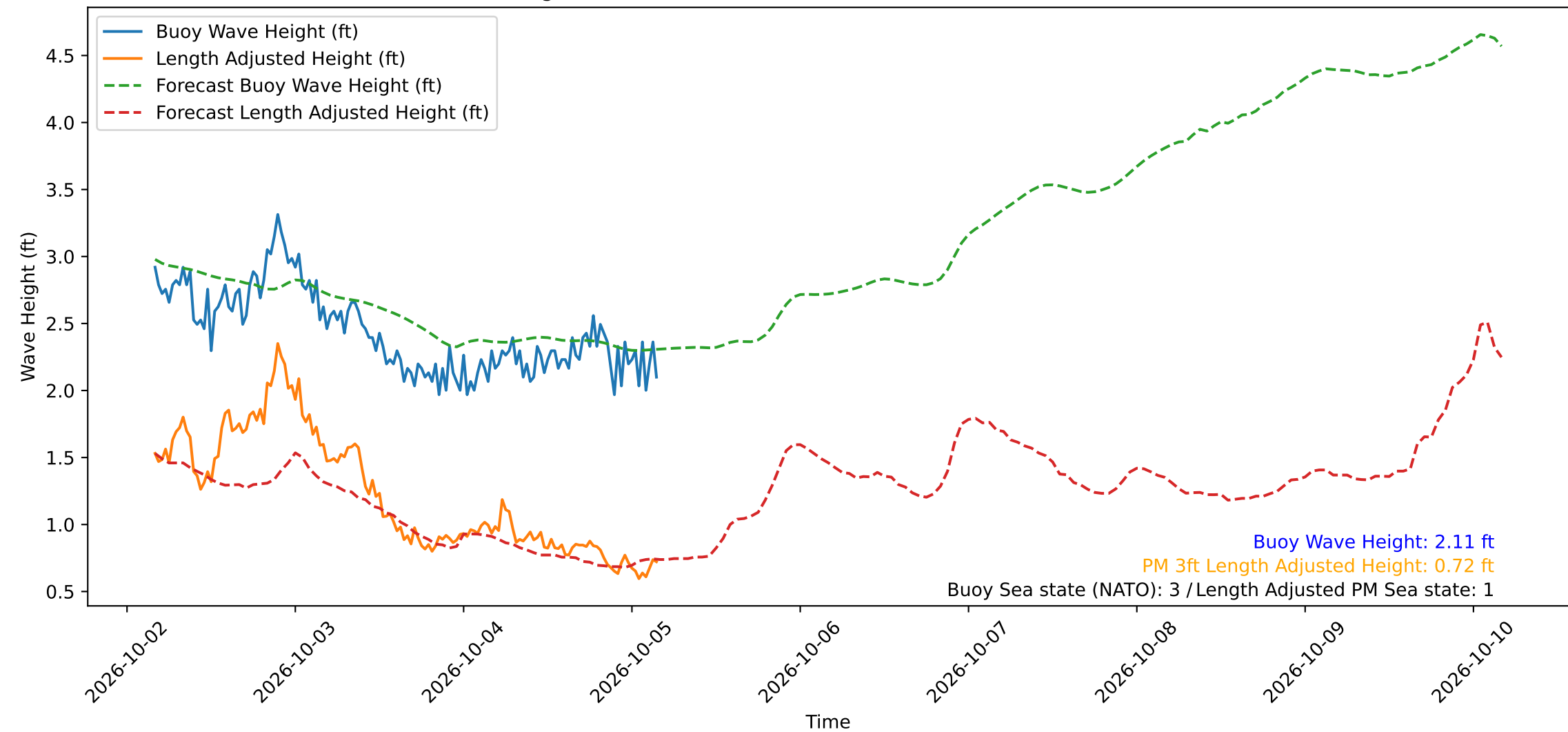
Wave Heights over Time for Oceanside Harbor at 2026-10-05 04:10:30
