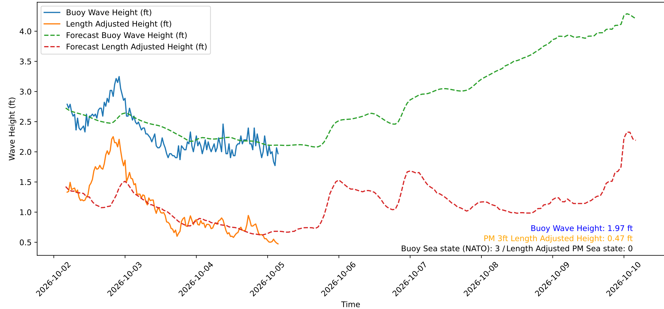
Wave Heights over Time for Red Beach at 2026-10-05 04:10:49
