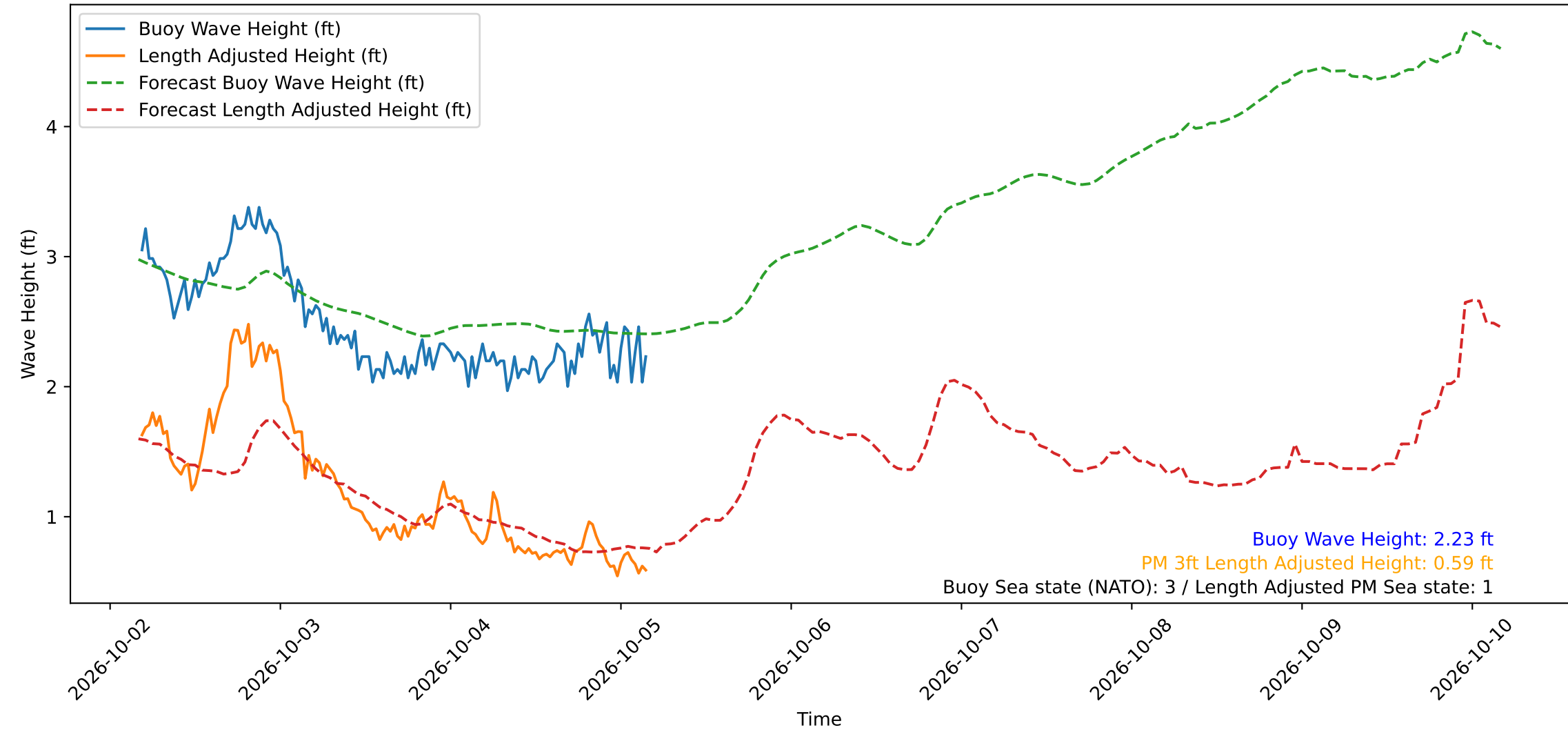
Wave Heights over Time for Green Beach at 2026-10-05 04:11:12
