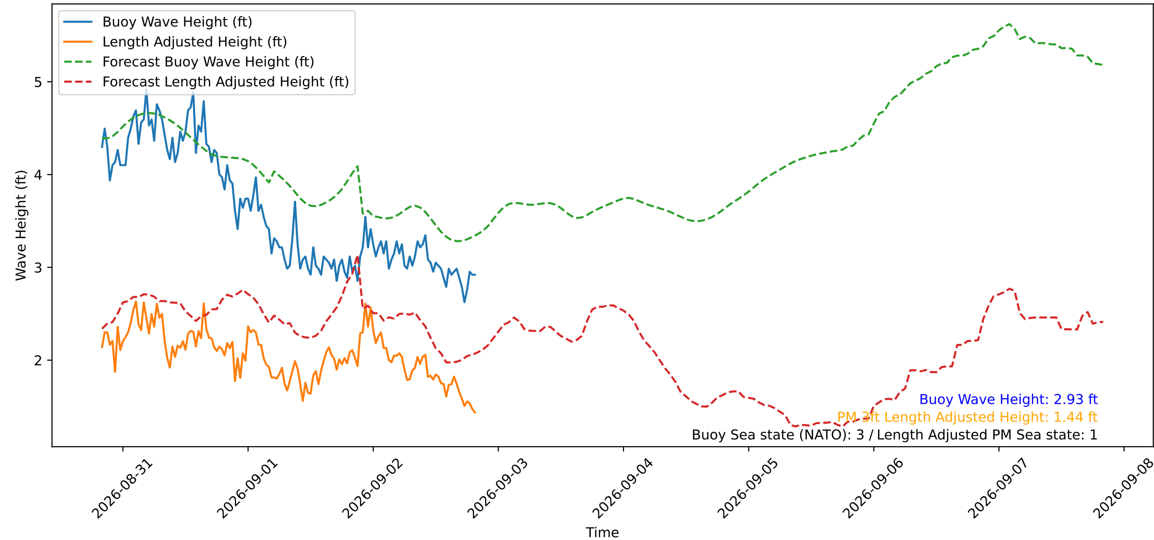
Wave Heights over Time for Oceanside Harbor at 2026-09-02 20:10:30
