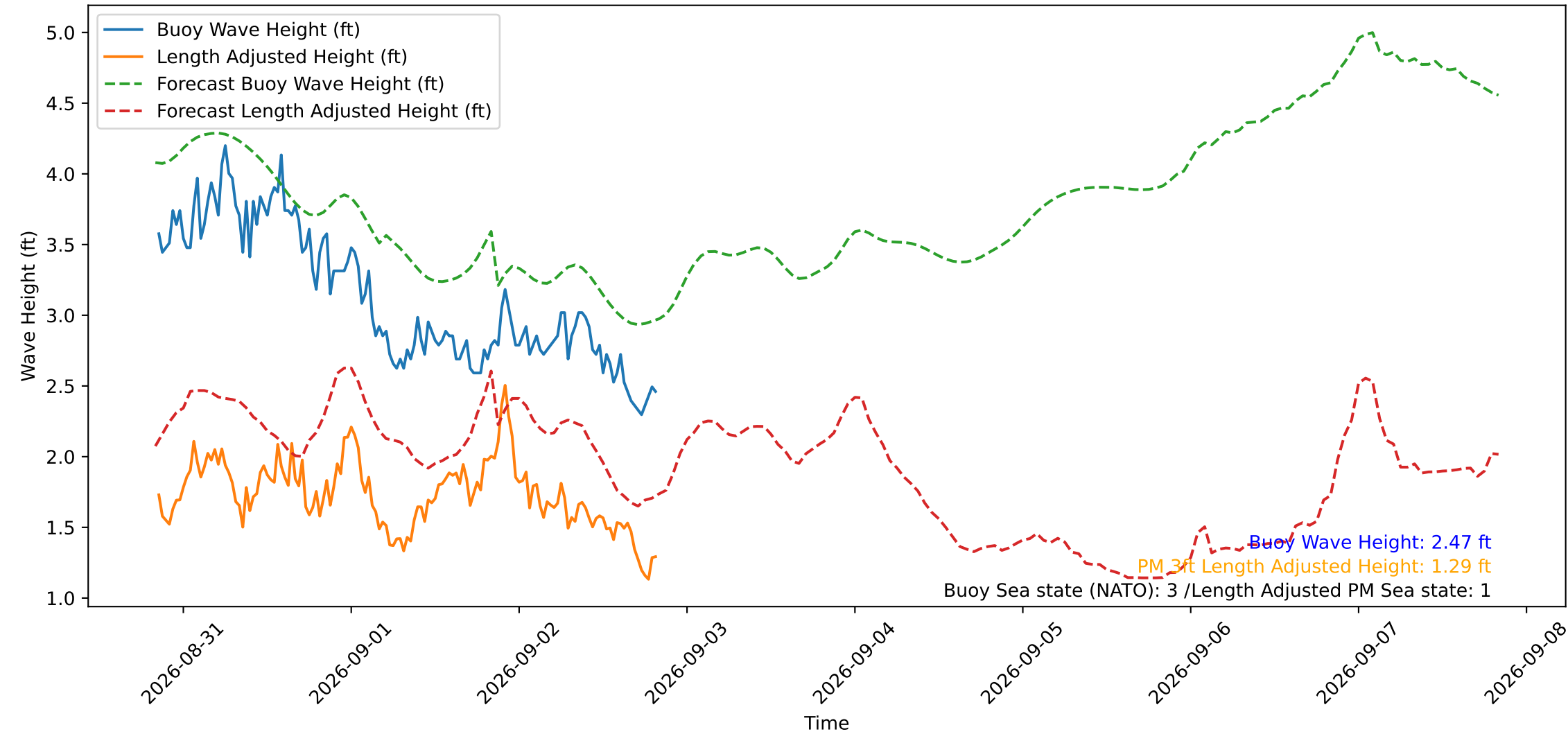
Wave Heights over Time for Red Beach at 2026-09-02 20:10:49
