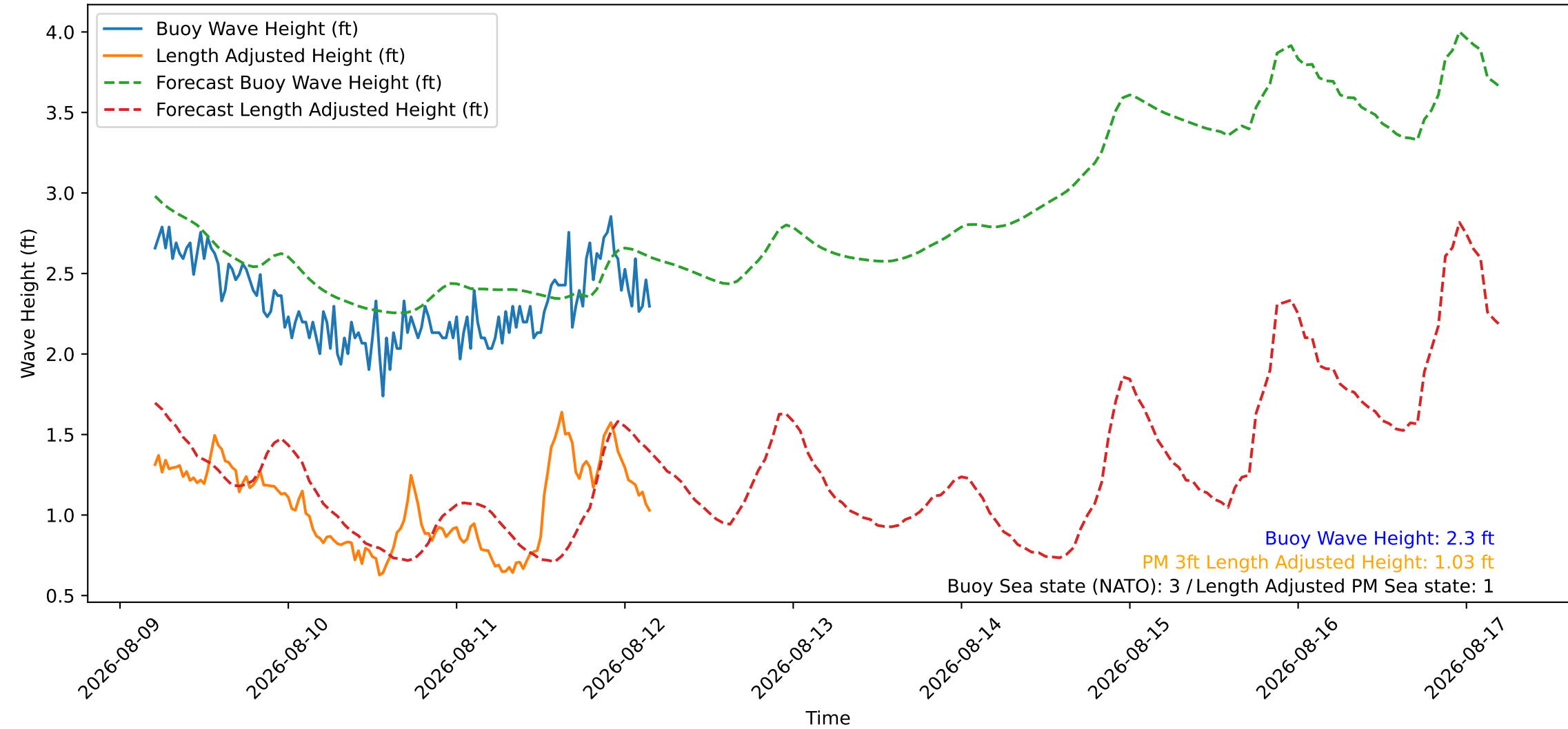
Wave Heights over Time for Red Beach at 2026-08-12 04:30:46
