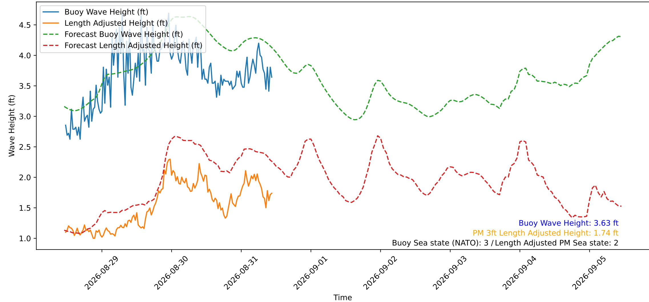
Wave Heights over Time for Red Beach at 2026-08-31 11:20:50
