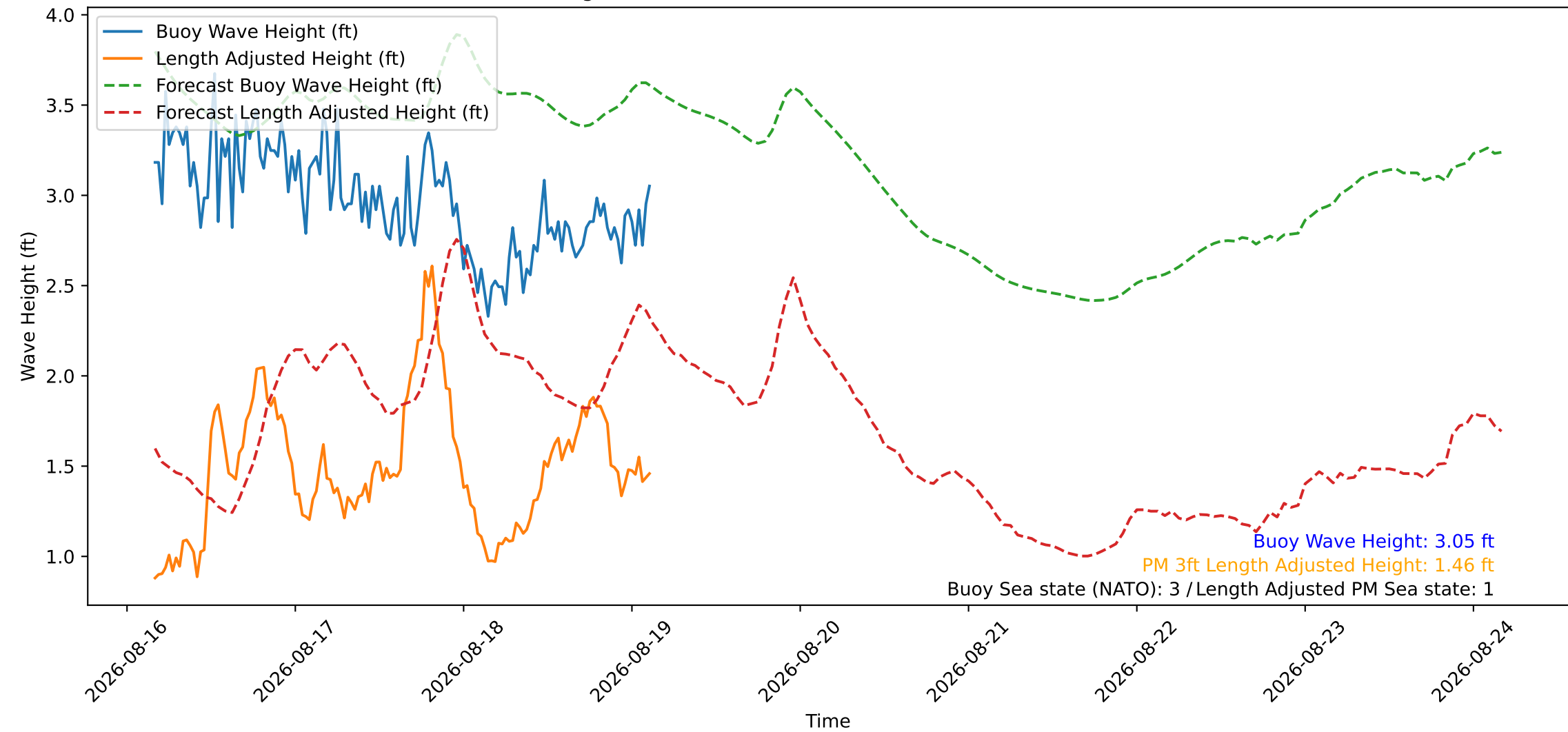
Wave Heights over Time for Red Beach at 2026-08-19 03:30:46
