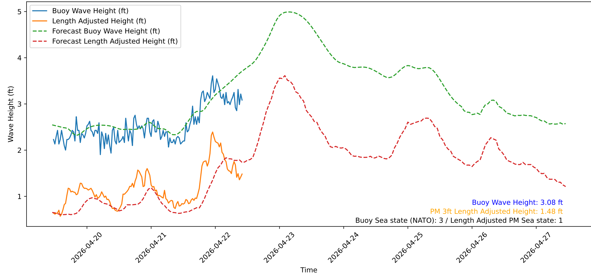
Wave Heights over Time for Oceanside Harbor at 2026-04-22 11:20:31
