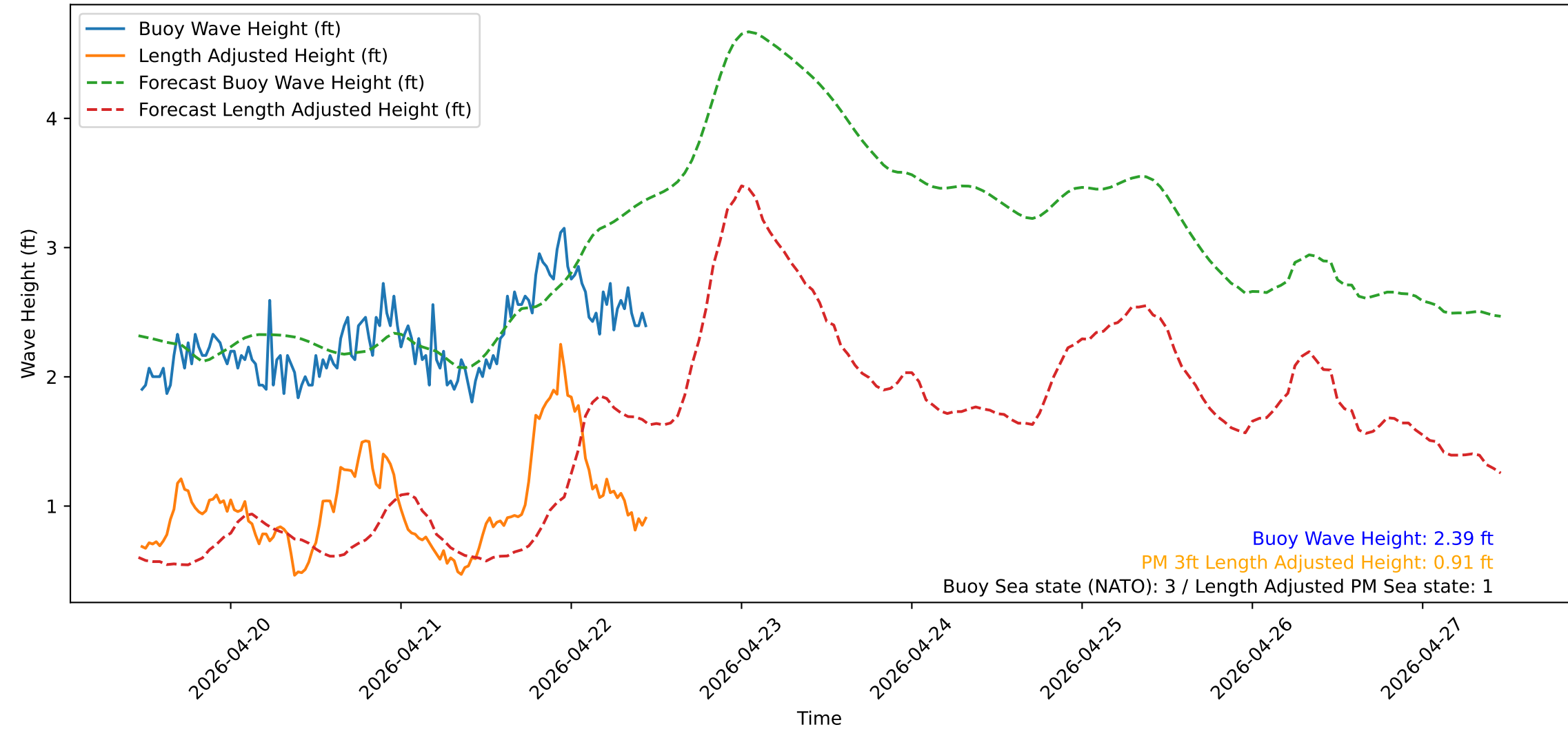
Wave Heights over Time for Red Beach at 2026-04-22 11:20:51
