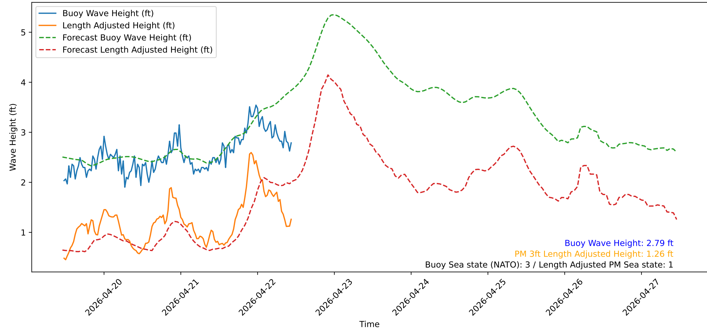
Wave Heights over Time for Green Beach at 2026-04-22 11:21:13
