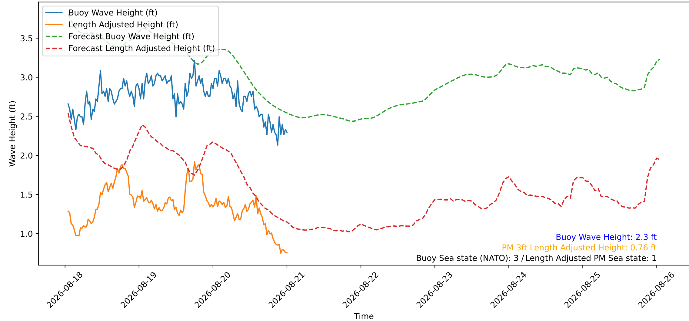
Wave Heights over Time for Red Beach at 2026-08-21 00:40:47
