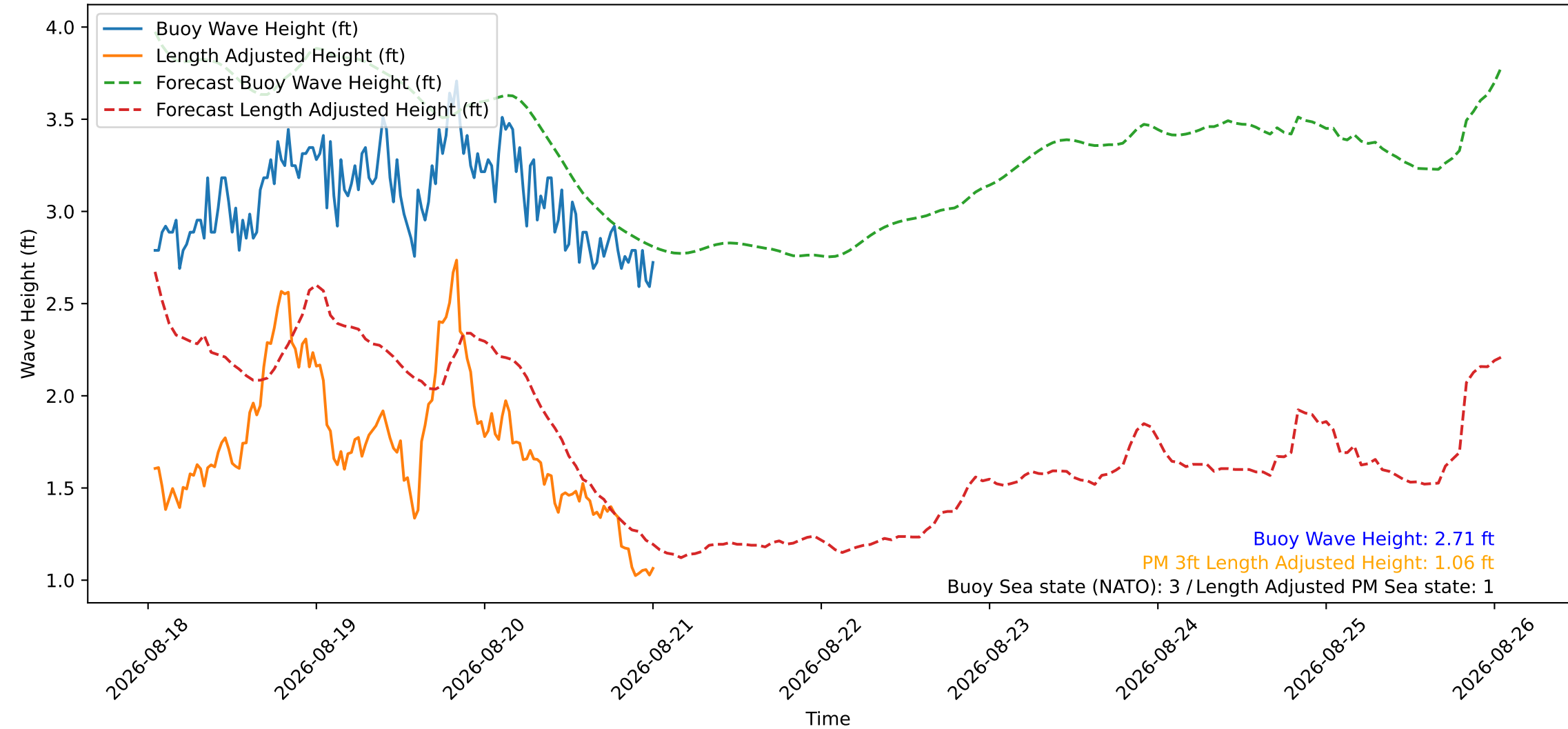
Wave Heights over Time for Green Beach at 2026-08-21 00:41:09
