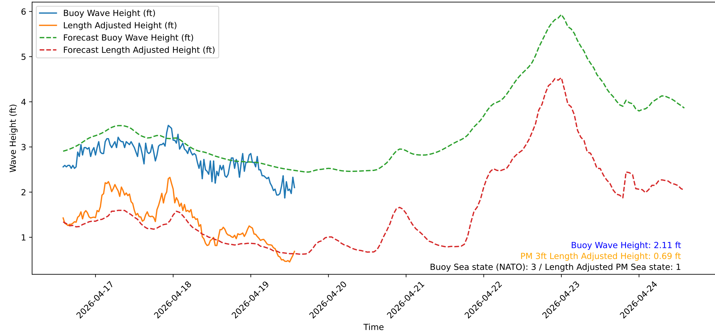
Wave Heights over Time for Green Beach at 2026-04-19 14:11:13
