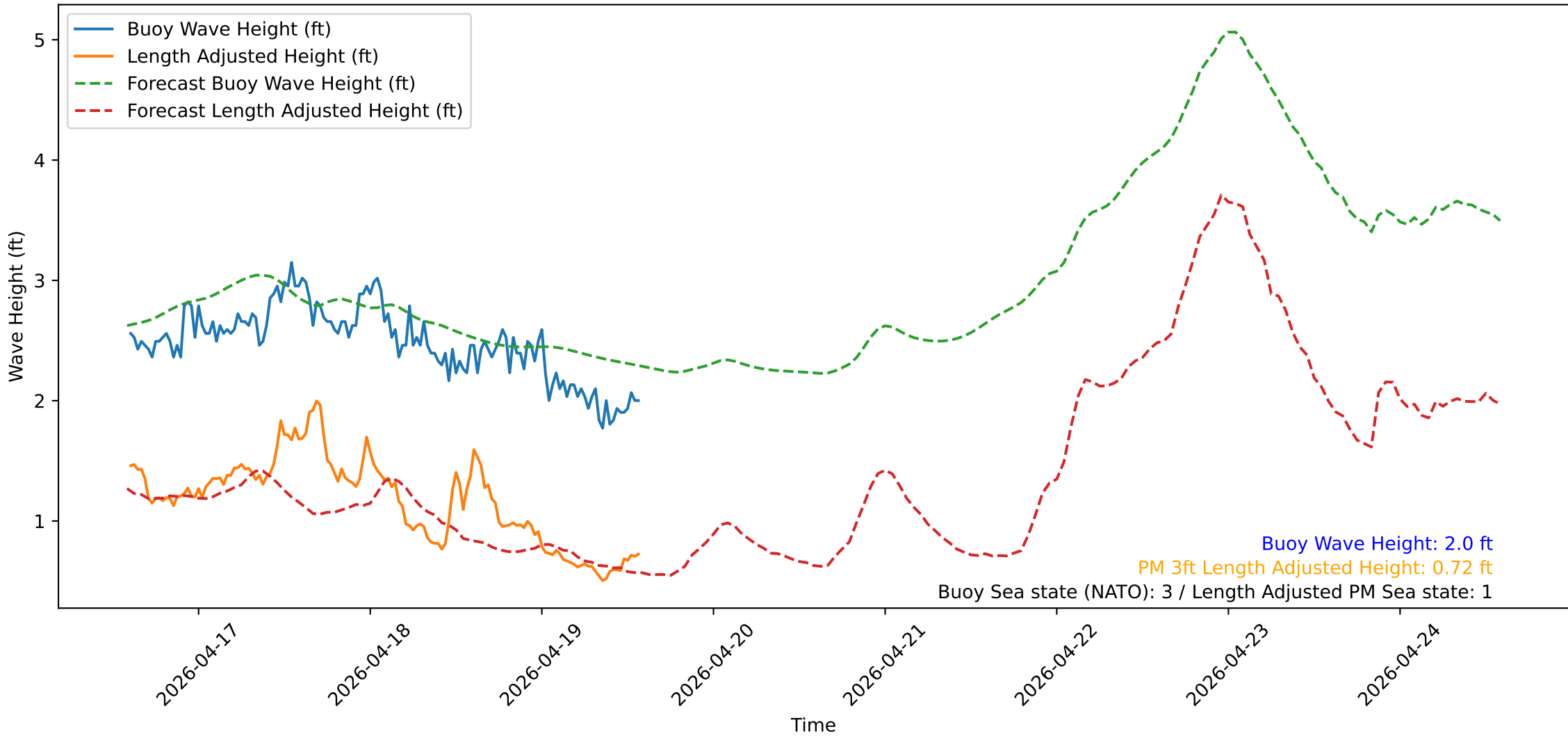
Wave Heights over Time for Red Beach at 2026-04-19 14:10:50
