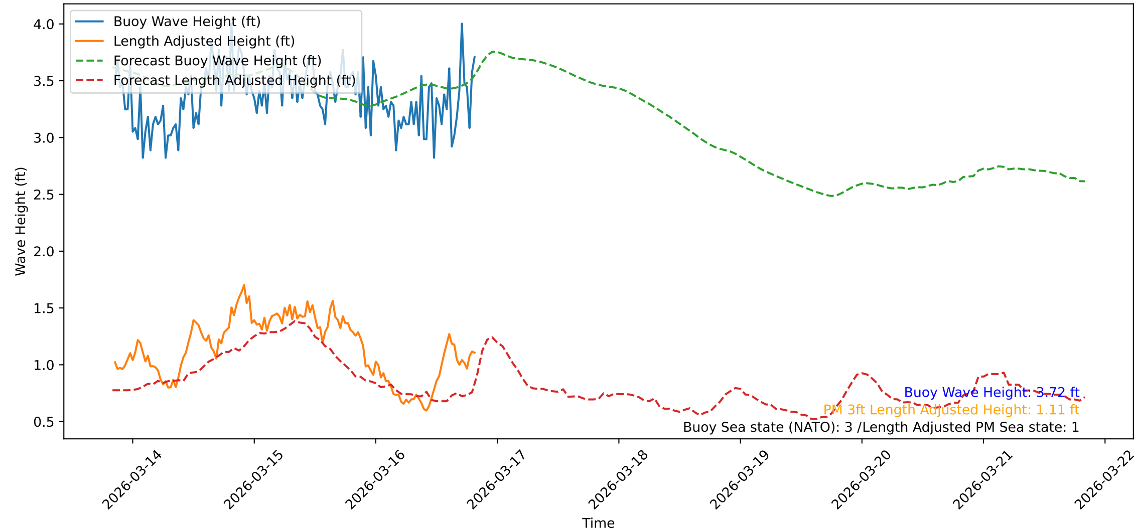
Wave Heights over Time for Green Beach at 2026-03-16 20:21:39
