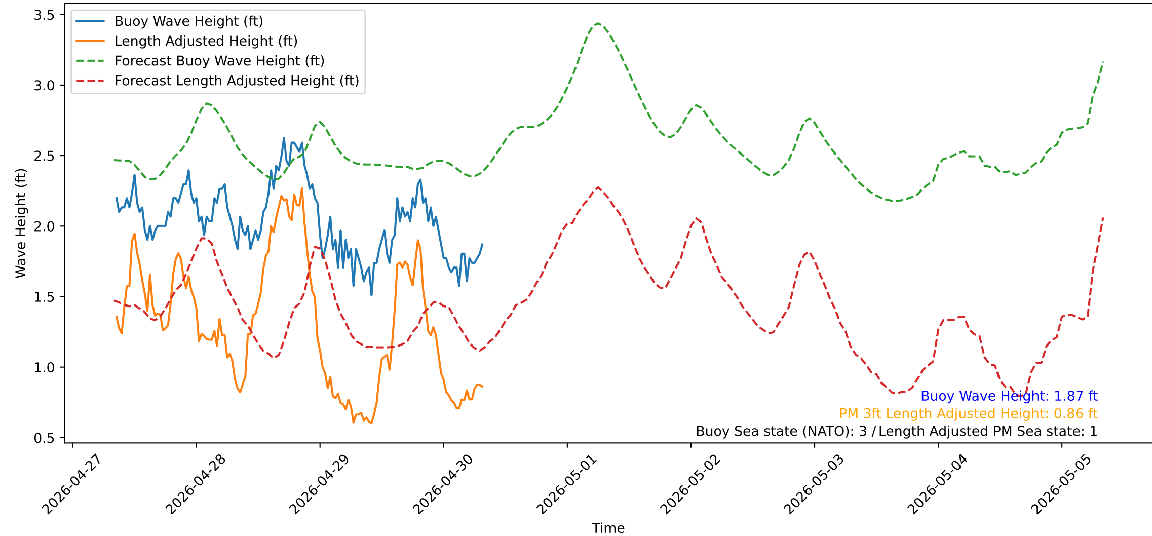
Wave Heights over Time for Red Beach at 2026-04-30 08:20:51
