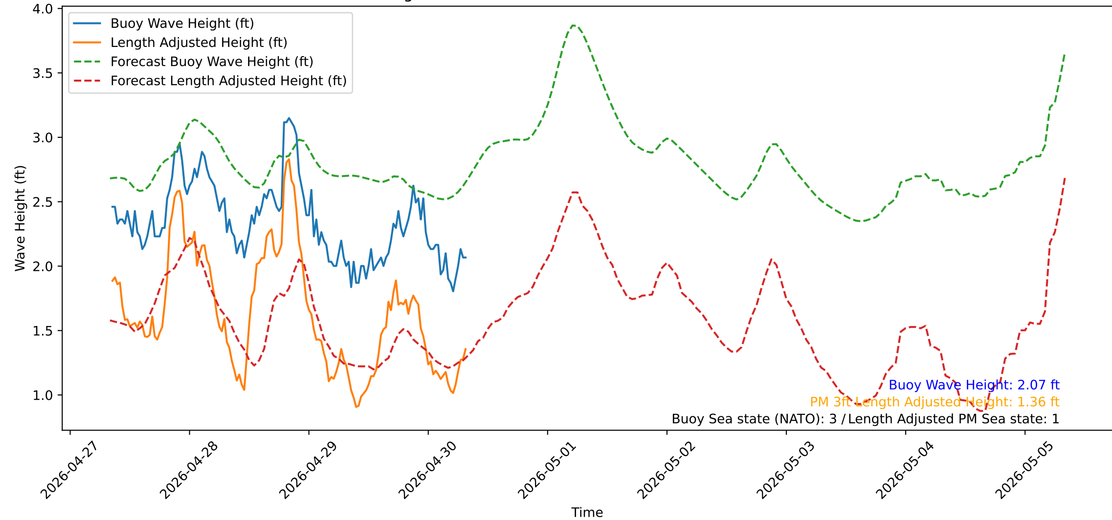
Wave Heights over Time for Green Beach at 2026-04-30 08:21:13
