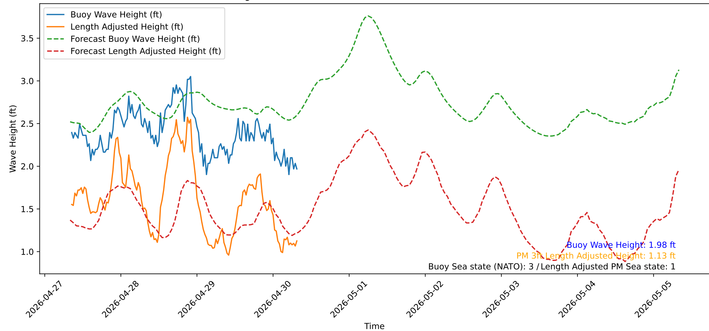
Wave Heights over Time for Oceanside Harbor at 2026-04-30 08:20:31
