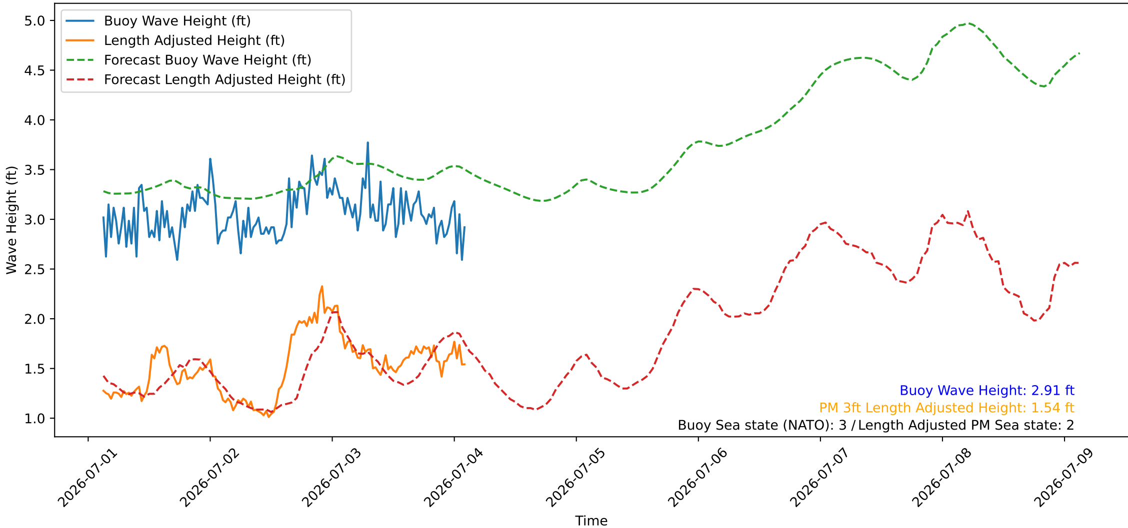
Wave Heights over Time for Oceanside Harbor at 2026-07-04 03:00:27
