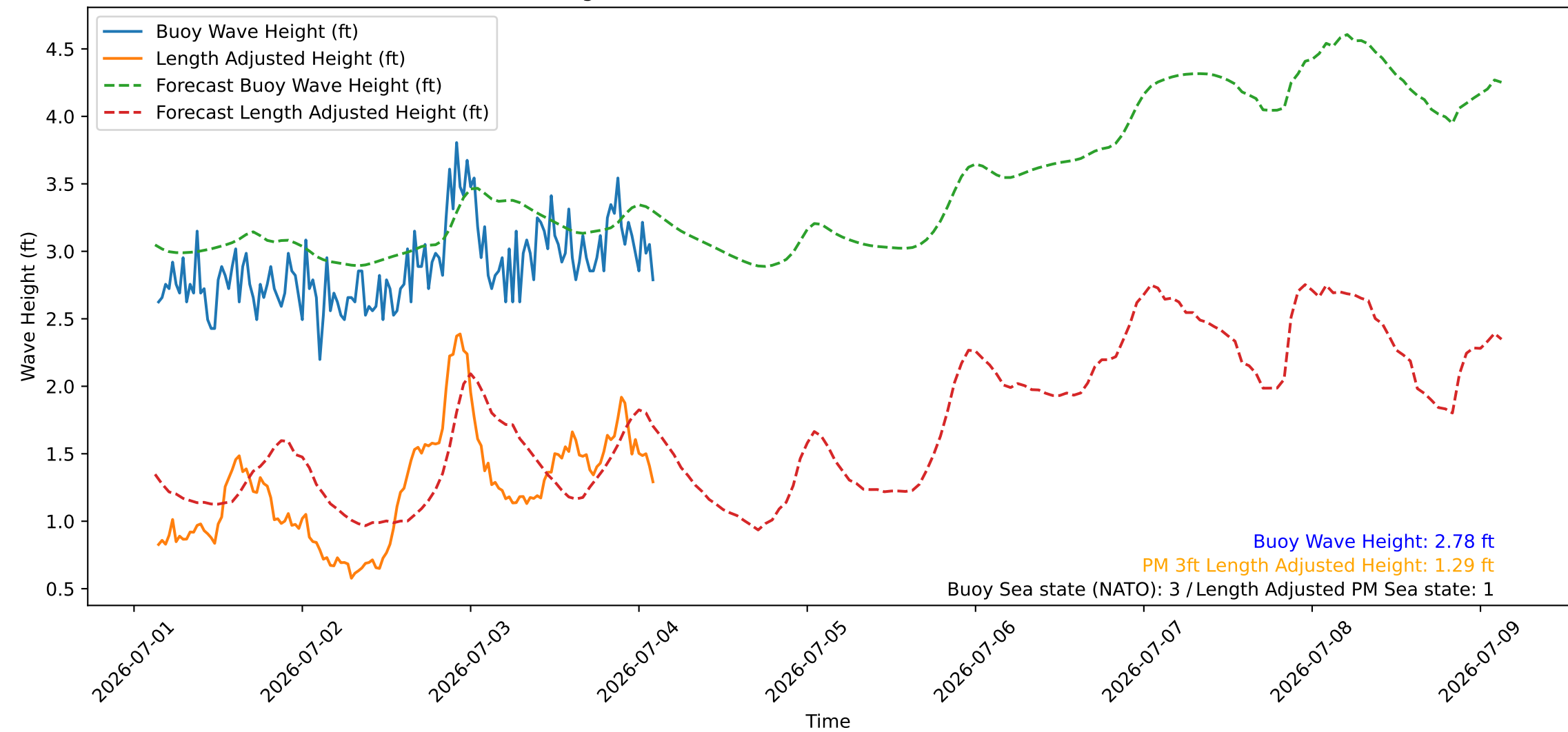
Wave Heights over Time for Red Beach at 2026-07-04 03:00:47
