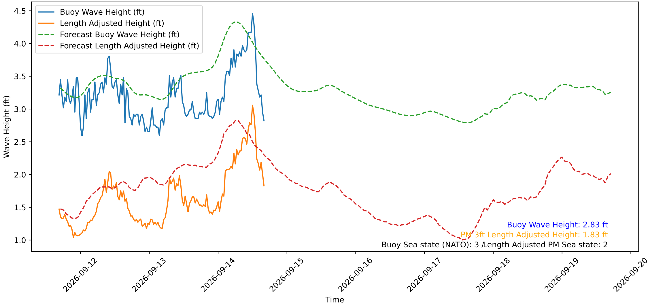
Wave Heights over Time for Oceanside Harbor at 2026-09-14 16:30:30
