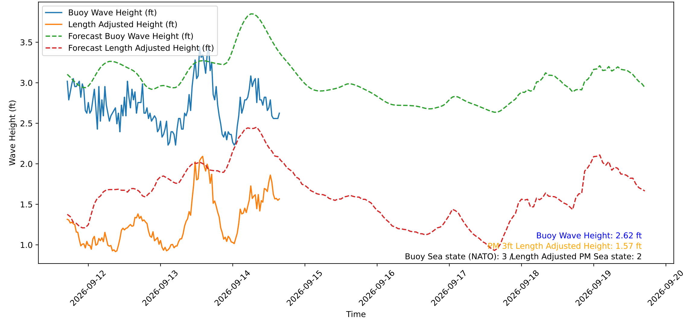
Wave Heights over Time for Red Beach at 2026-09-14 16:30:50
