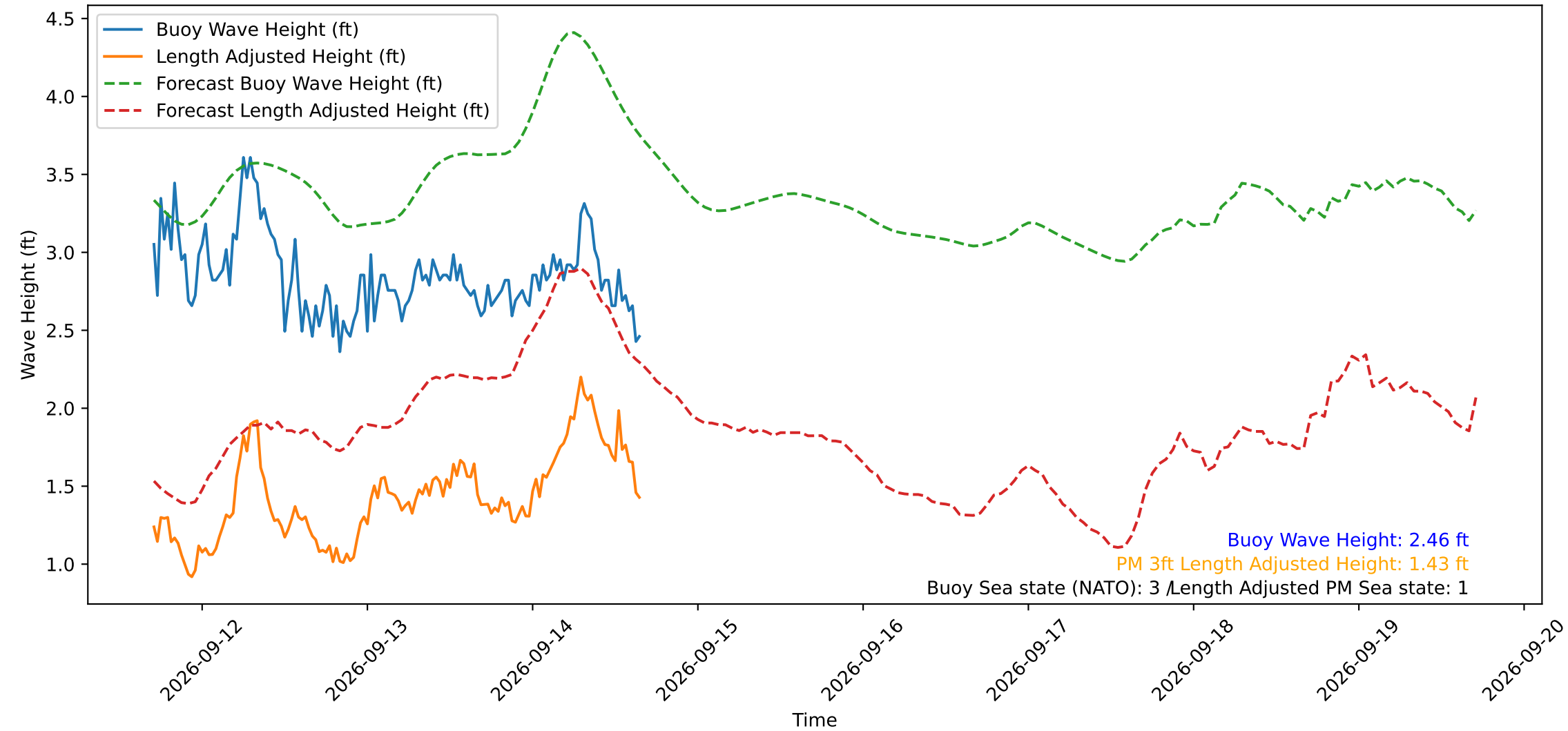
Wave Heights over Time for Green Beach at 2026-09-14 16:31:13
