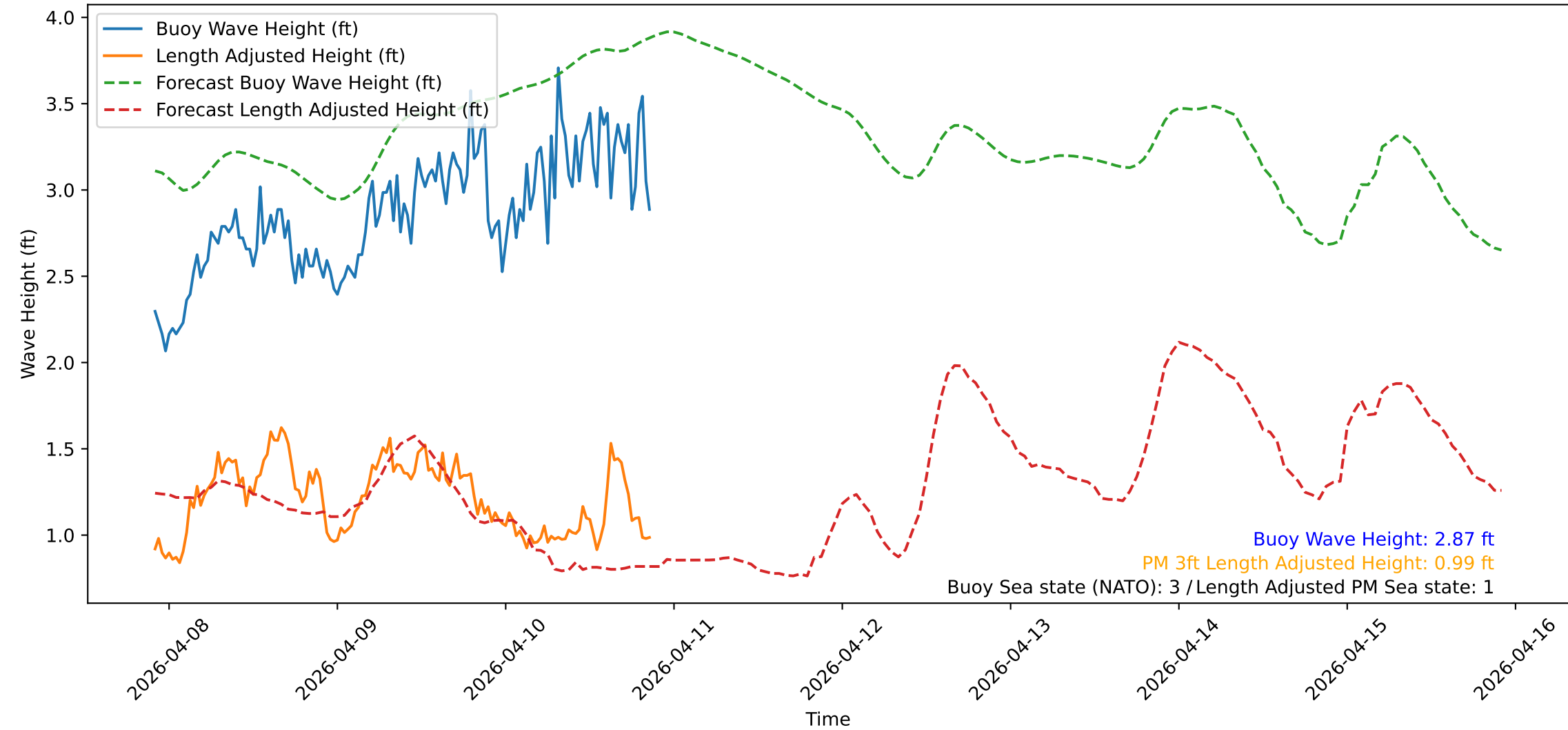
Wave Heights over Time for Red Beach at 2026-04-10 21:30:50
