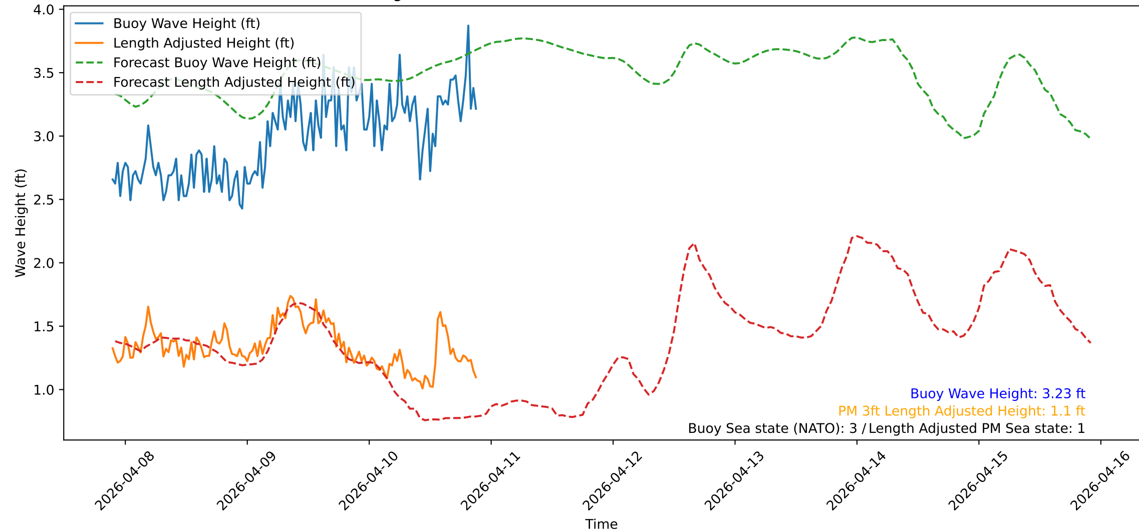
Wave Heights over Time for Oceanside Harbor at 2026-04-10 21:30:31
