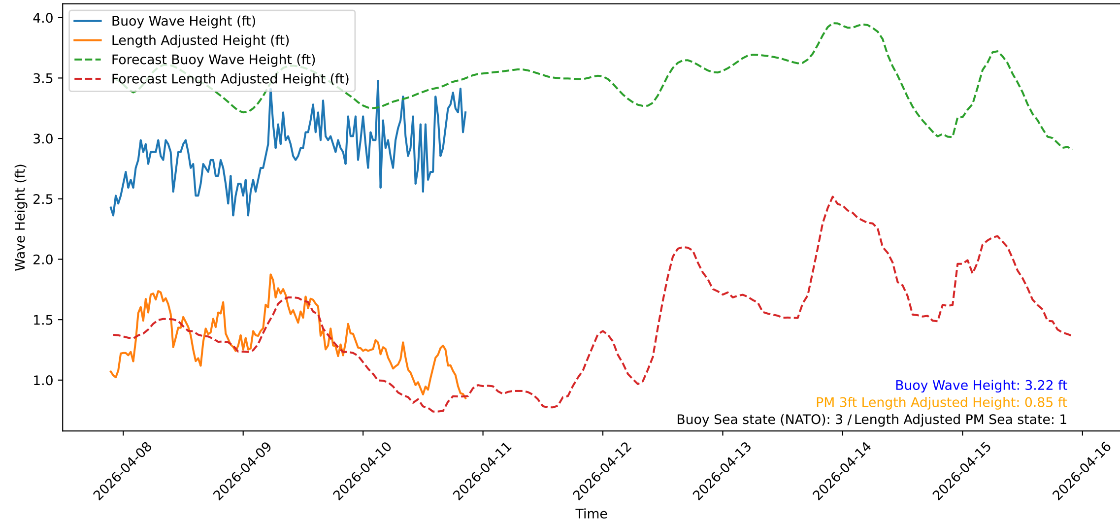
Wave Heights over Time for Green Beach at 2026-04-10 21:31:12
