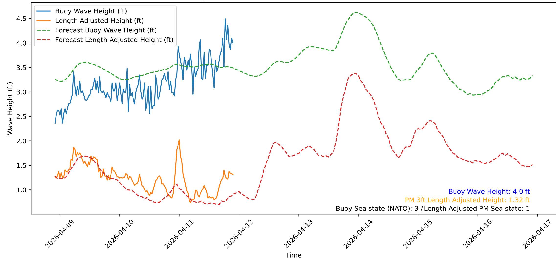
Wave Heights over Time for Green Beach at 2026-04-11 22:11:13
