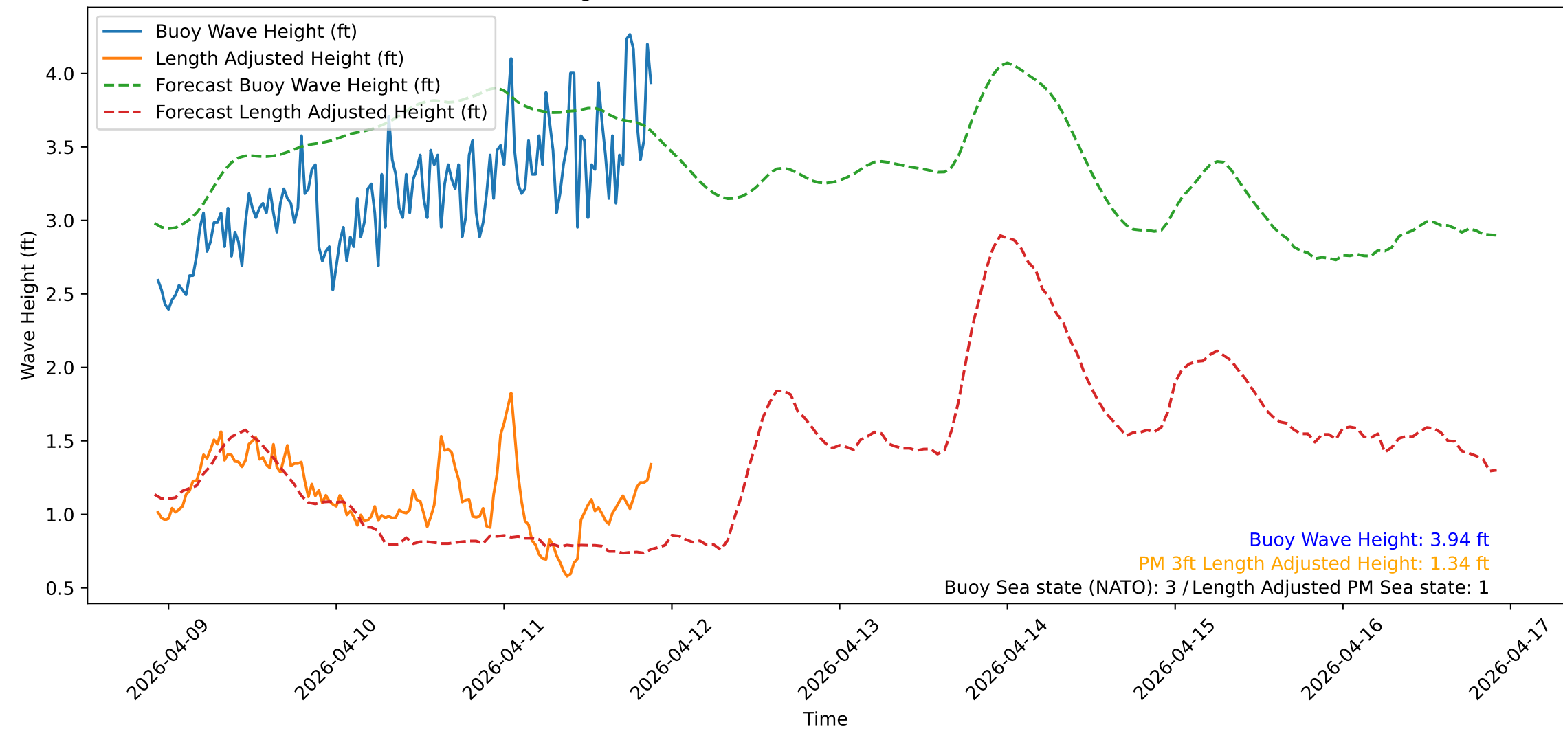
Wave Heights over Time for Red Beach at 2026-04-11 22:10:50
