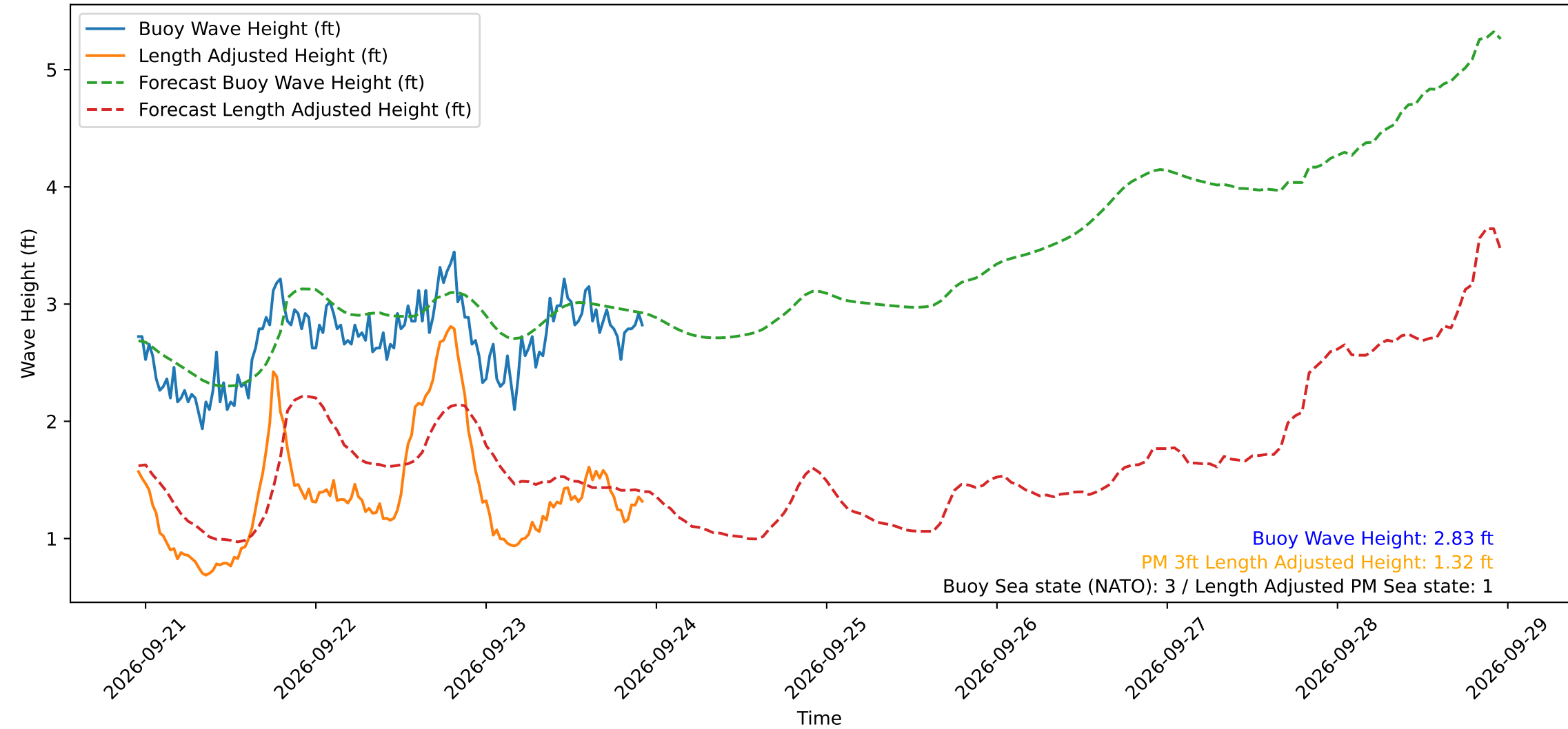
Wave Heights over Time for Green Beach at 2026-09-23 22:51:15
