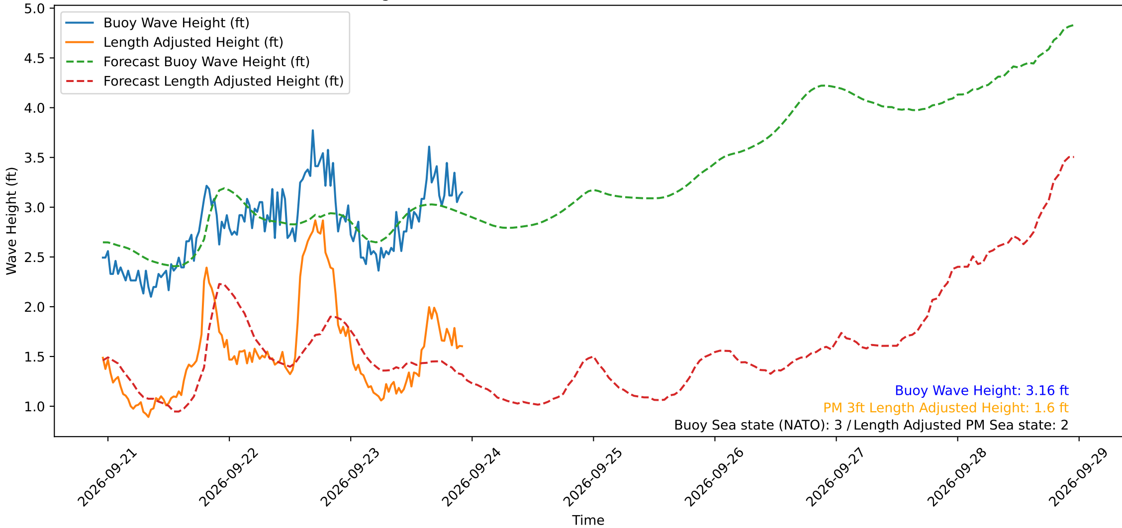
Wave Heights over Time for Oceanside Harbor at 2026-09-23 22:50:29
