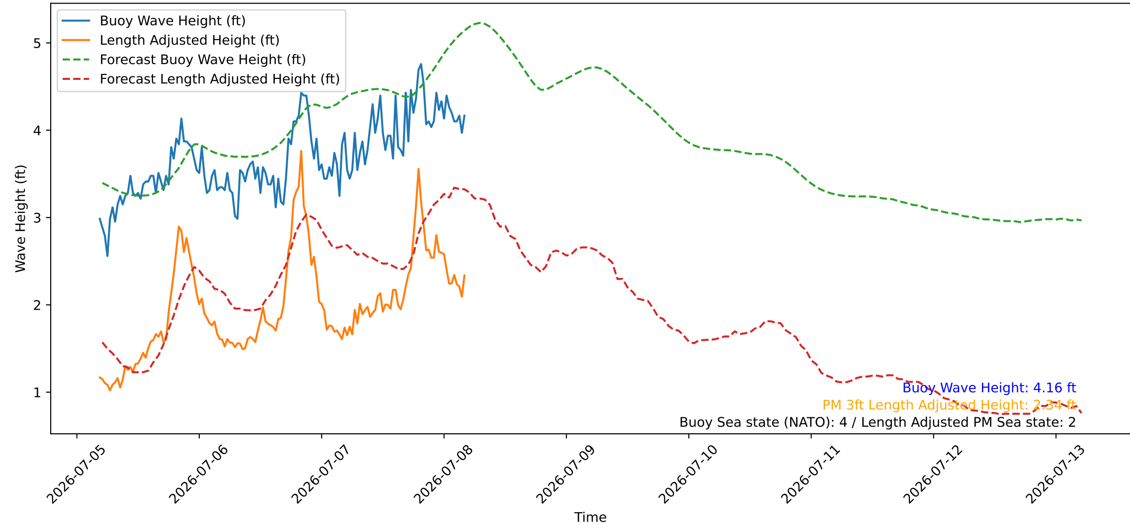
Wave Heights over Time for Green Beach at 2026-07-08 04:41:09
