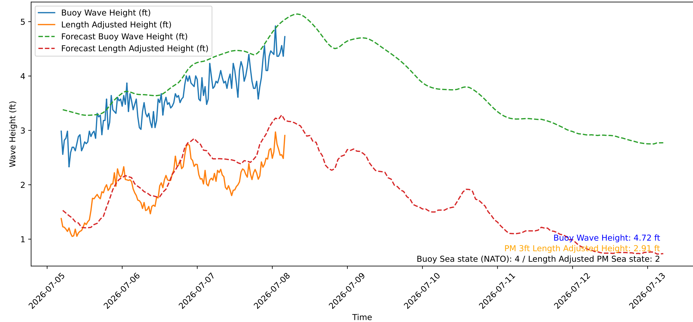
Wave Heights over Time for Oceanside Harbor at 2026-07-08 04:40:27
