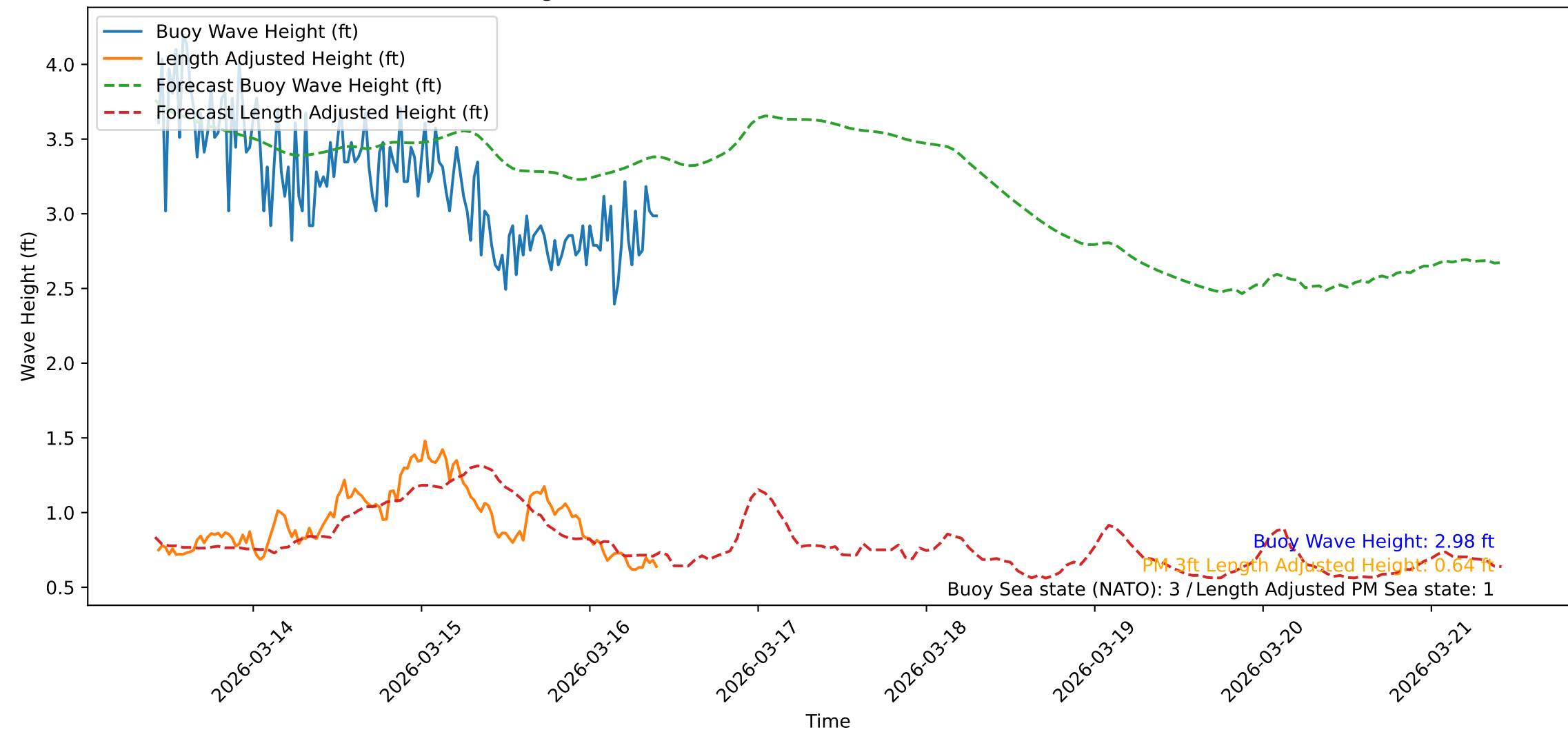
Wave Heights over Time for Oceanside Harbor at 2026-03-16 10:20:40
