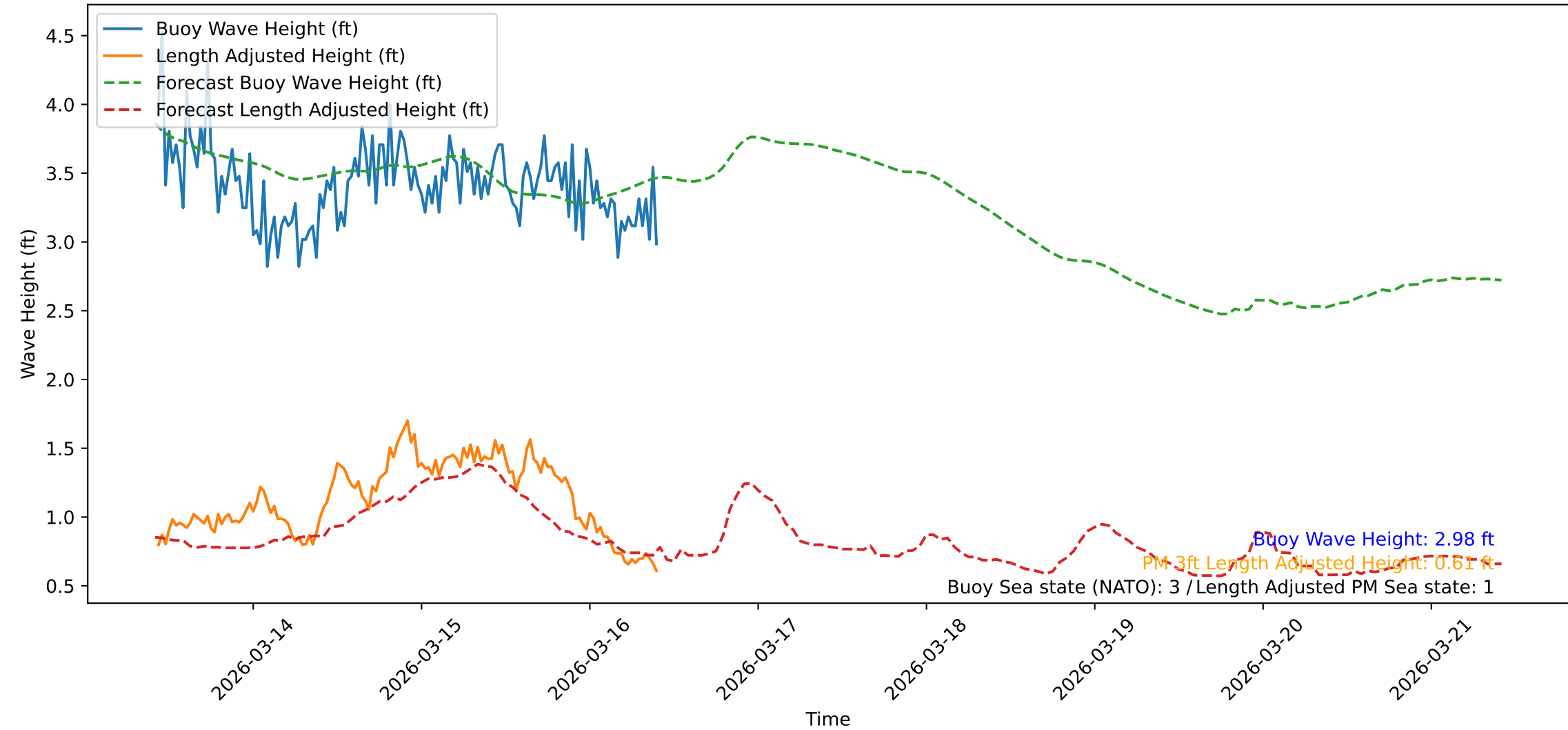
Wave Heights over Time for Green Beach at 2026-03-16 10:21:37
