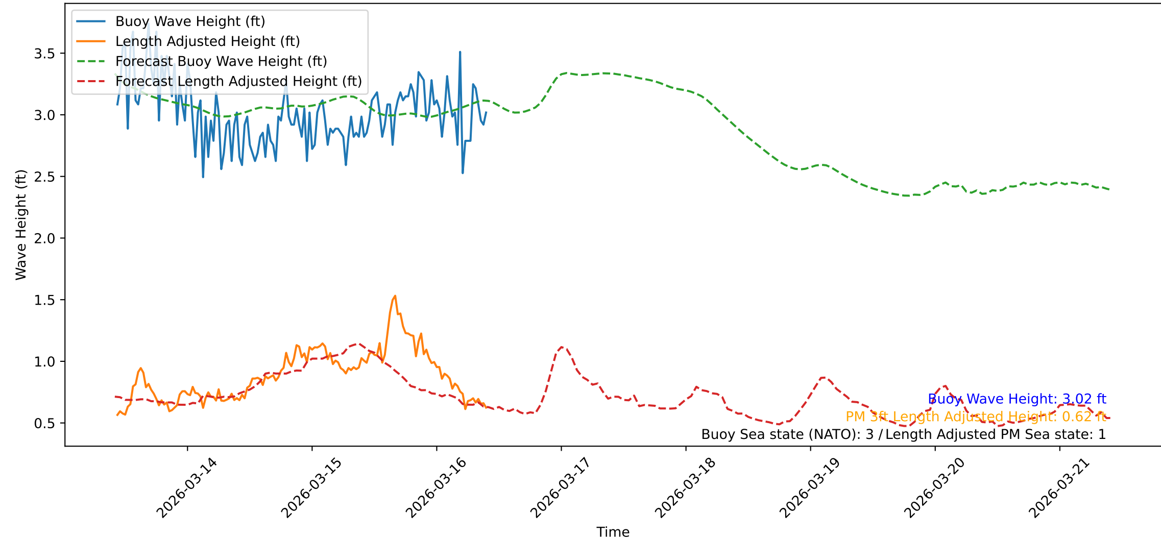
Wave Heights over Time for Red Beach at 2026-03-16 10:21:03
