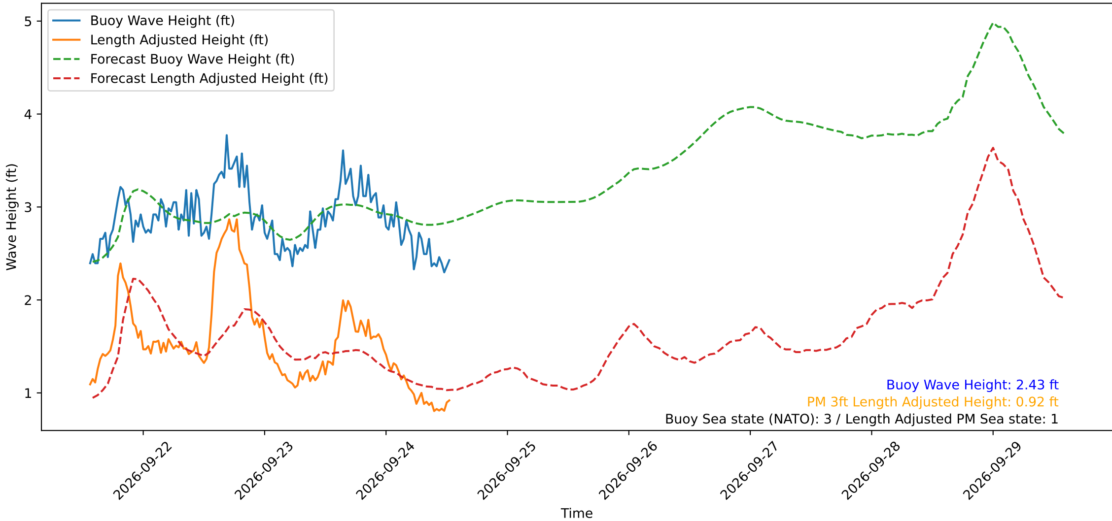
Wave Heights over Time for Oceanside Harbor at 2026-09-24 13:30:31
