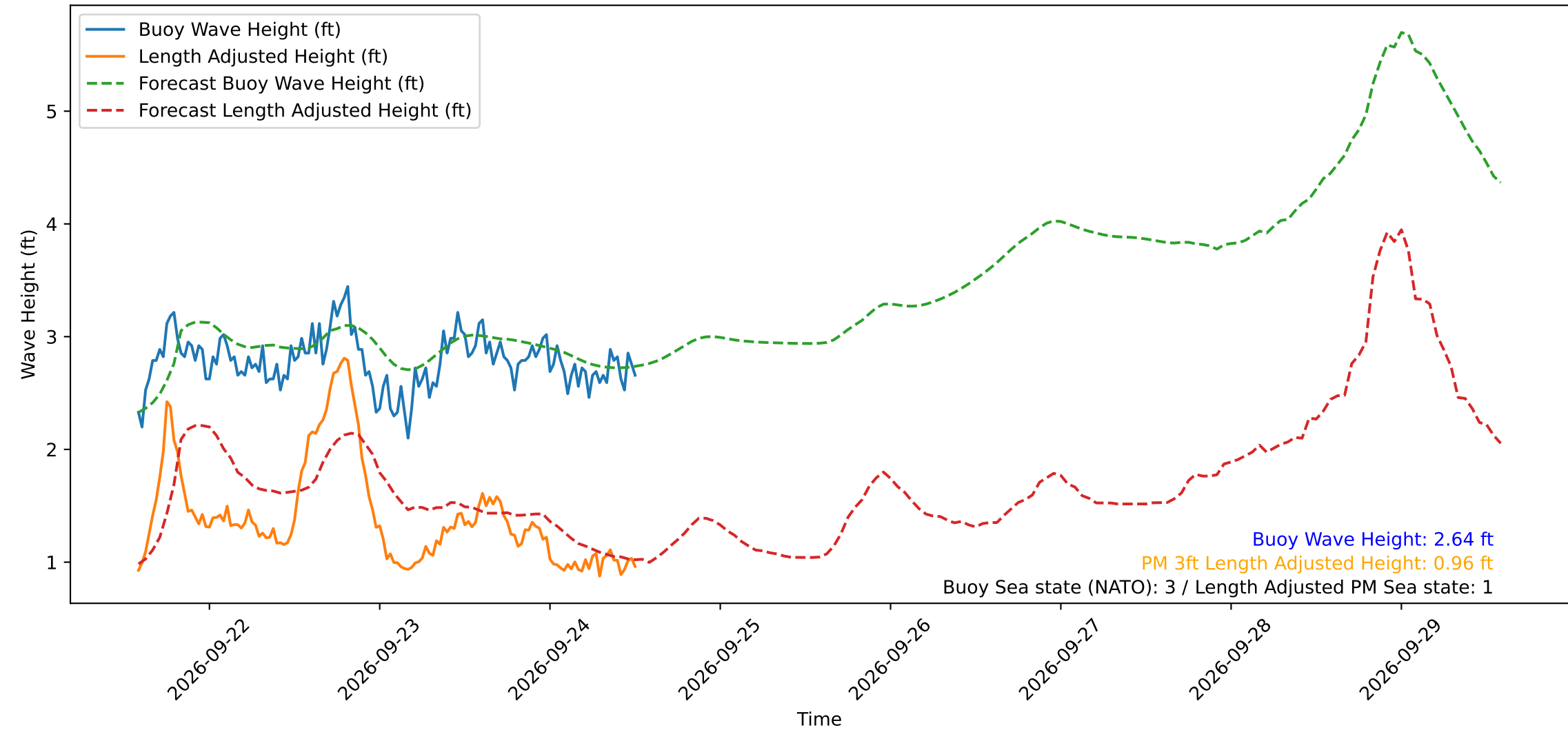
Wave Heights over Time for Green Beach at 2026-09-24 13:31:16
