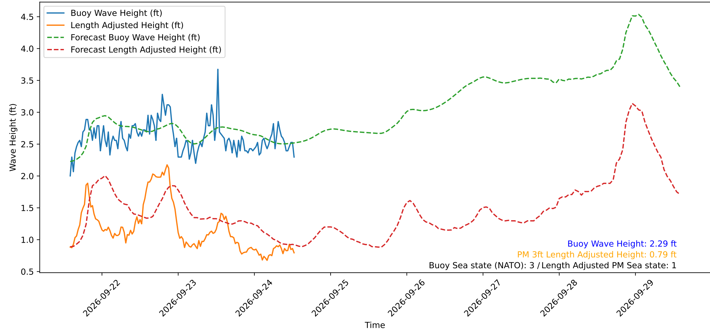
Wave Heights over Time for Red Beach at 2026-09-24 13:30:52
