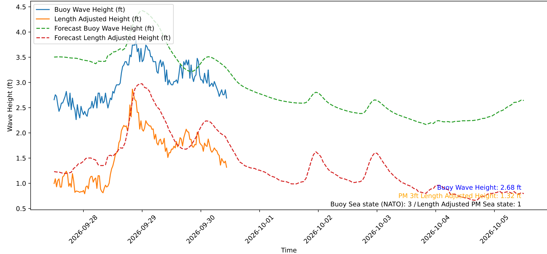
Wave Heights over Time for Red Beach at 2026-09-30 11:30:49
