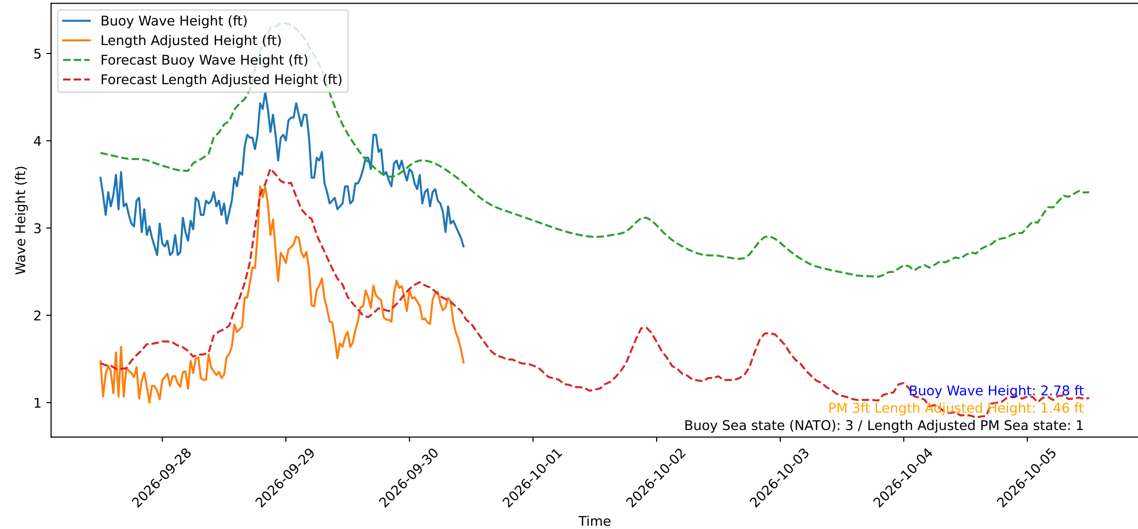
Wave Heights over Time for Green Beach at 2026-09-30 11:31:12
