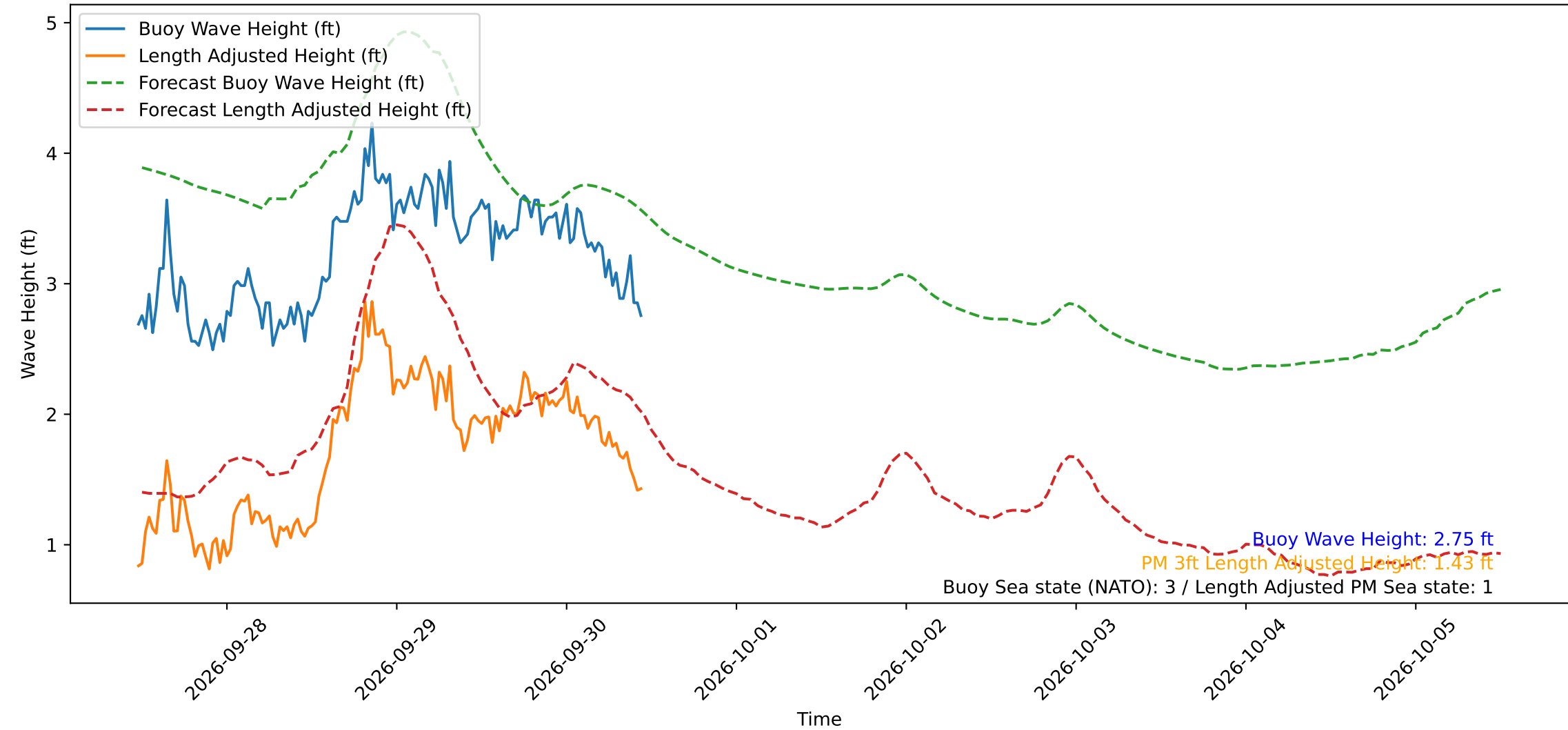
Wave Heights over Time for Oceanside Harbor at 2026-09-30 11:30:29
