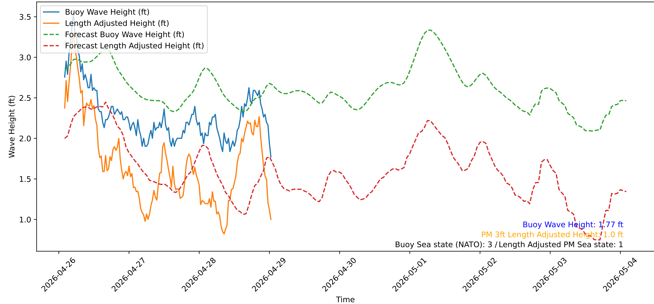
Wave Heights over Time for Red Beach at 2026-04-29 01:30:50
