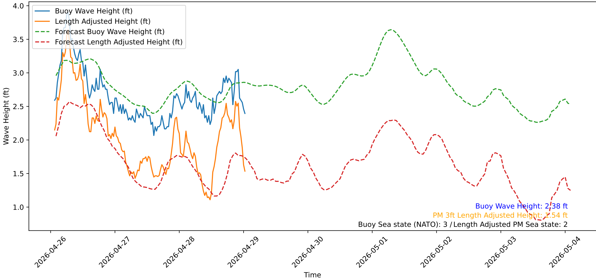
Wave Heights over Time for Oceanside Harbor at 2026-04-29 01:30:31
