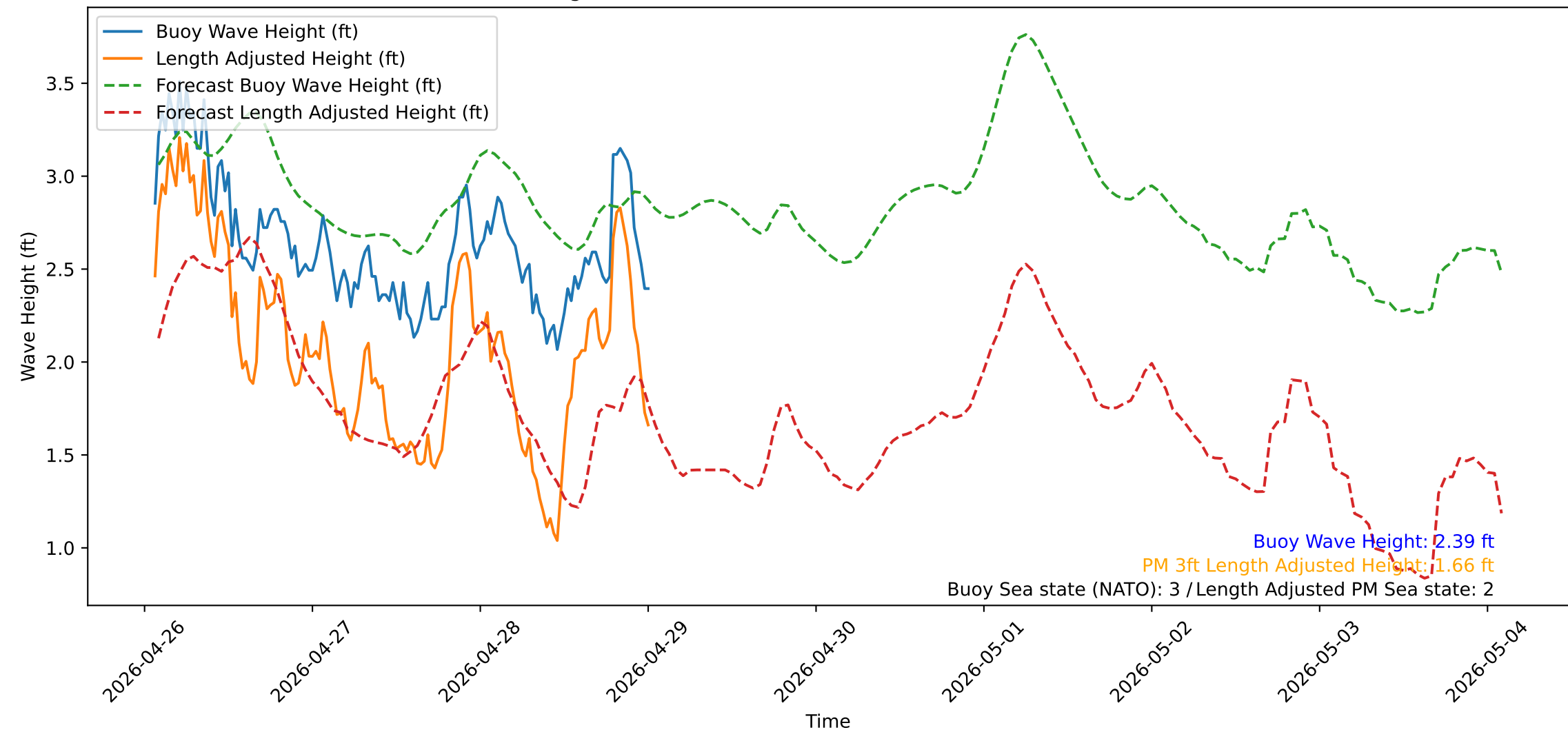
Wave Heights over Time for Green Beach at 2026-04-29 01:31:12
