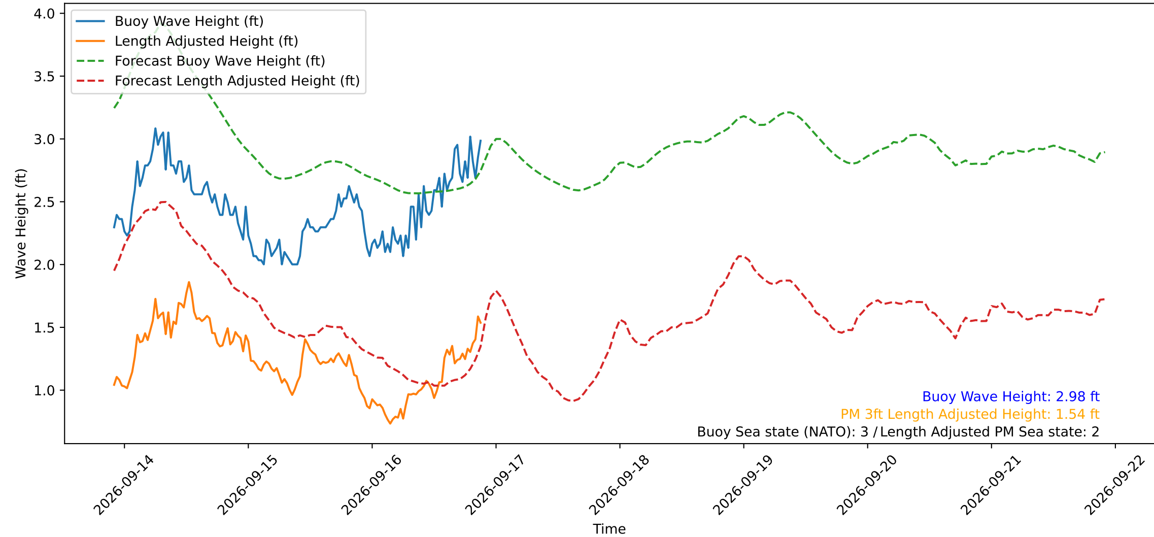
Wave Heights over Time for Red Beach at 2026-09-16 21:50:49
