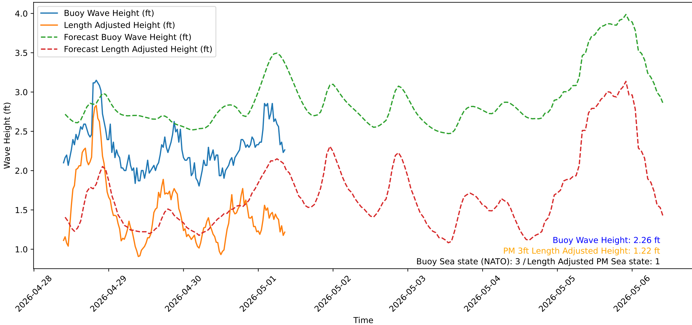
Wave Heights over Time for Green Beach at 2026-05-01 09:31:13
