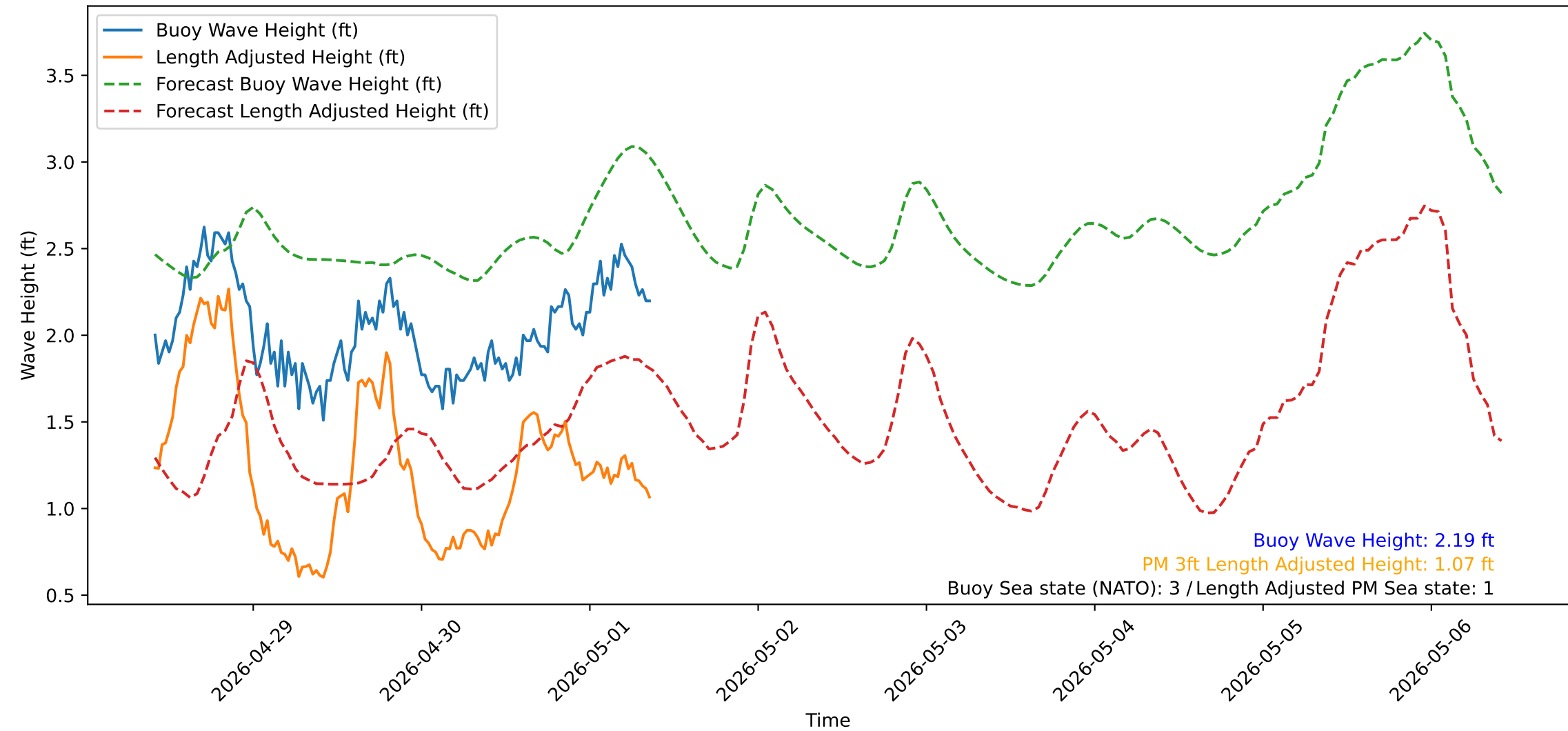
Wave Heights over Time for Red Beach at 2026-05-01 09:30:51
