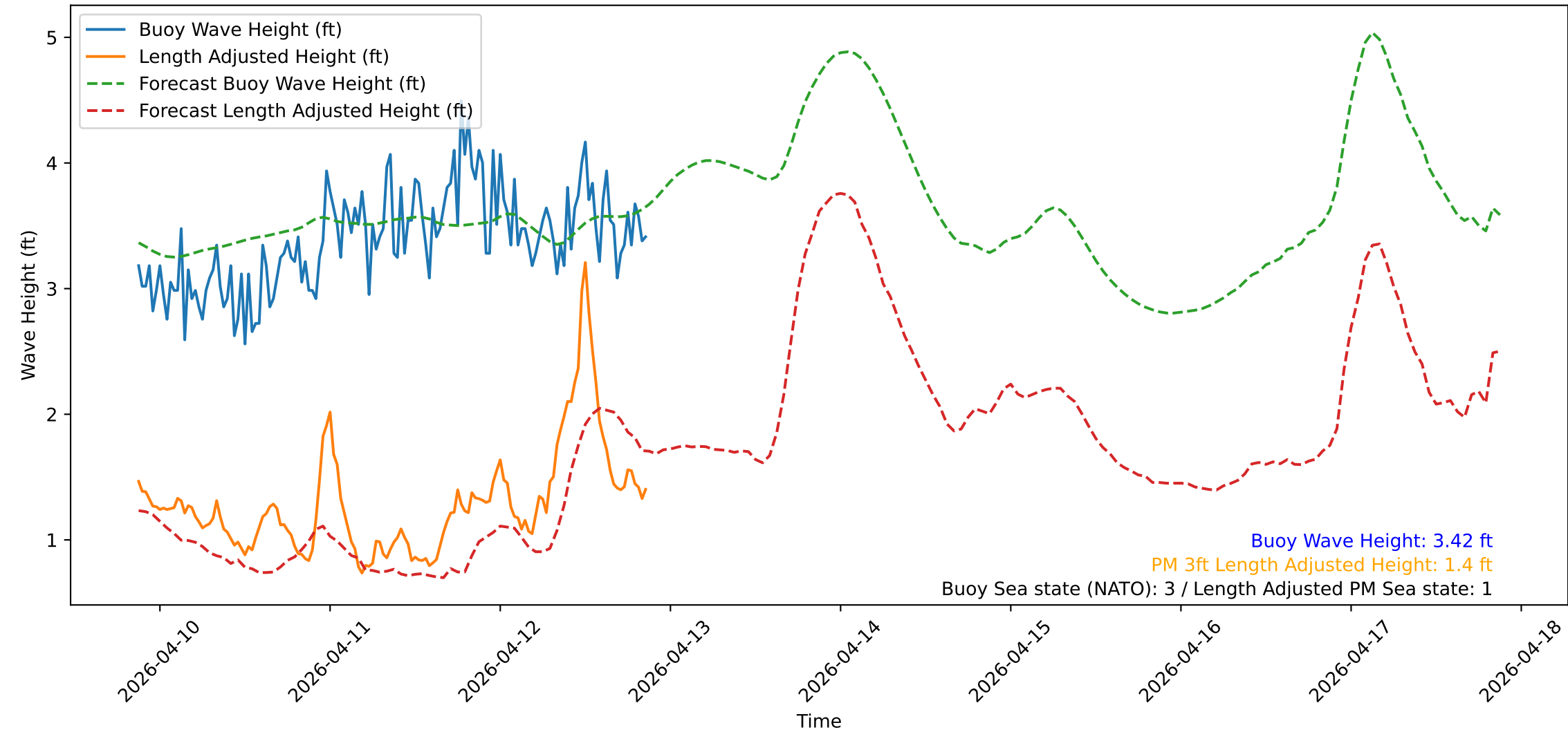
Wave Heights over Time for Green Beach at 2026-04-12 21:11:11
