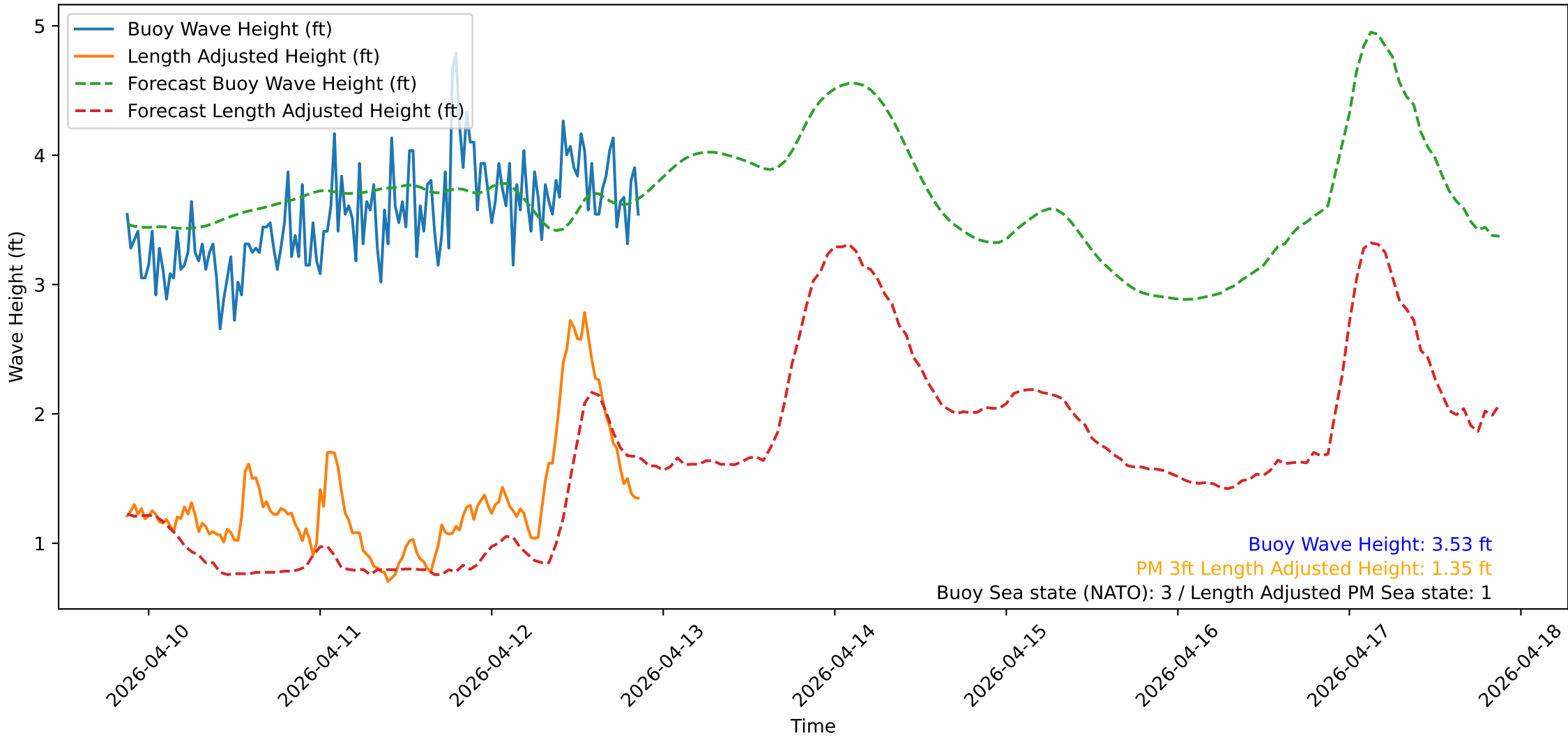
Wave Heights over Time for Oceanside Harbor at 2026-04-12 21:10:30
