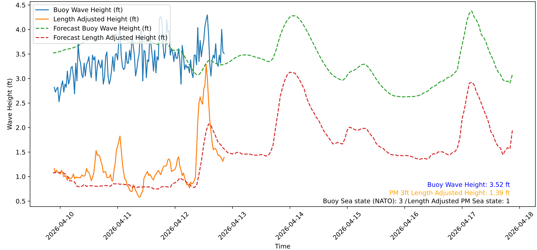
Wave Heights over Time for Red Beach at 2026-04-12 21:10:49
