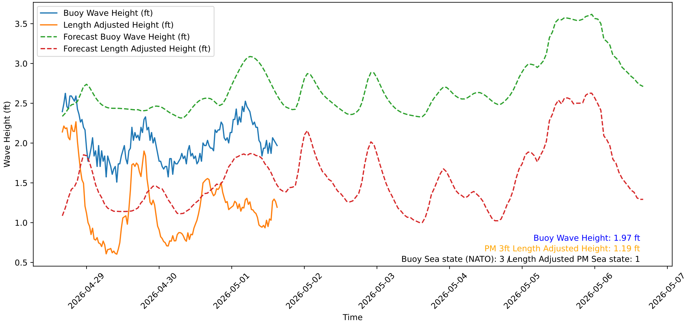
Wave Heights over Time for Red Beach at 2026-05-01 15:50:53
