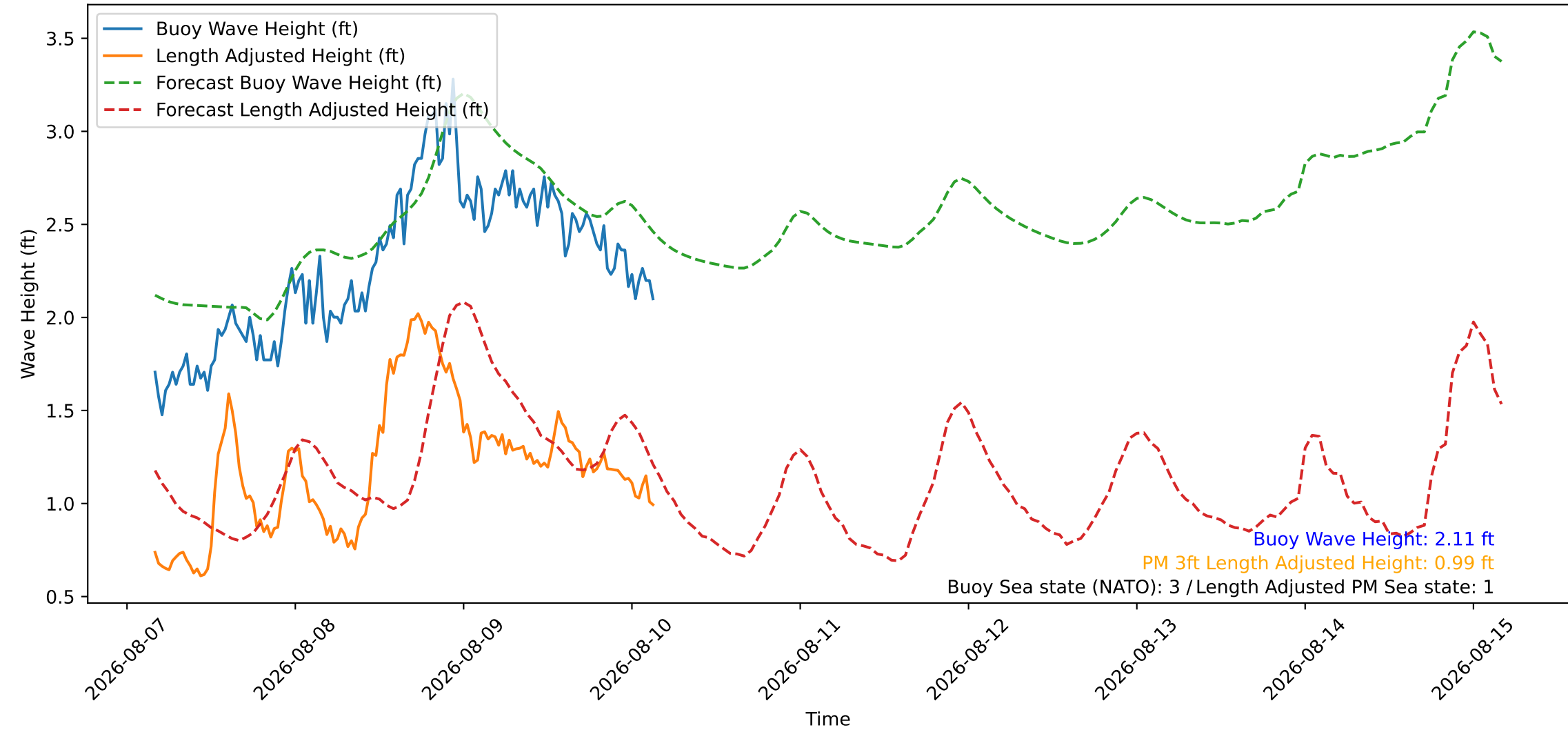
Wave Heights over Time for Red Beach at 2026-08-10 03:50:47
