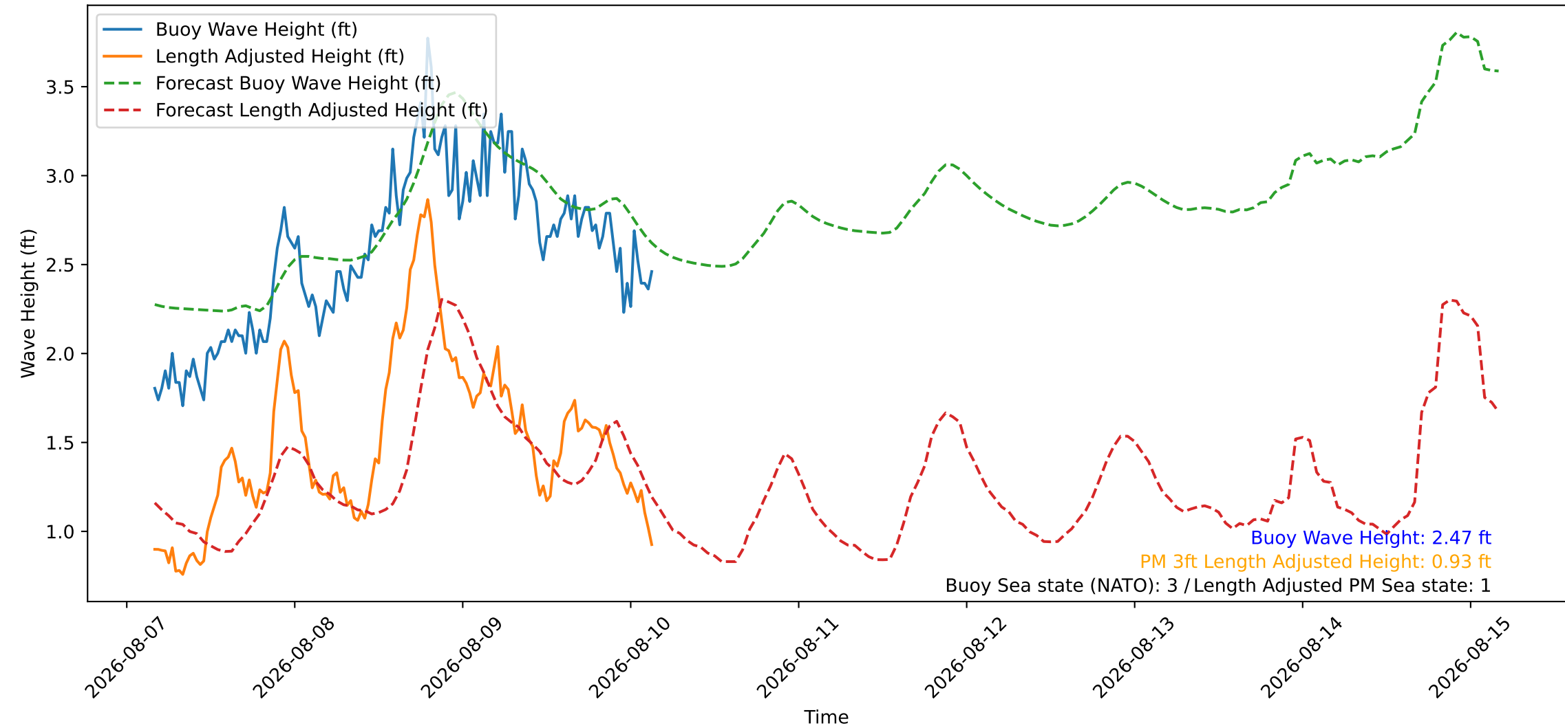
Wave Heights over Time for Green Beach at 2026-08-10 03:51:09
