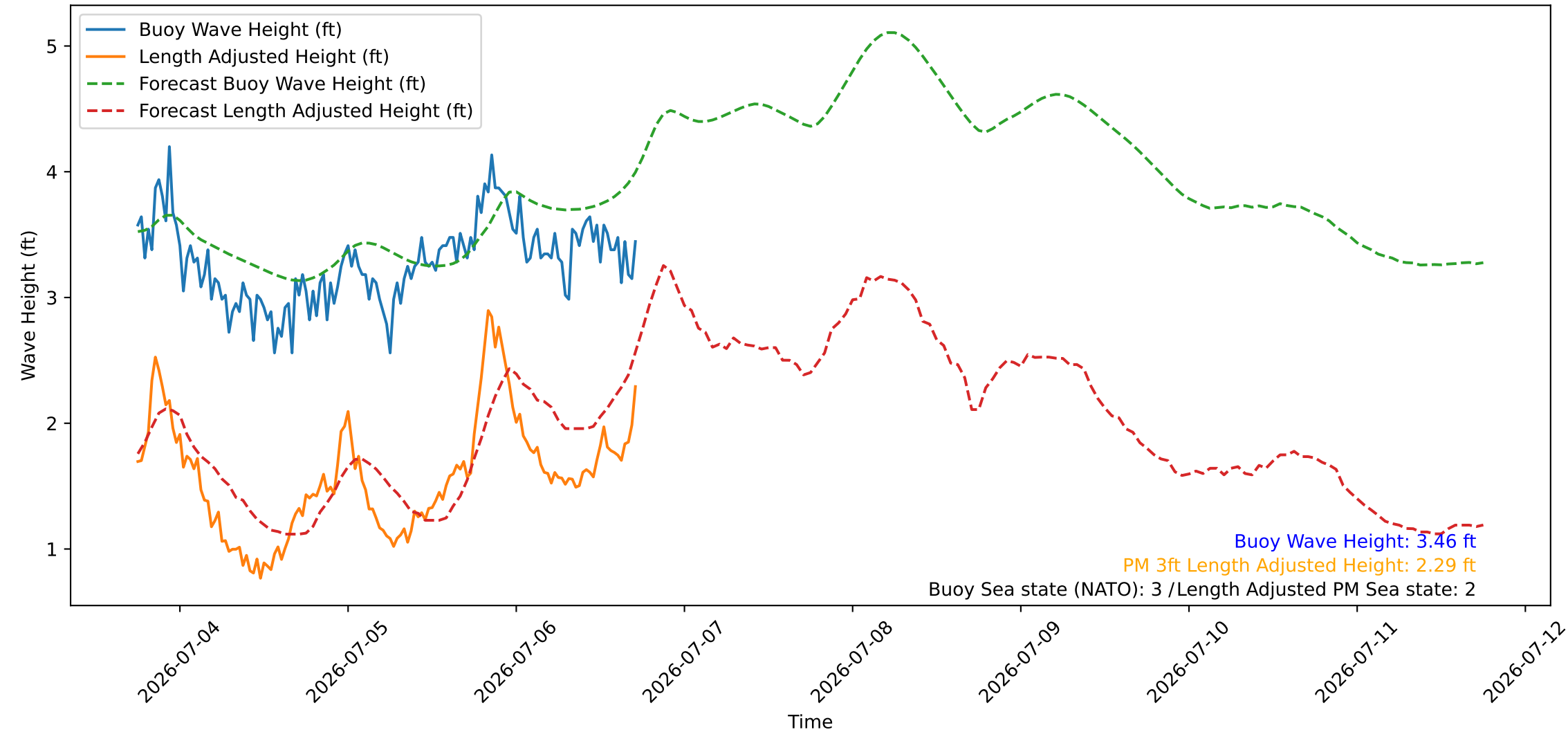
Wave Heights over Time for Green Beach at 2026-07-06 18:01:08
