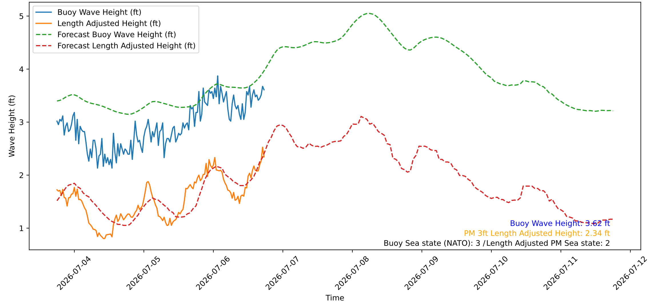
Wave Heights over Time for Oceanside Harbor at 2026-07-06 18:00:26
