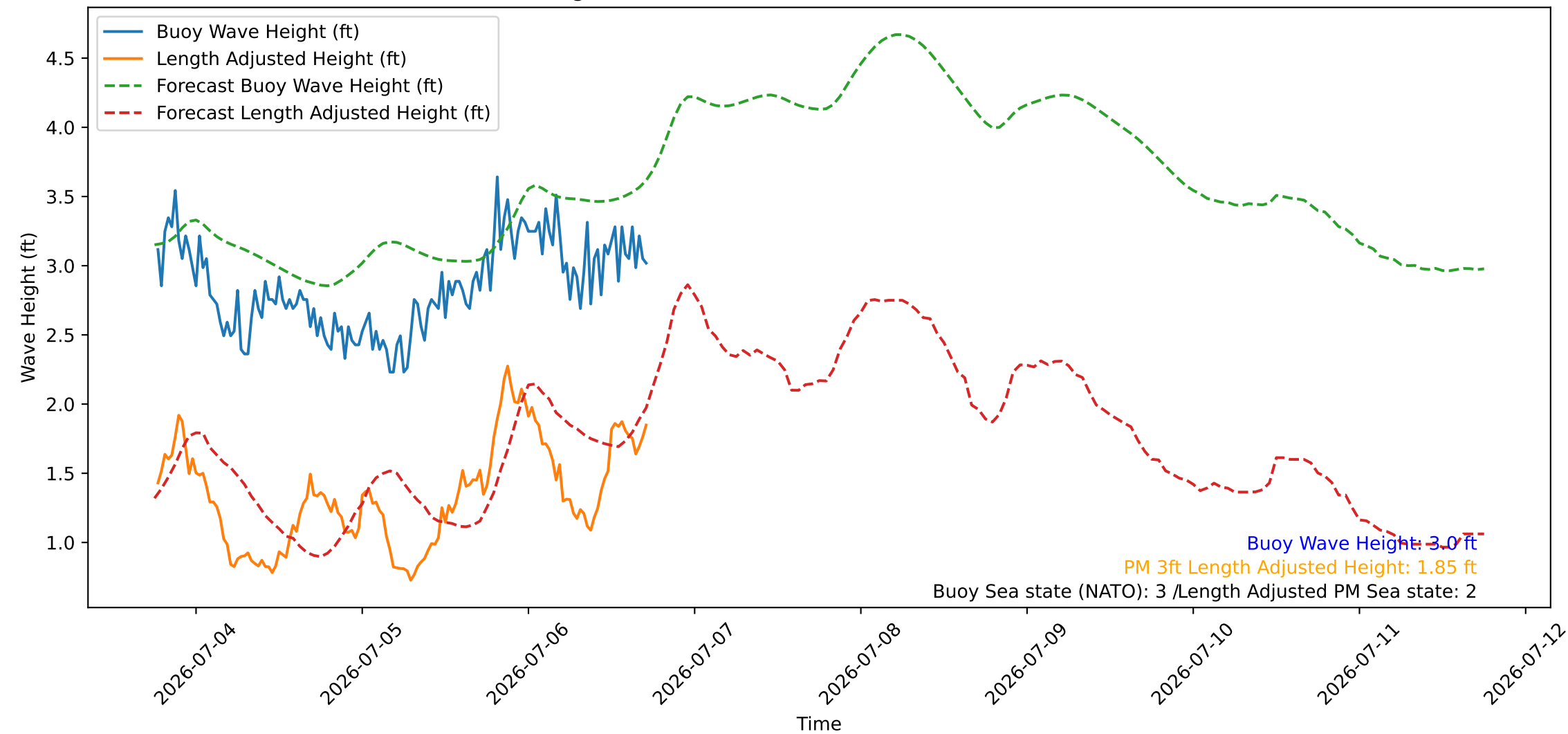
Wave Heights over Time for Red Beach at 2026-07-06 18:00:46
