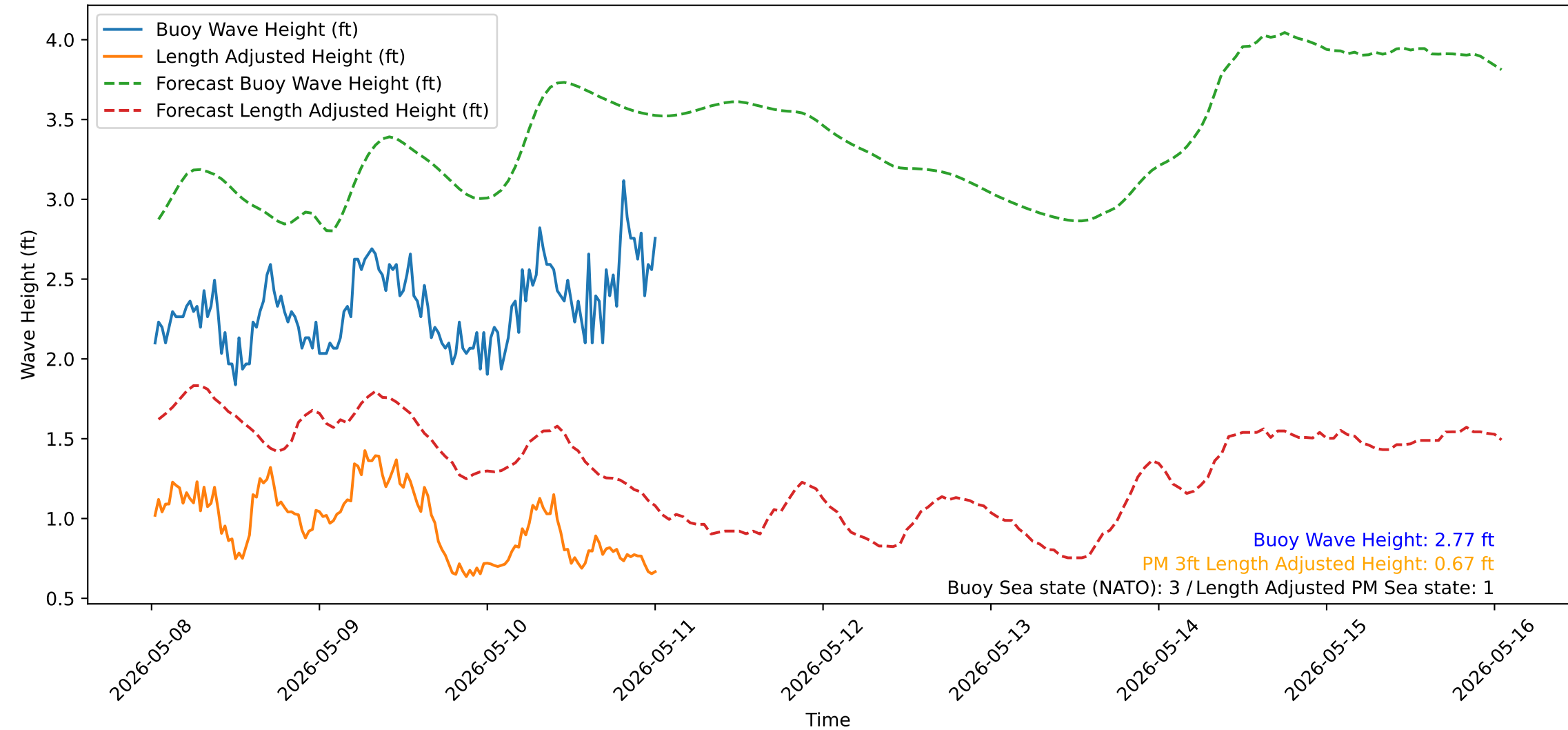
Wave Heights over Time for Green Beach at 2026-05-11 00:41:13
