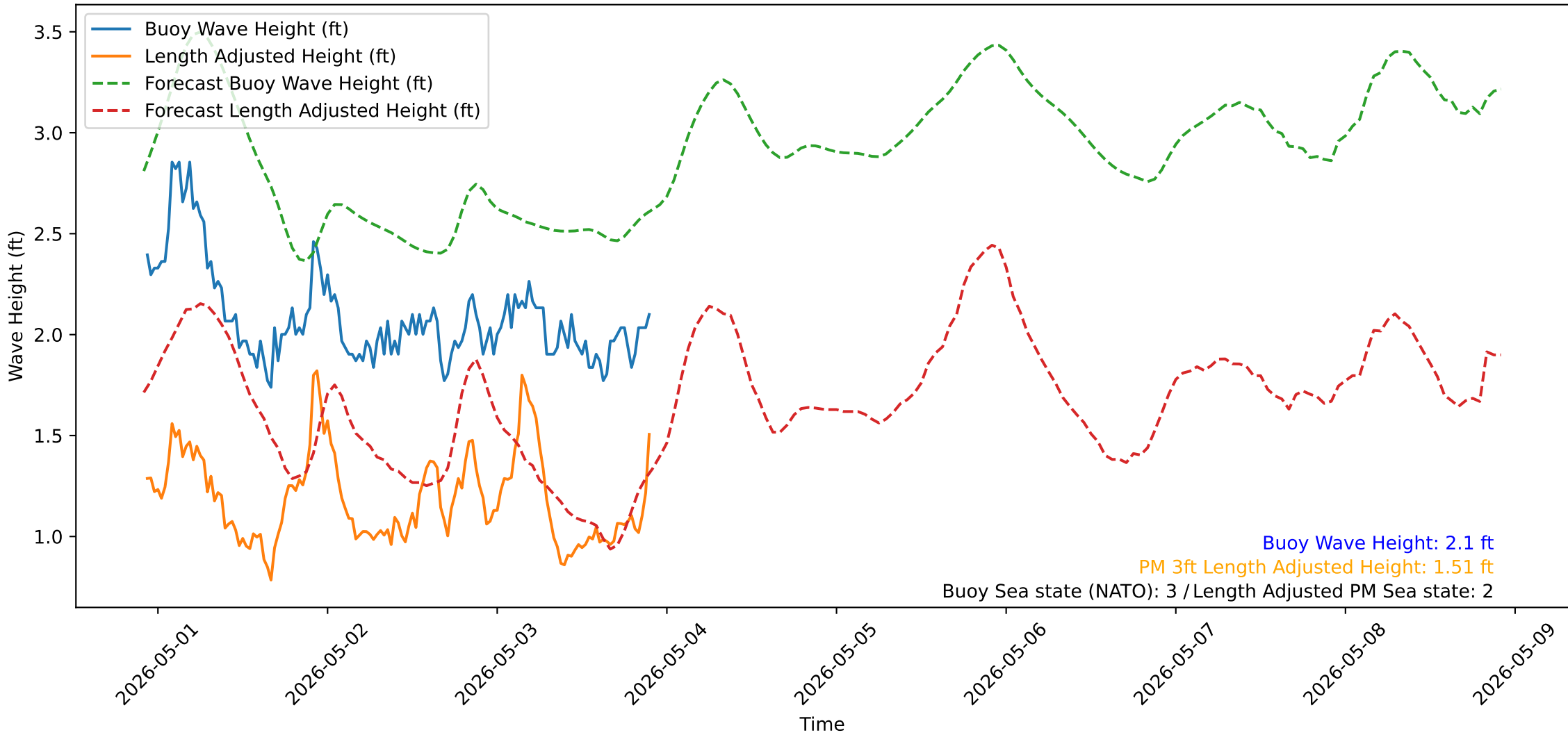
Wave Heights over Time for Green Beach at 2026-05-03 22:21:13
