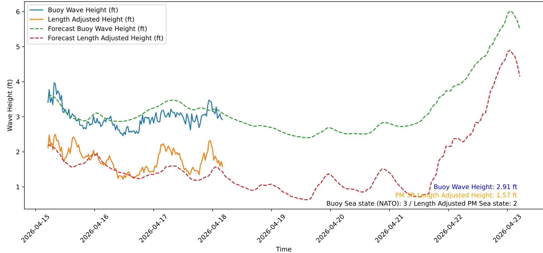
Wave Heights over Time for Green Beach at 2026-04-18 05:01:13
