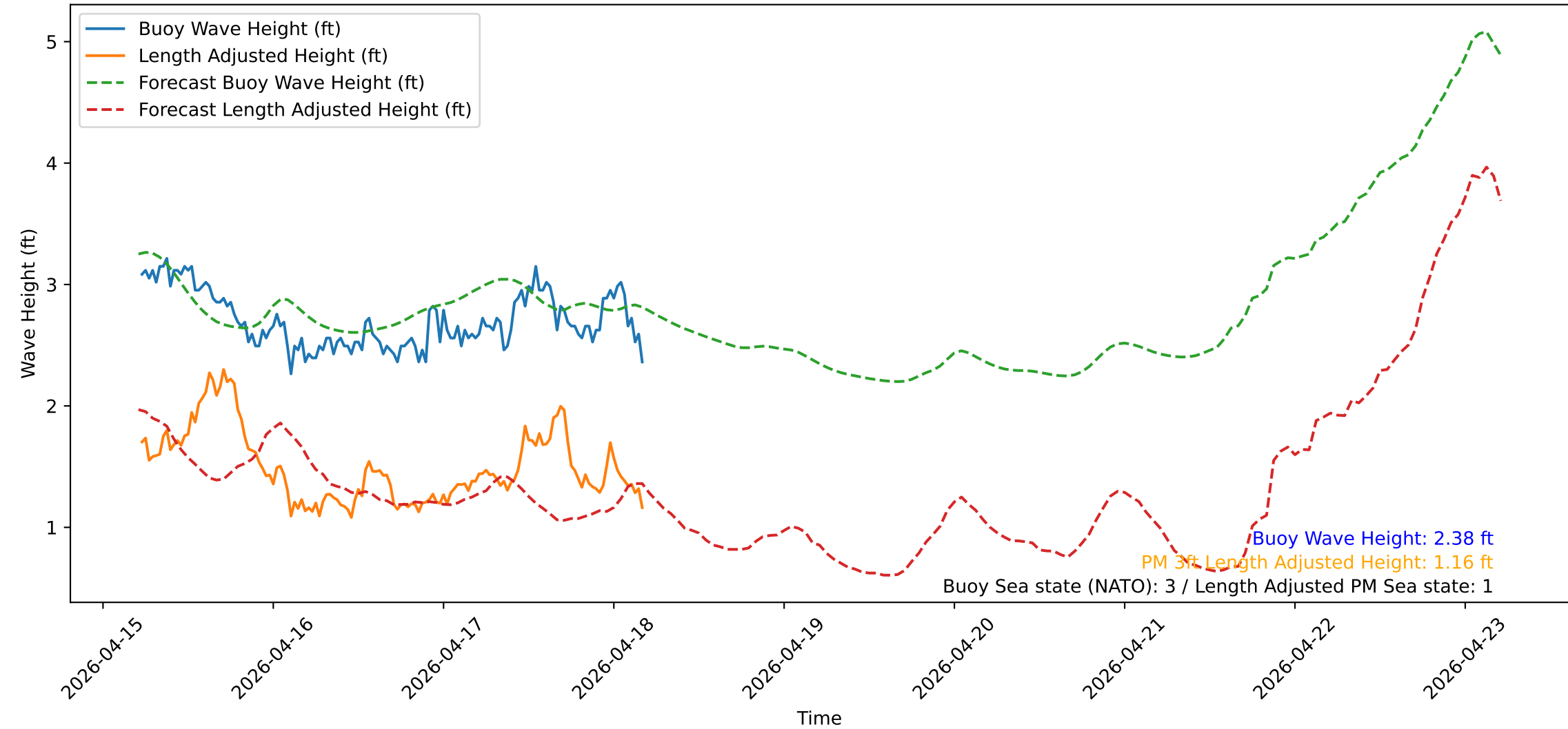
Wave Heights over Time for Red Beach at 2026-04-18 05:00:51
