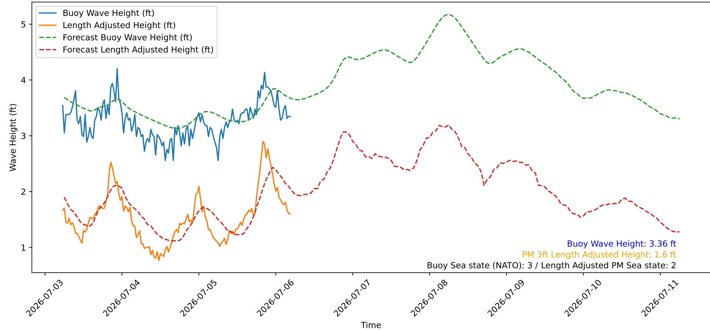
Wave Heights over Time for Green Beach at 2026-07-06 05:31:08
