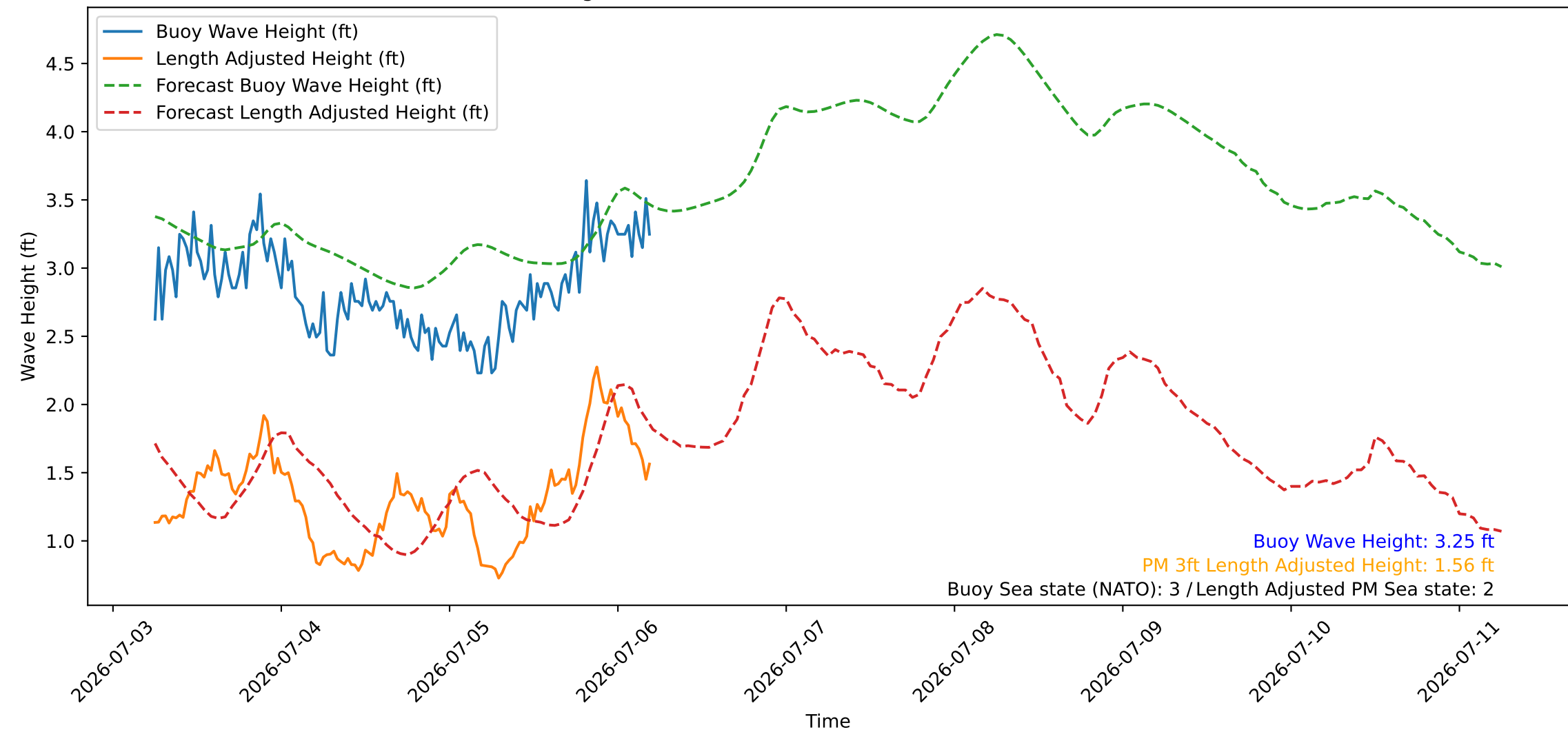
Wave Heights over Time for Red Beach at 2026-07-06 05:30:46
