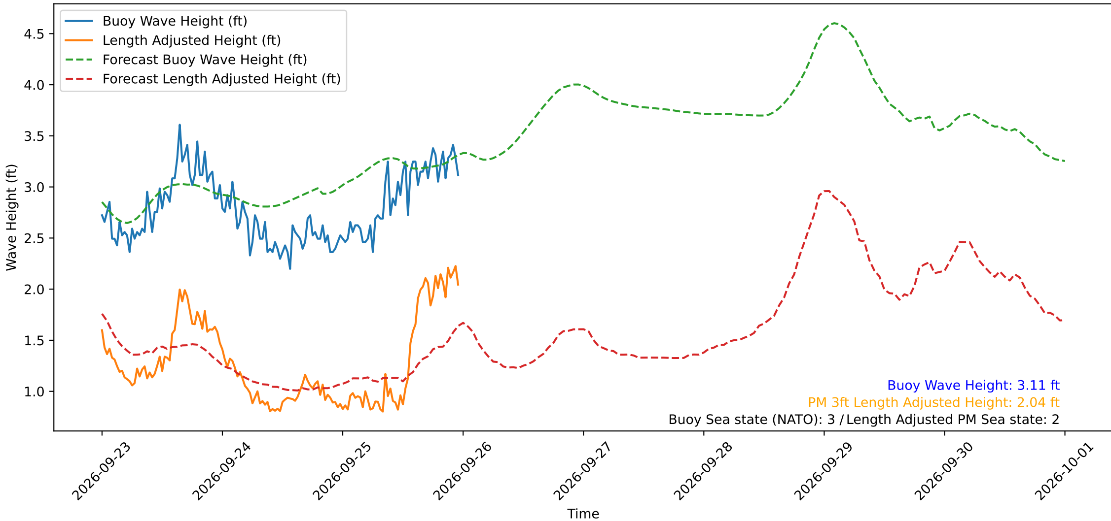
Wave Heights over Time for Oceanside Harbor at 2026-09-25 23:50:29
