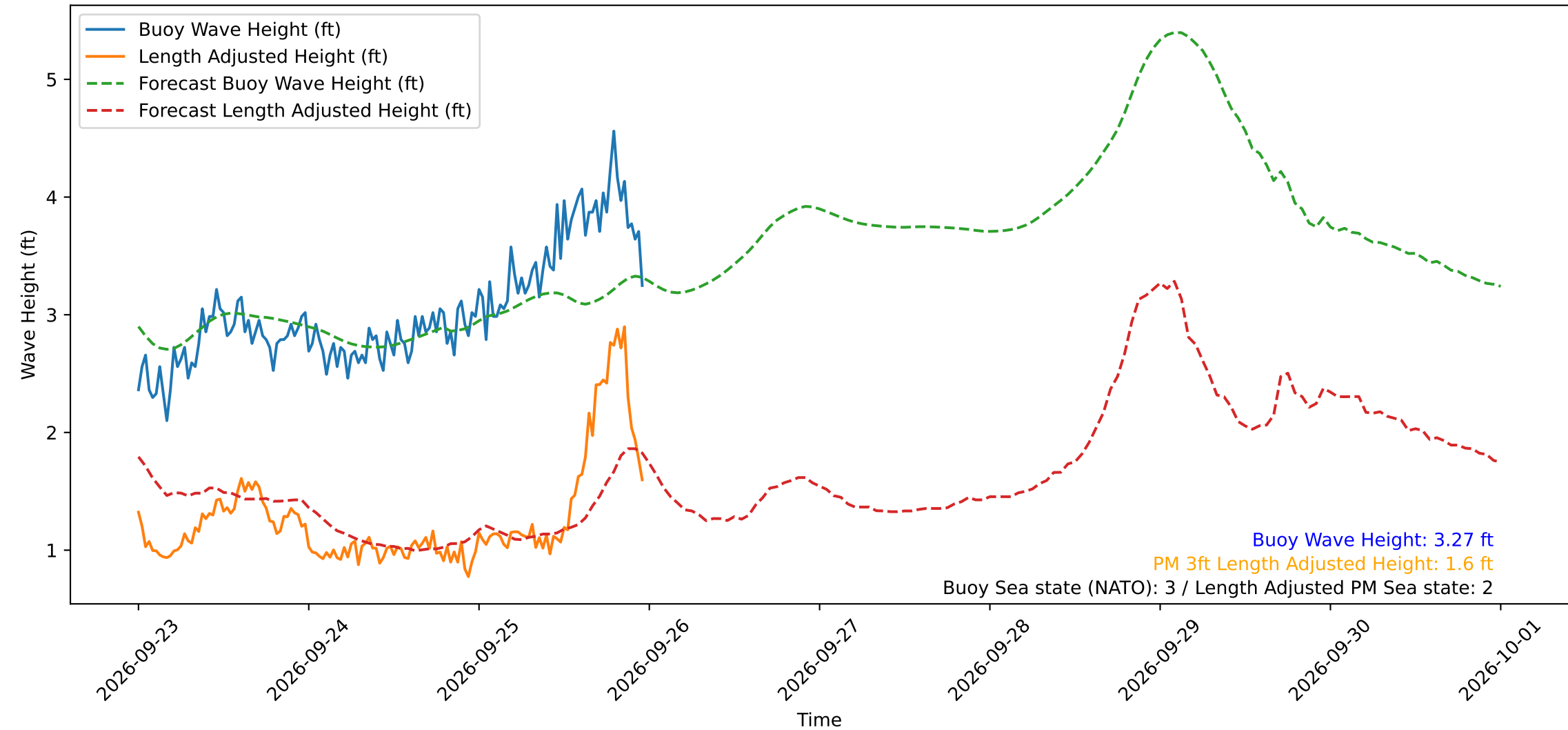
Wave Heights over Time for Green Beach at 2026-09-25 23:51:13
