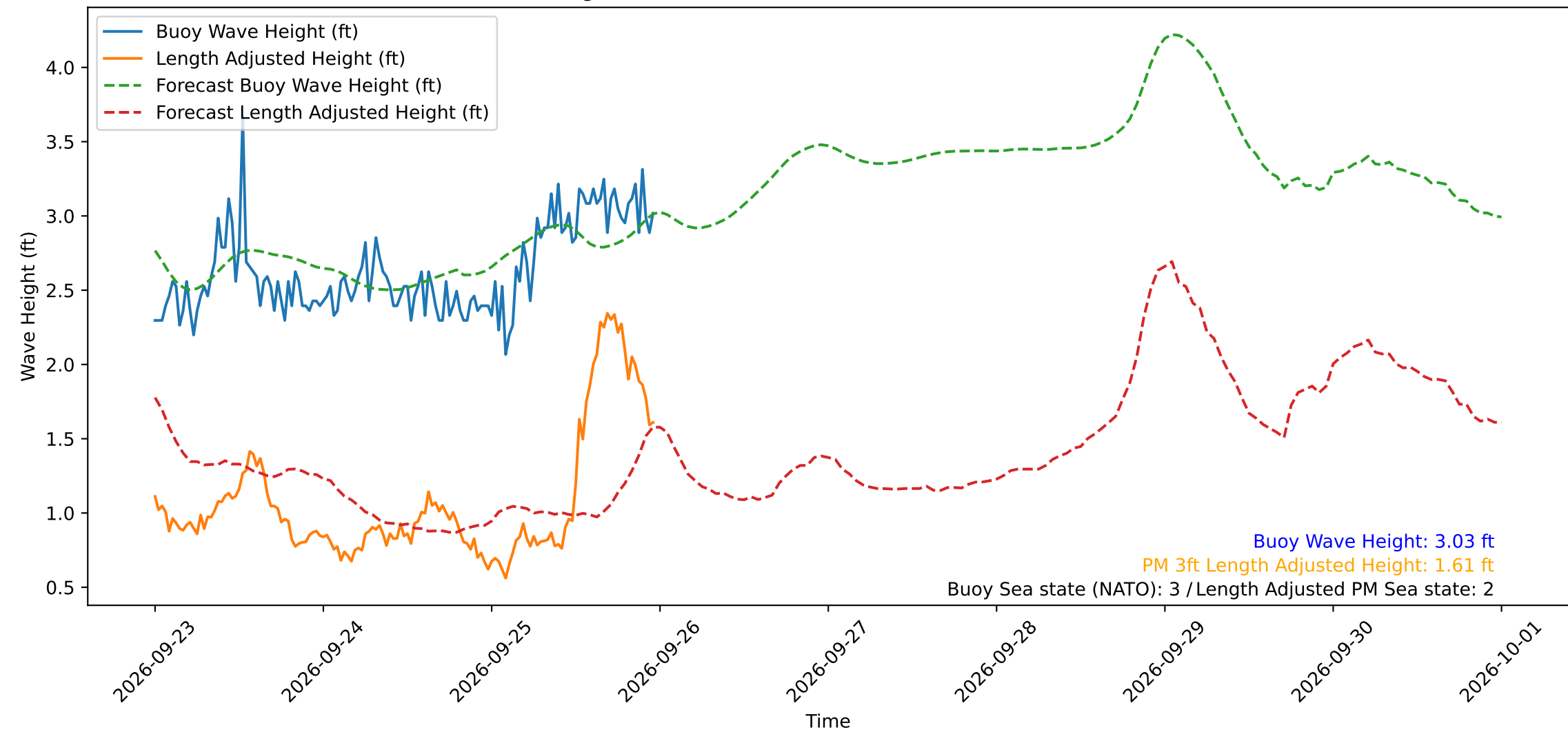
Wave Heights over Time for Red Beach at 2026-09-25 23:50:50
