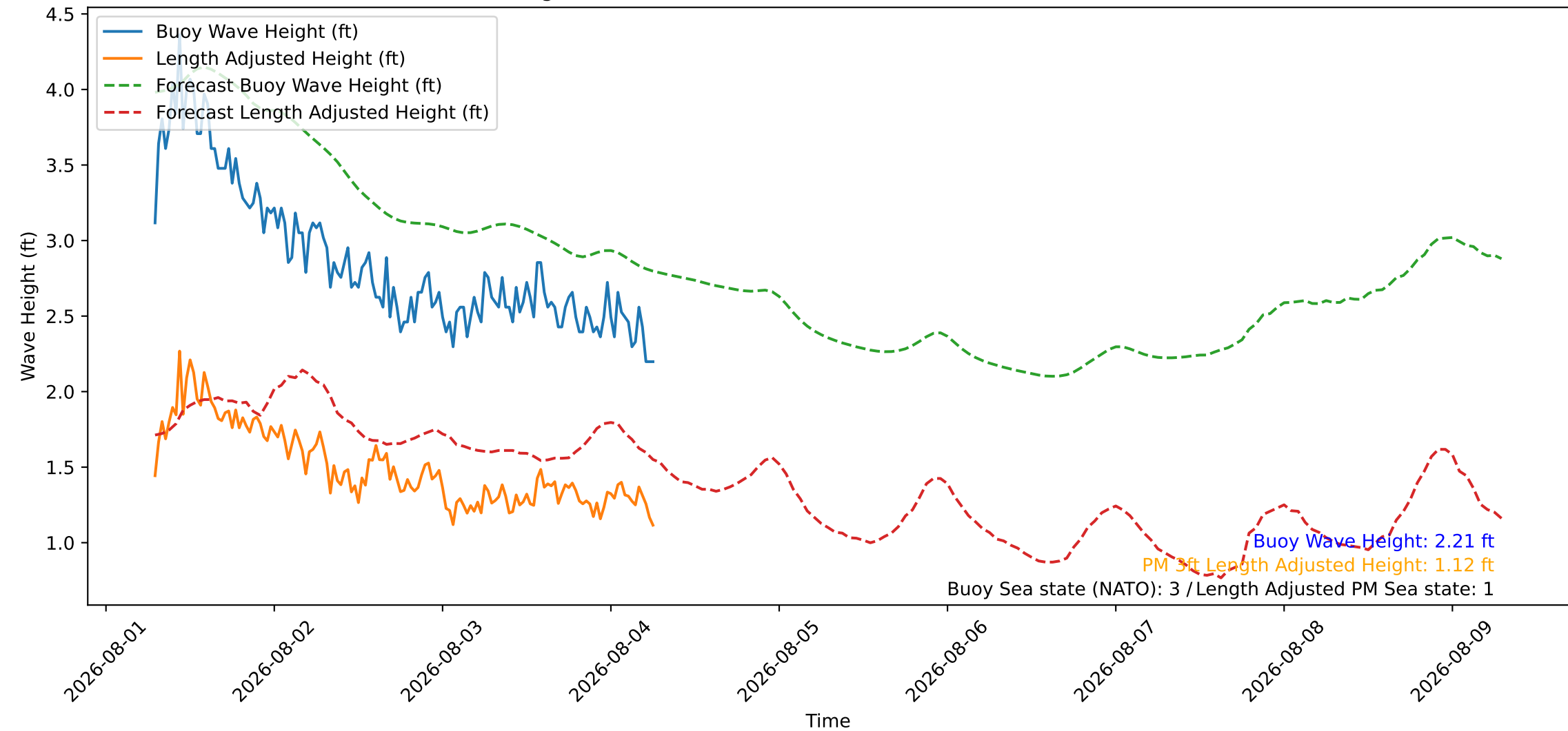
Wave Heights over Time for Oceanside Harbor at 2026-08-04 07:00:26
