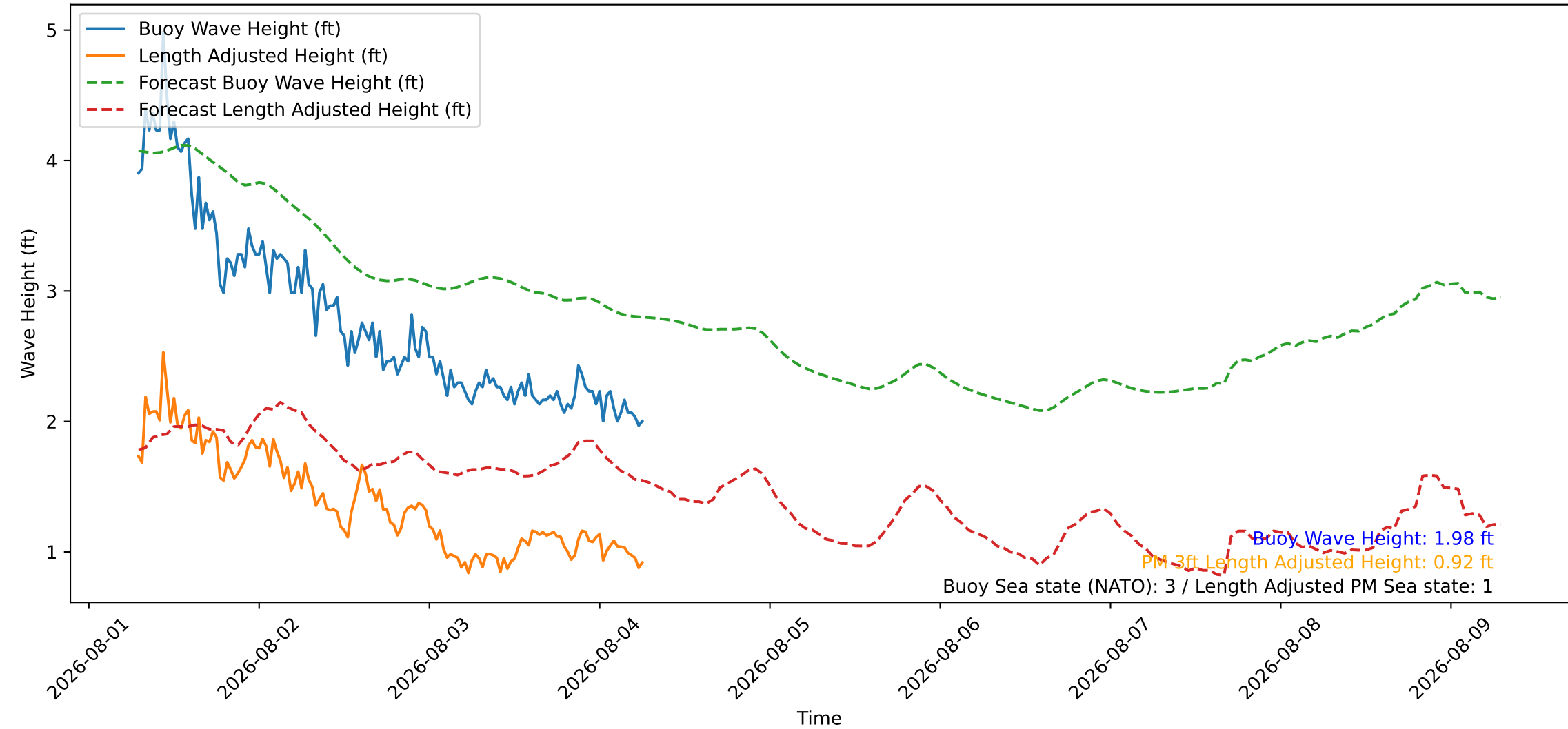
Wave Heights over Time for Green Beach at 2026-08-04 07:01:08
