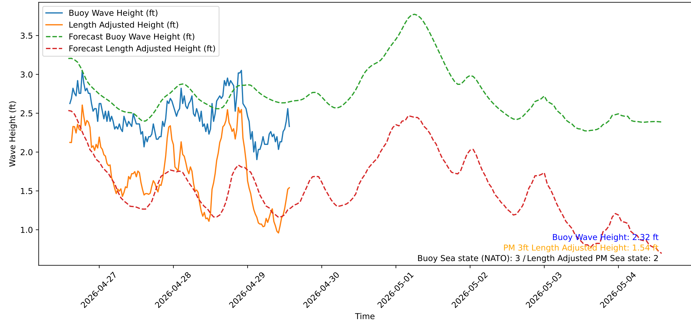
Wave Heights over Time for Oceanside Harbor at 2026-04-29 14:20:31
