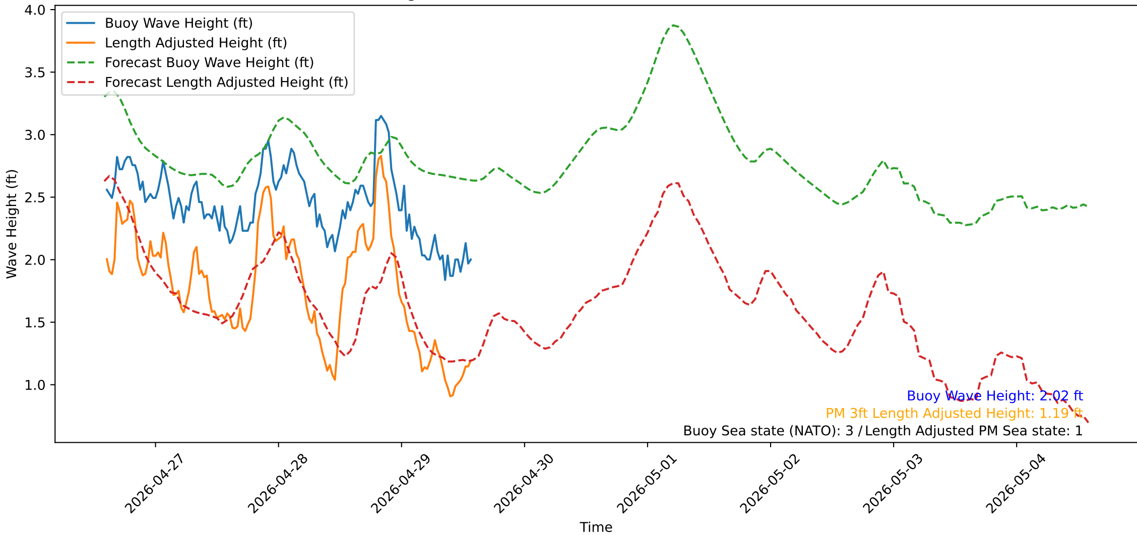
Wave Heights over Time for Green Beach at 2026-04-29 14:21:14
