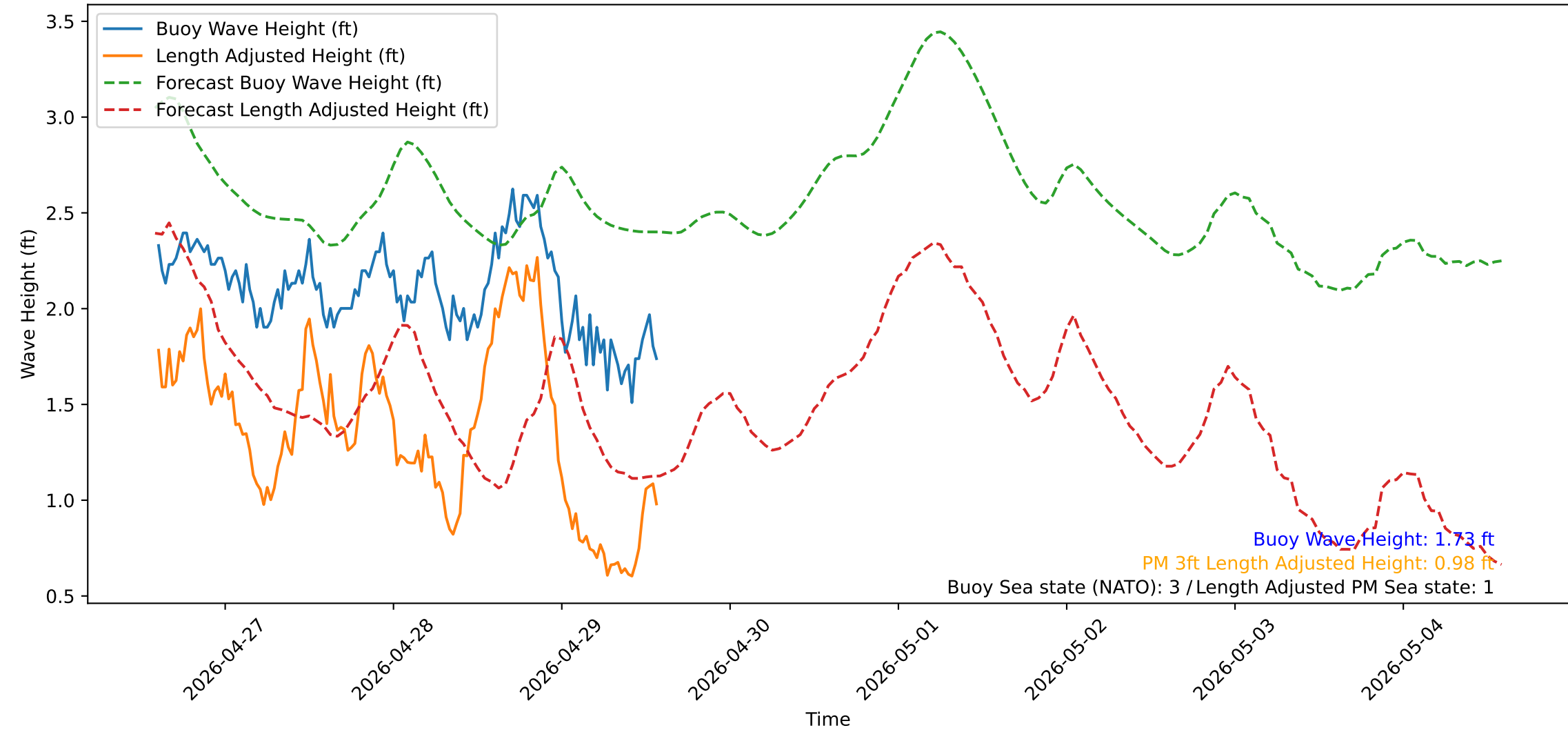
Wave Heights over Time for Red Beach at 2026-04-29 14:20:52
