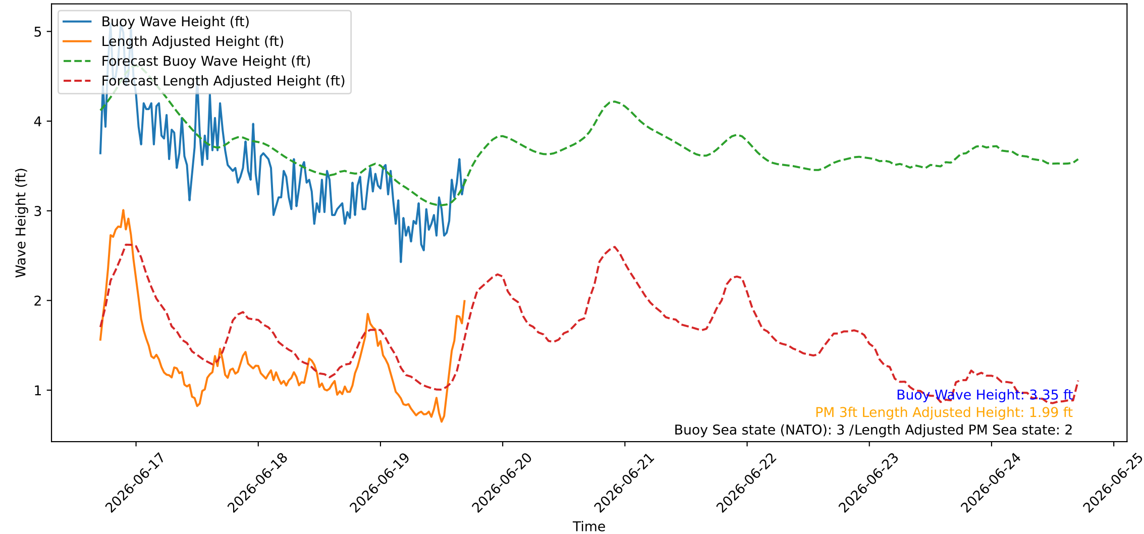
Wave Heights over Time for Green Beach at 2026-06-19 17:11:07
