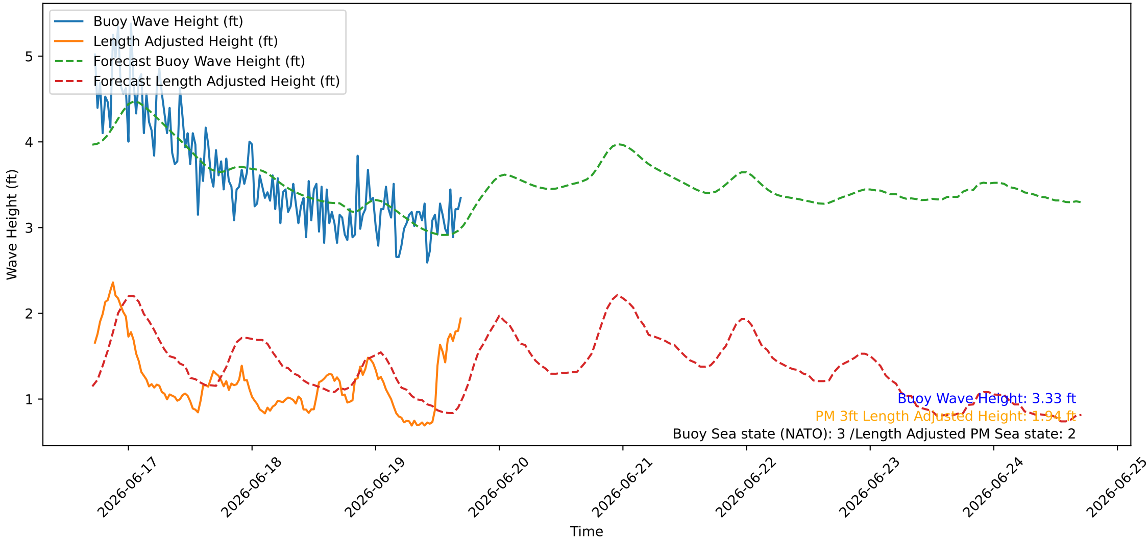
Wave Heights over Time for Red Beach at 2026-06-19 17:10:45
