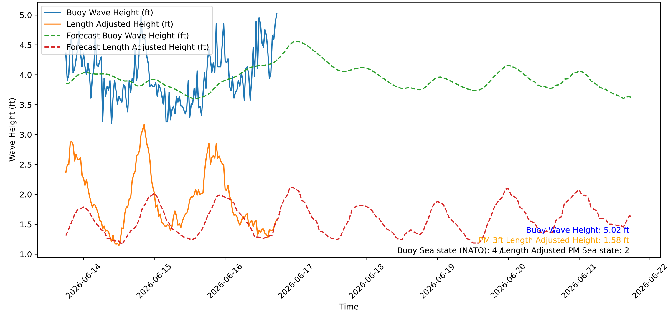
Wave Heights over Time for Oceanside Harbor at 2026-06-16 18:10:26
