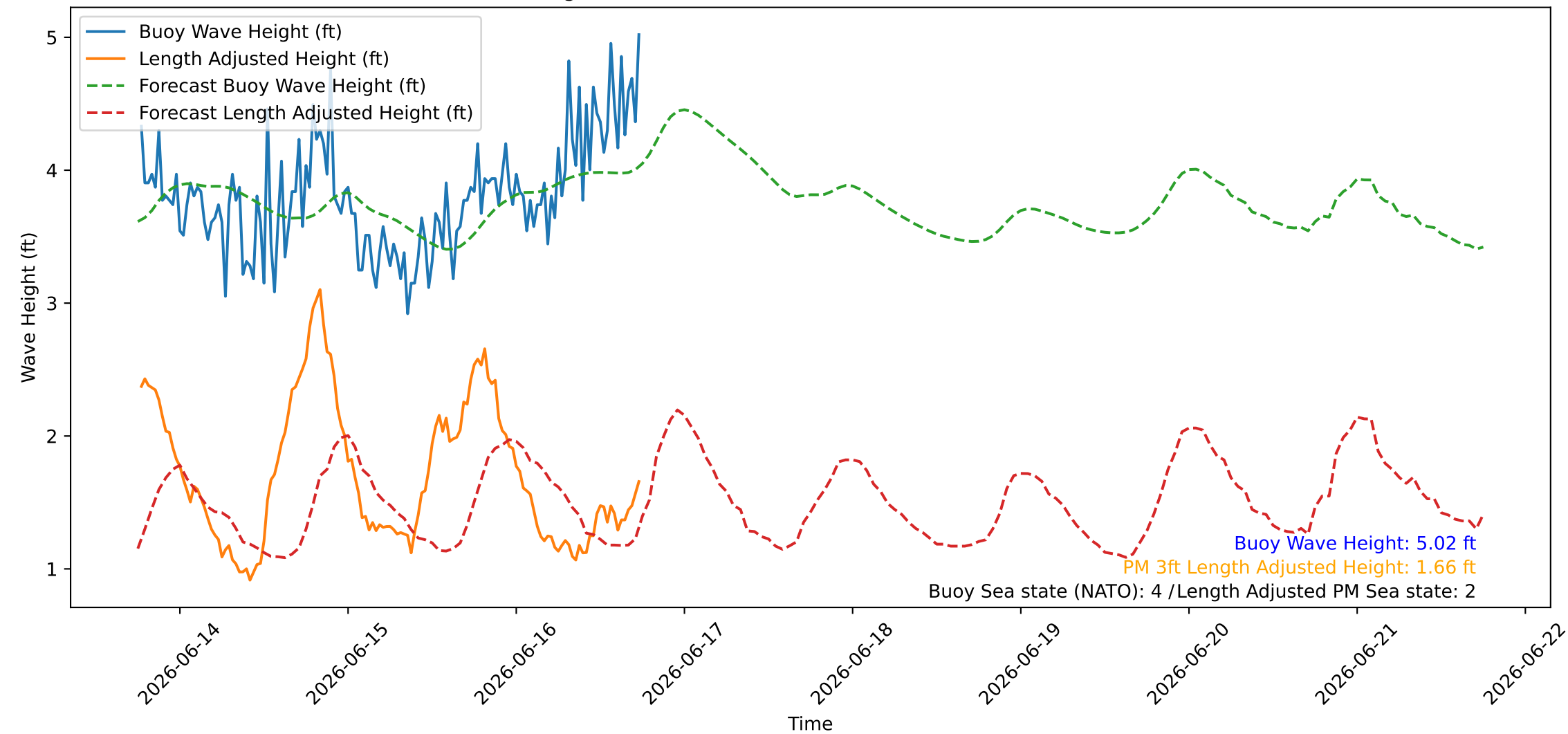
Wave Heights over Time for Red Beach at 2026-06-16 18:10:46
