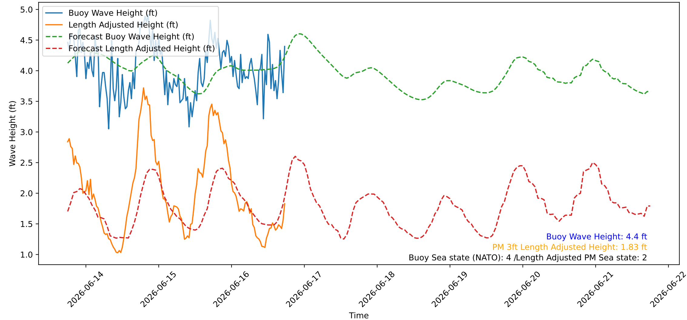
Wave Heights over Time for Green Beach at 2026-06-16 18:11:09
