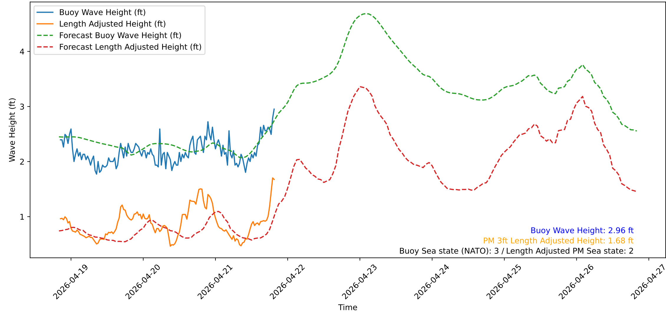
Wave Heights over Time for Red Beach at 2026-04-21 20:20:52
