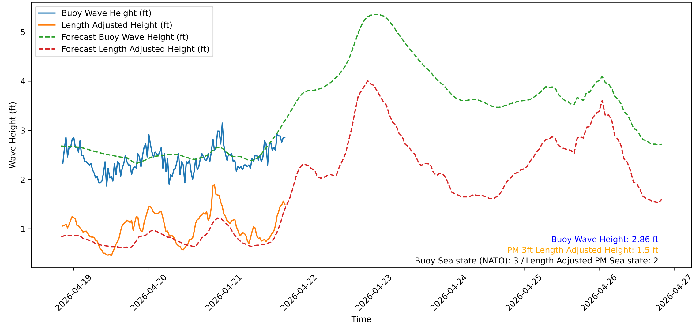
Wave Heights over Time for Green Beach at 2026-04-21 20:21:15
