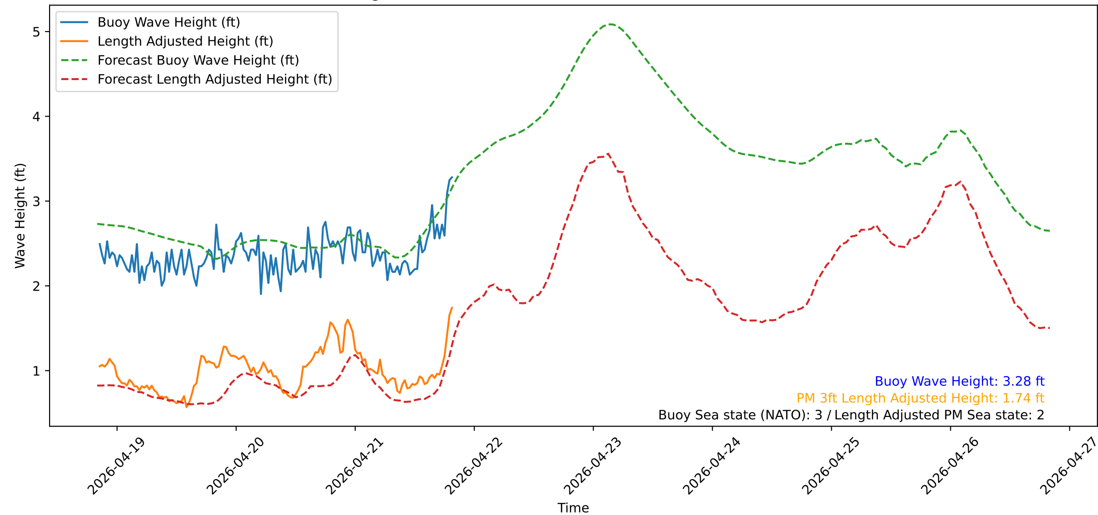
Wave Heights over Time for Oceanside Harbor at 2026-04-21 20:20:32
