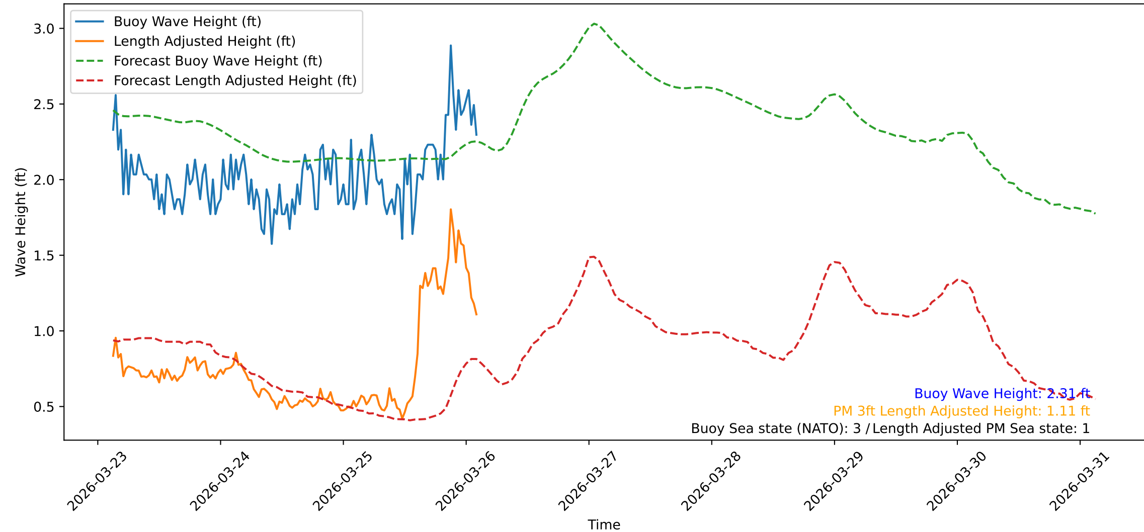
Wave Heights over Time for Oceanside Harbor at 2026-03-26 03:00:31
