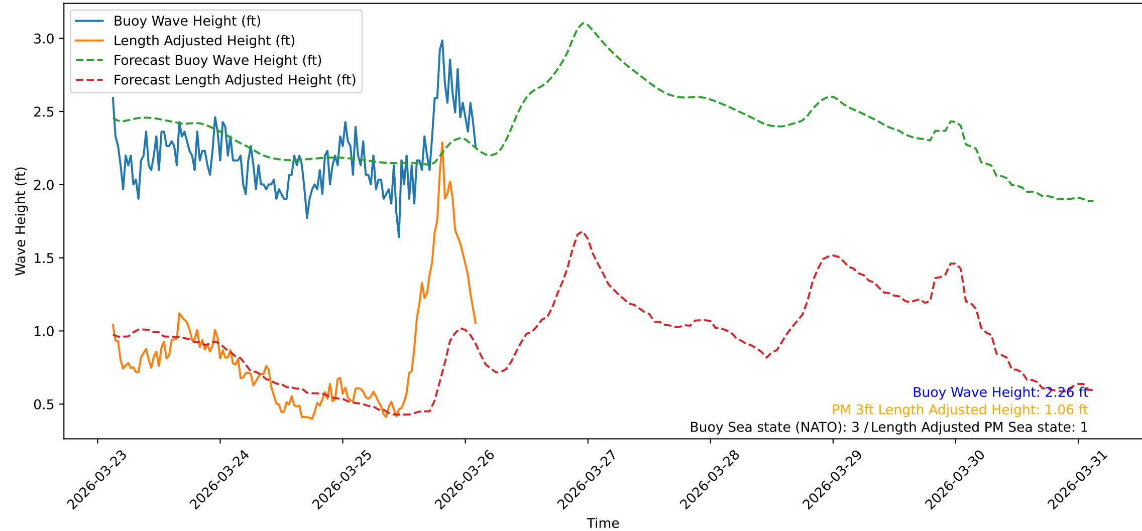
Wave Heights over Time for Green Beach at 2026-03-26 03:01:09
