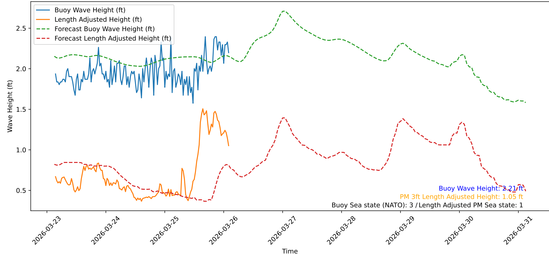
Wave Heights over Time for Red Beach at 2026-03-26 03:00:47
