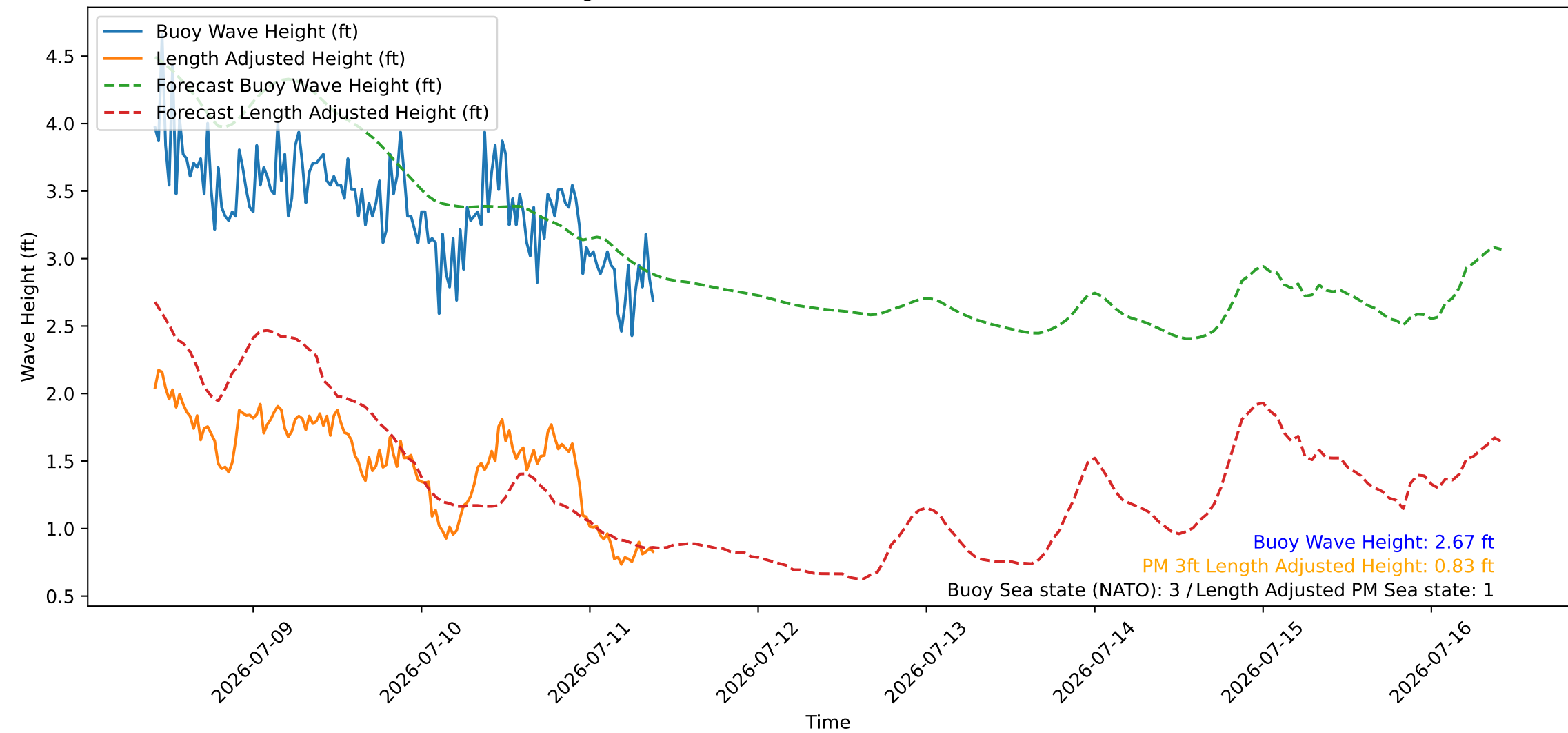
Wave Heights over Time for Red Beach at 2026-07-11 09:40:45
