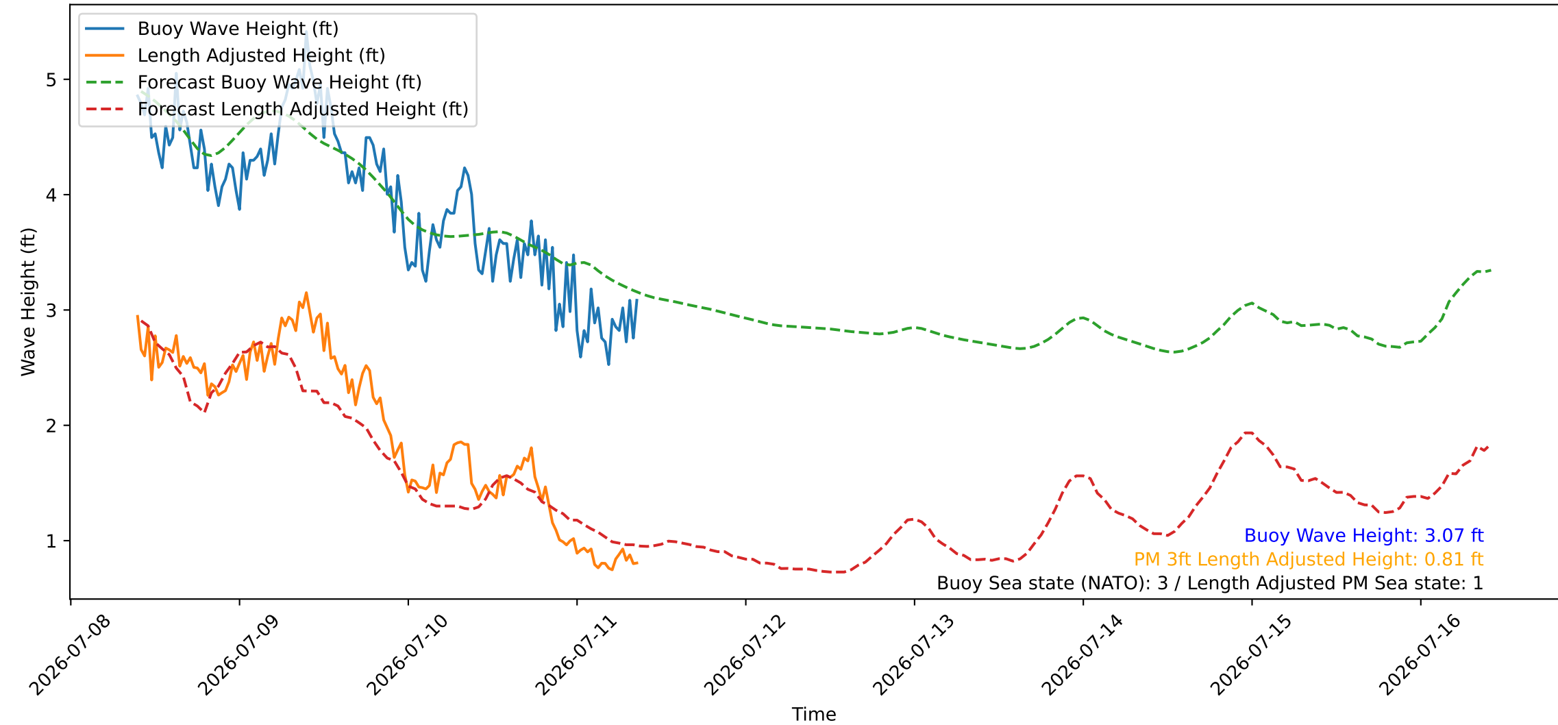
Wave Heights over Time for Oceanside Harbor at 2026-07-11 09:40:26
