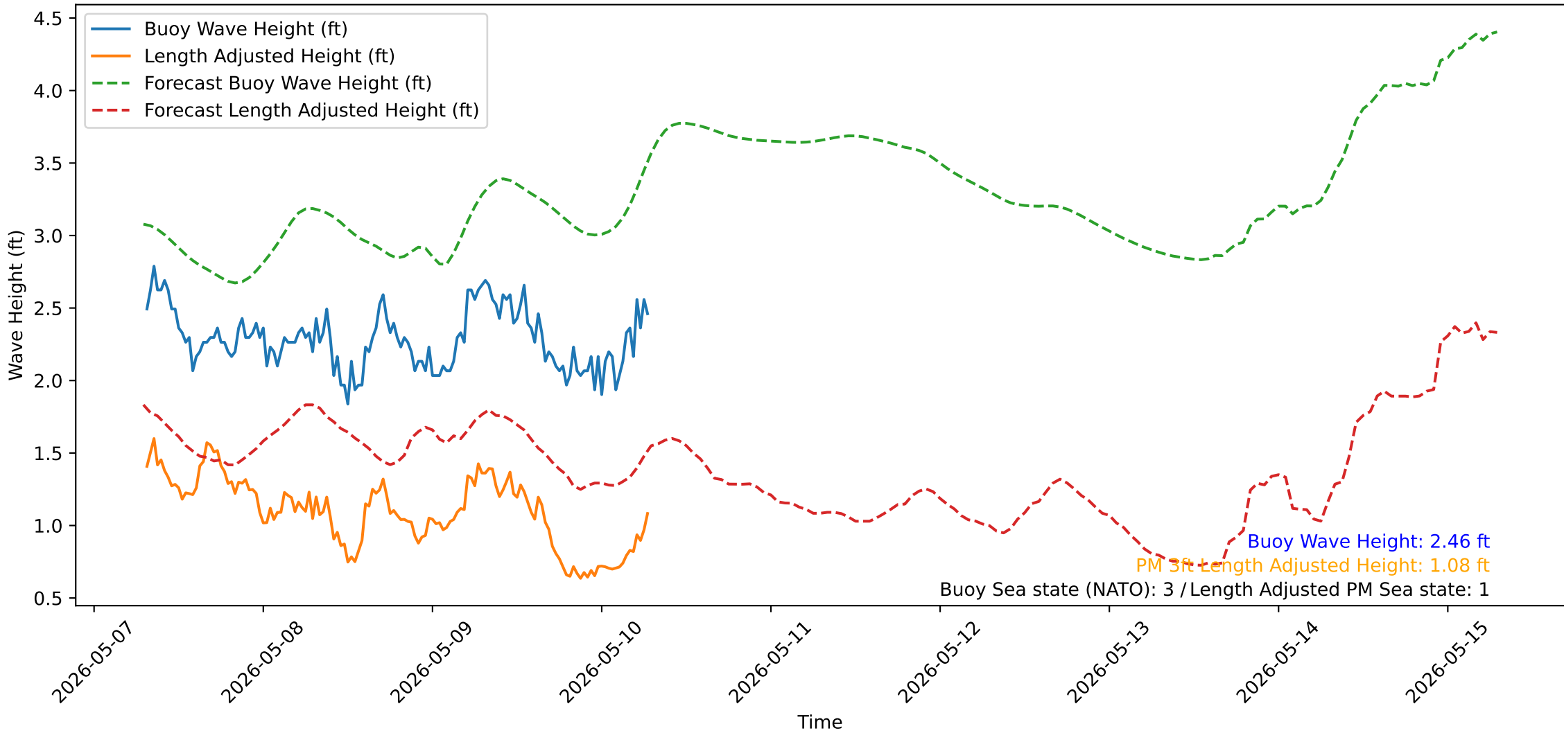
Wave Heights over Time for Green Beach at 2026-05-10 07:21:14
