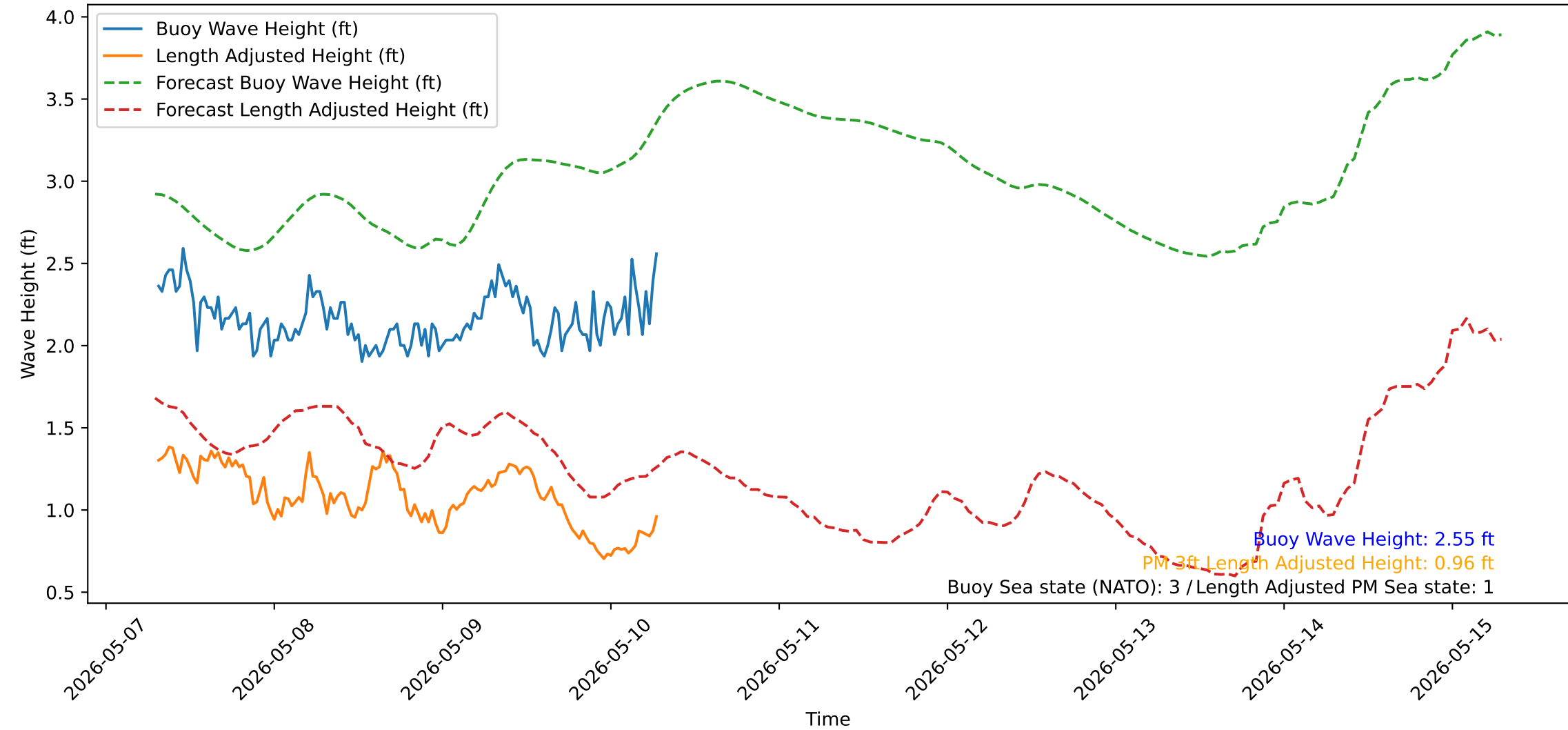
Wave Heights over Time for Red Beach at 2026-05-10 07:20:52
