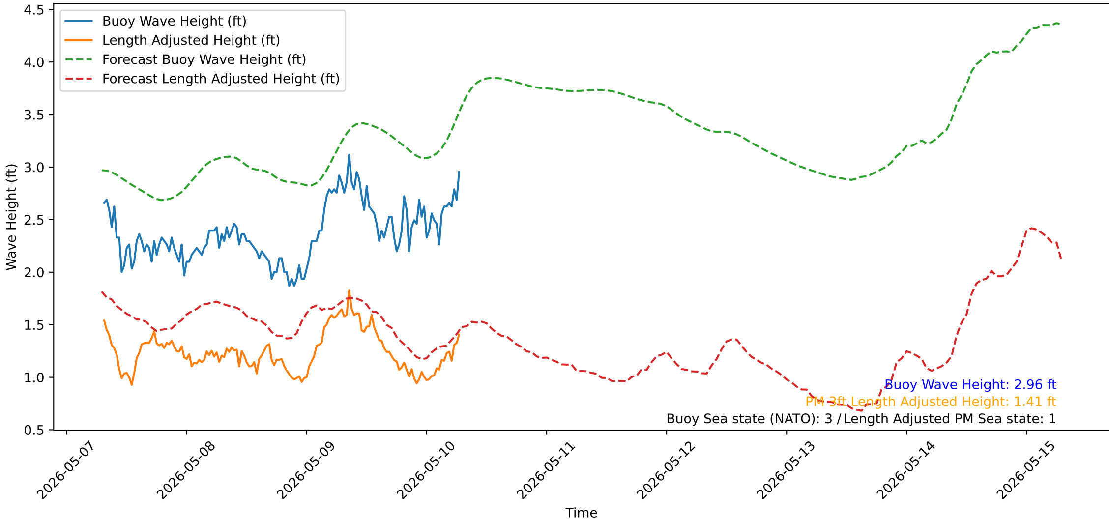
Wave Heights over Time for Oceanside Harbor at 2026-05-10 07:20:31
