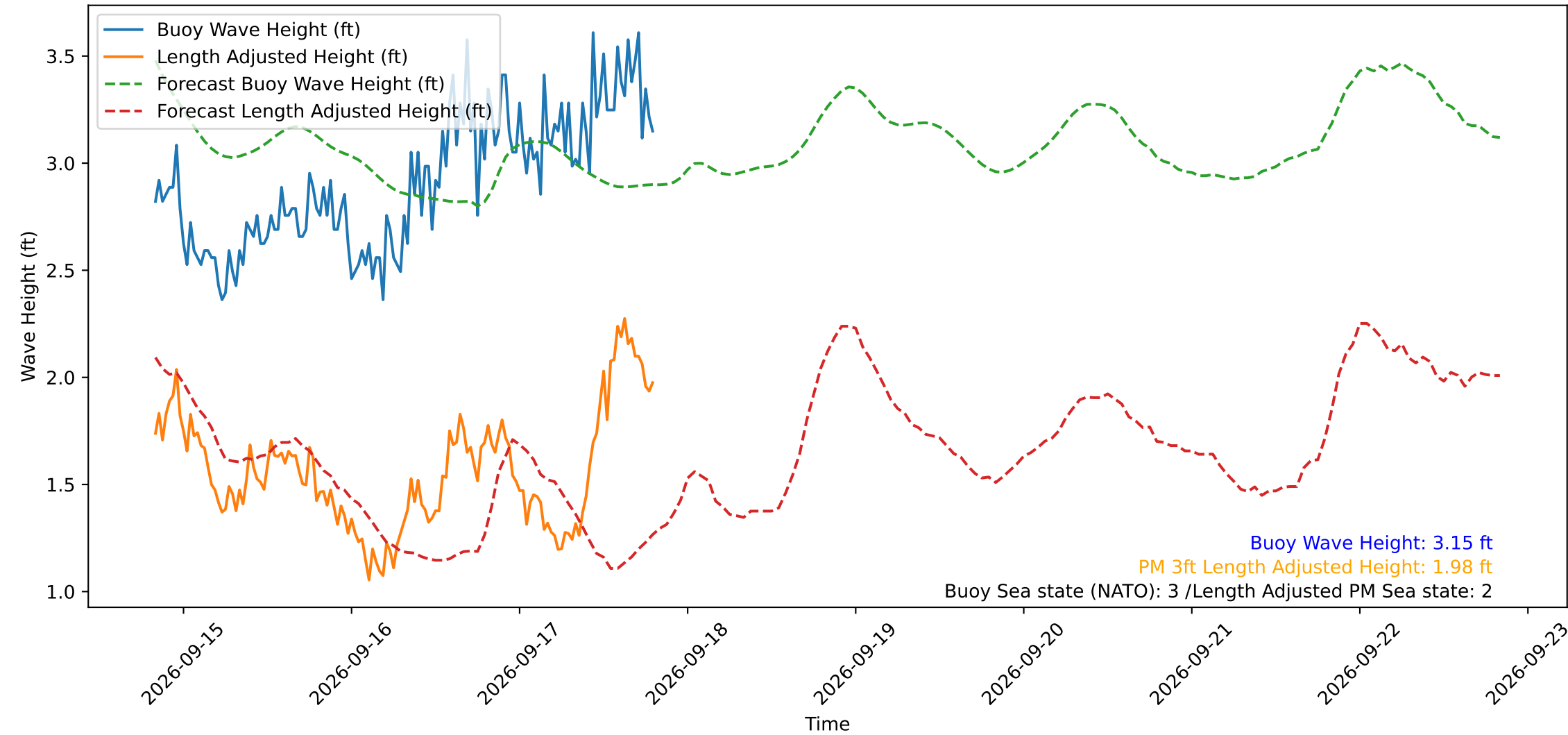
Wave Heights over Time for Oceanside Harbor at 2026-09-17 19:50:29
