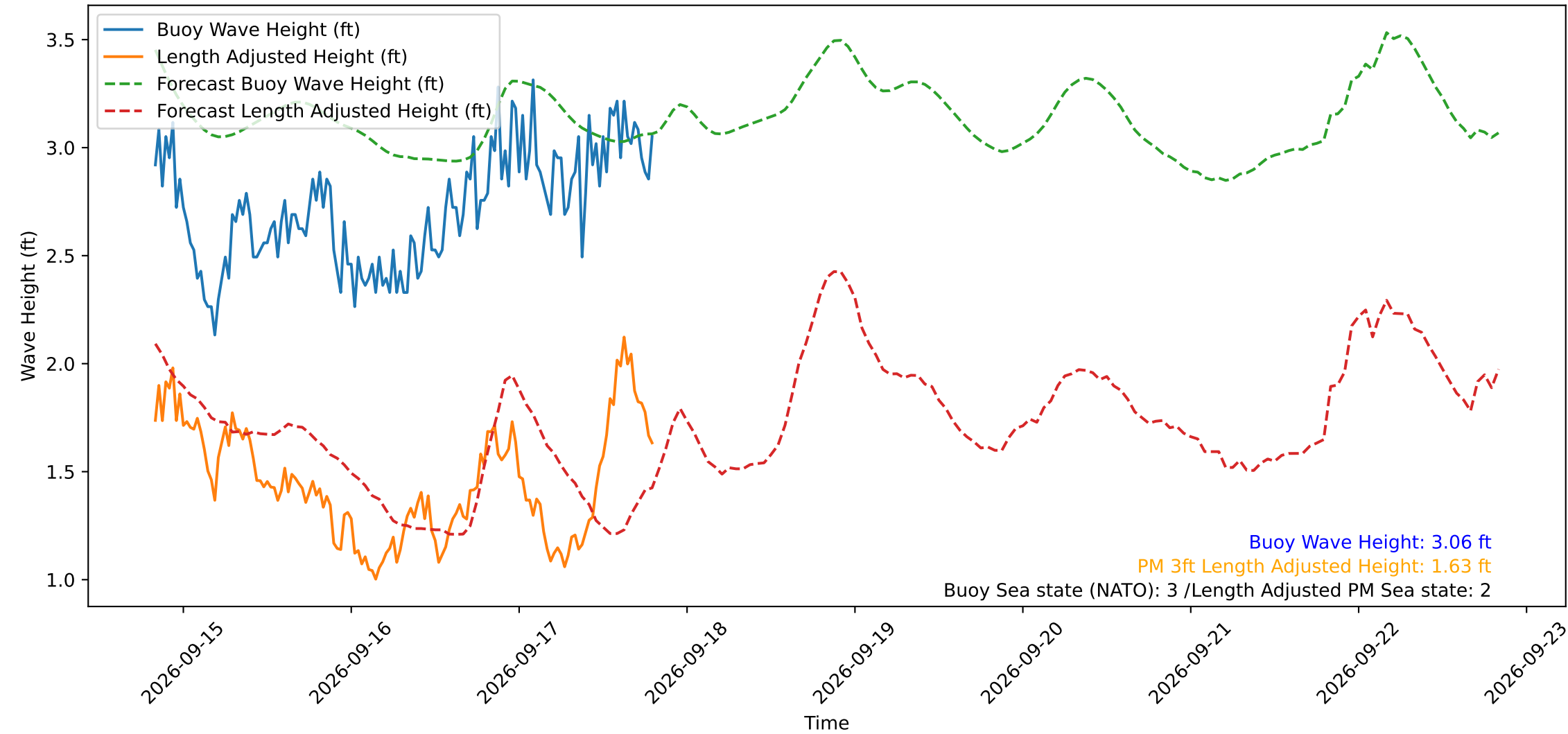
Wave Heights over Time for Green Beach at 2026-09-17 19:51:13
