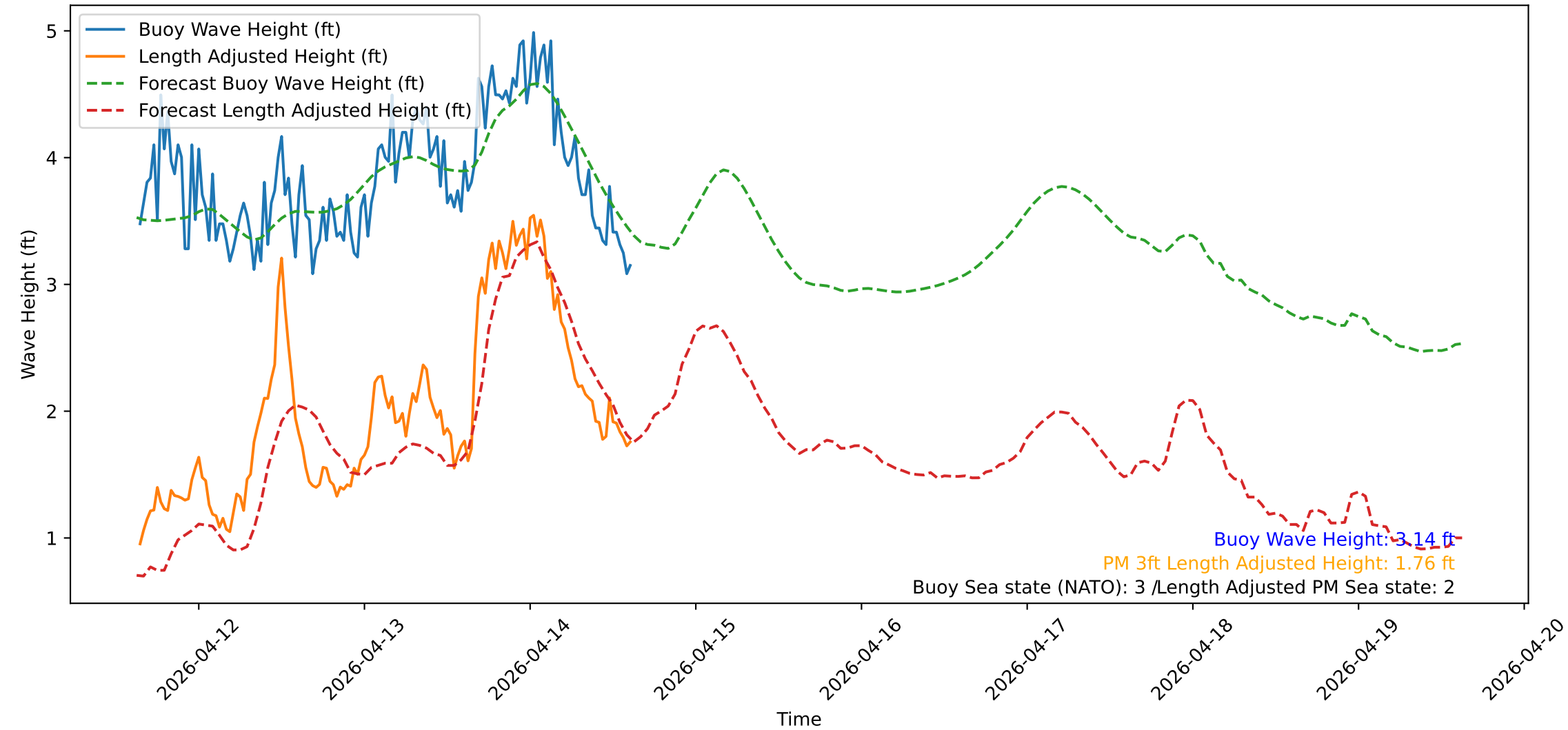
Wave Heights over Time for Green Beach at 2026-04-14 15:21:13
